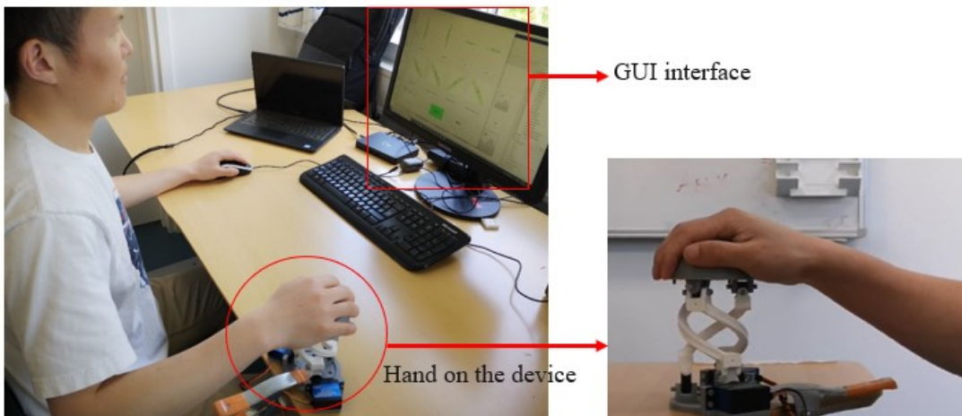
Figure 3.4 – Experiment setup
