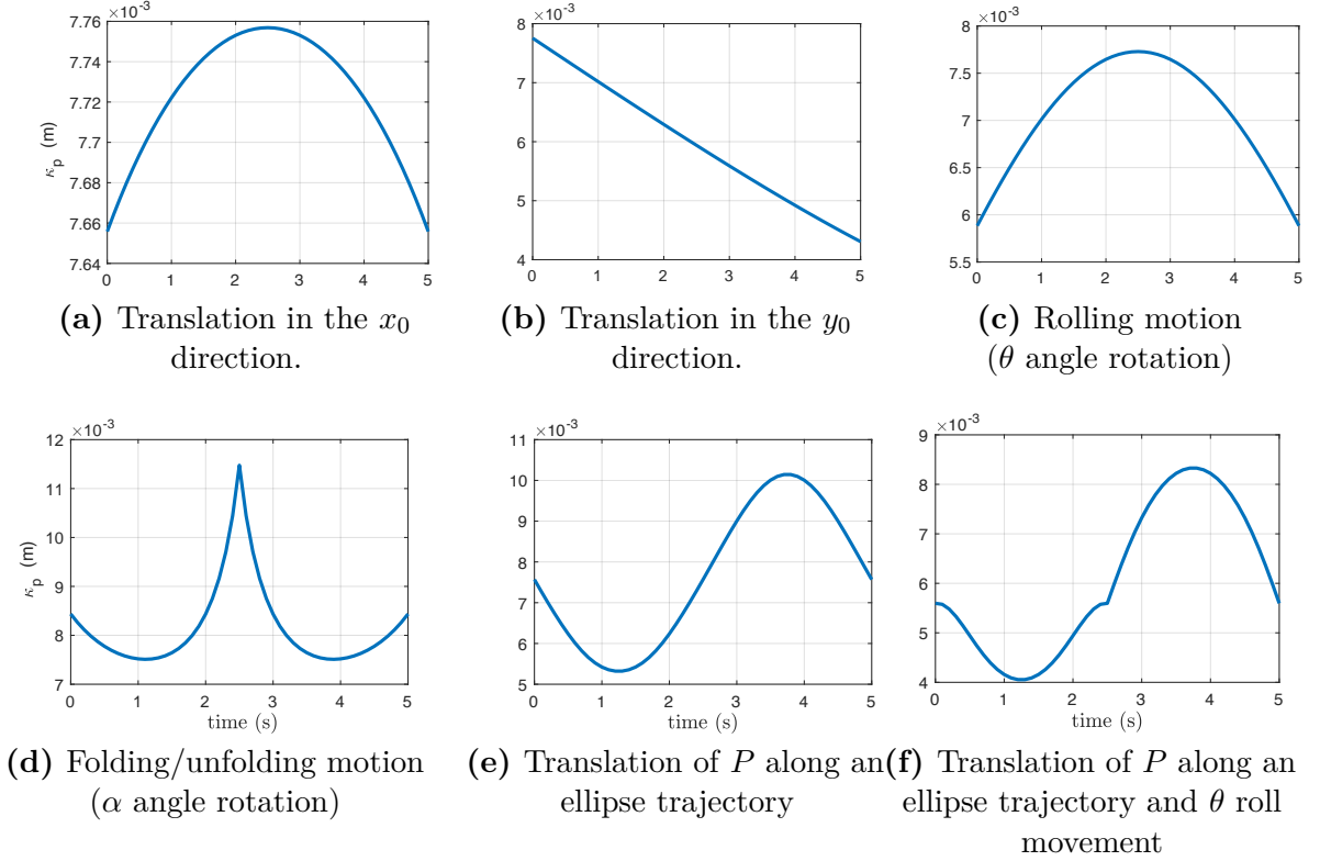
Figure 4.9 – Numerical simulations: Kinematic manipulability index \kappa_p evaluated considering the position Jacobian matrix \mathbf{J}_p .
