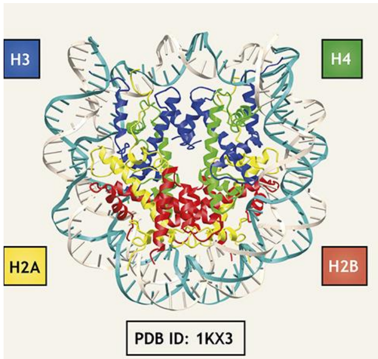
Figure 4. Nucleosome core particle.
