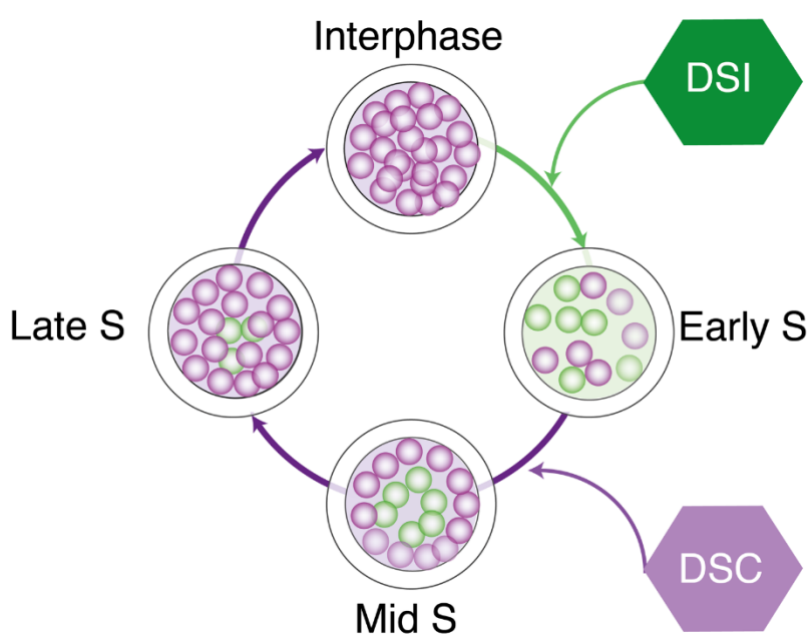
Figure. 25. H3.1/H3.2 enrichment at chromocenter during the cell cycle.
