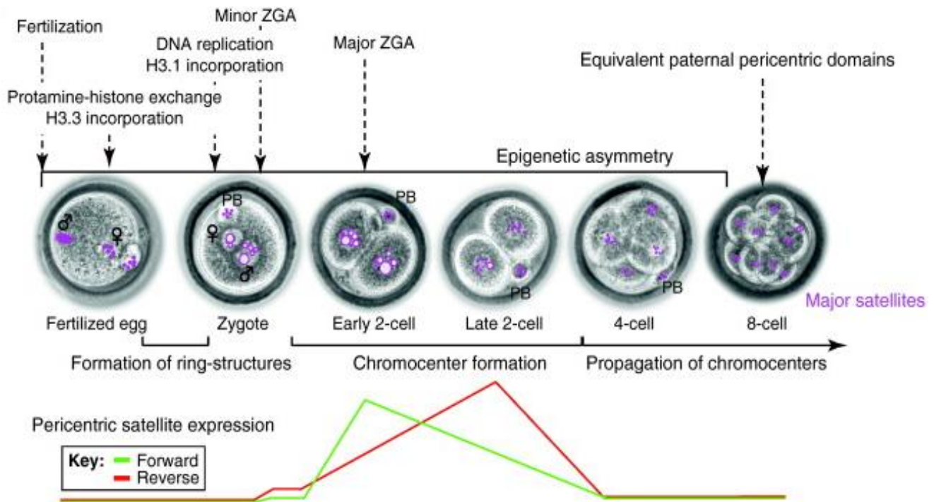
Figure 15. Pericentric satellite reorganization and expression during preimplantation development.
