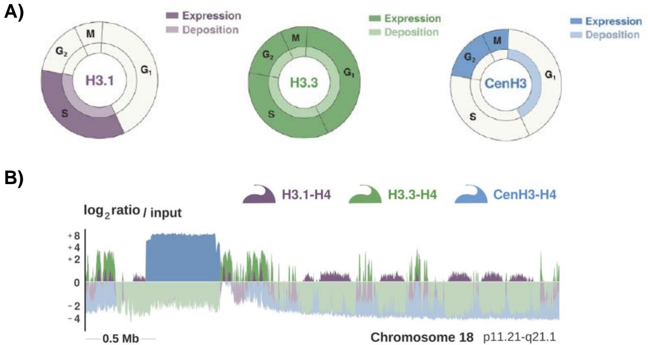
Figure 5. H3 variants are deposited at different timings and locations. A) Schematic representation of H3.1, H3.3 and CenH3 expression and timing of deposition. B) Genomic distribution (ChIP-seq) of H3.1, H3.3, and CenH3 in HeLa cells. The plot shows the enrichment relative to input for all variants at a representative region spanning the centromere and the proximal short and long arms of chromosome 18 (p11.21-q21.1). Adapted from (Mendiratta et al., 2019).
