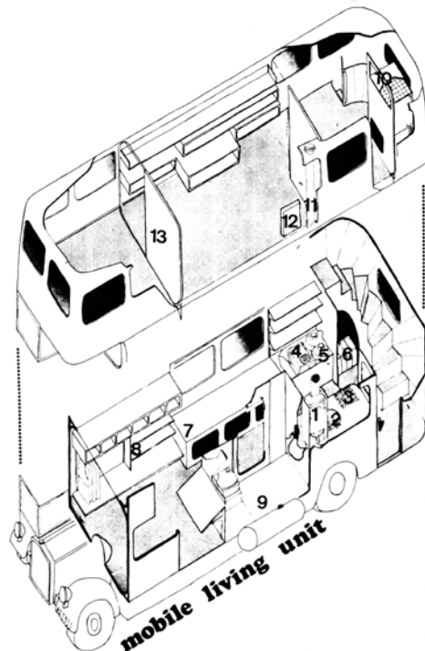
The bus converted by three Newcastle students Andrew Thorne, Angus Brown and Eric Parry. Key. 1. Geysers. 2. Sink. 3. Cooker. 4. Generator. 5. Calor gas. 6. Batteries. 7. Eating Area/Storage beneath. 8. Storage. 9. Shower/w.c. cabinet. 10. Water tank. 11. Geysers flue. 12. Gas panel heater. 13. Flexible partition.
