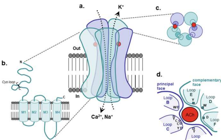
Figure 14. Structure of nAChR.
