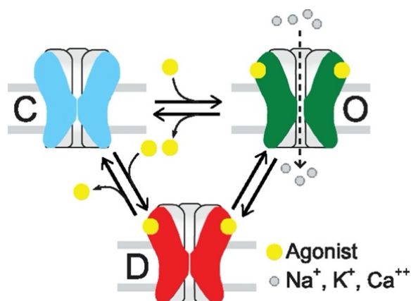
Figure 15. nAChR configuration states. Closed (C), open (O) and desensitized (D) 136 .
