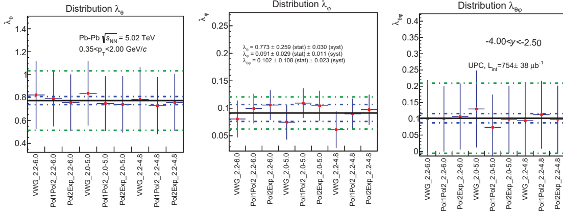
FIGURE 5.10. Polarisation parameters ( \lambda_\theta , \lambda_\phi , \lambda_{\theta\phi} ) obtained by introducing full transverse polarisation in the MC. The black solid line indicates the average values. Dotted blue lines indicate the attributed systematic uncertainties calculated using the differences with respect to the nominal values of polarisation parameters. The dotted green lines show the average statistical uncertainties.
