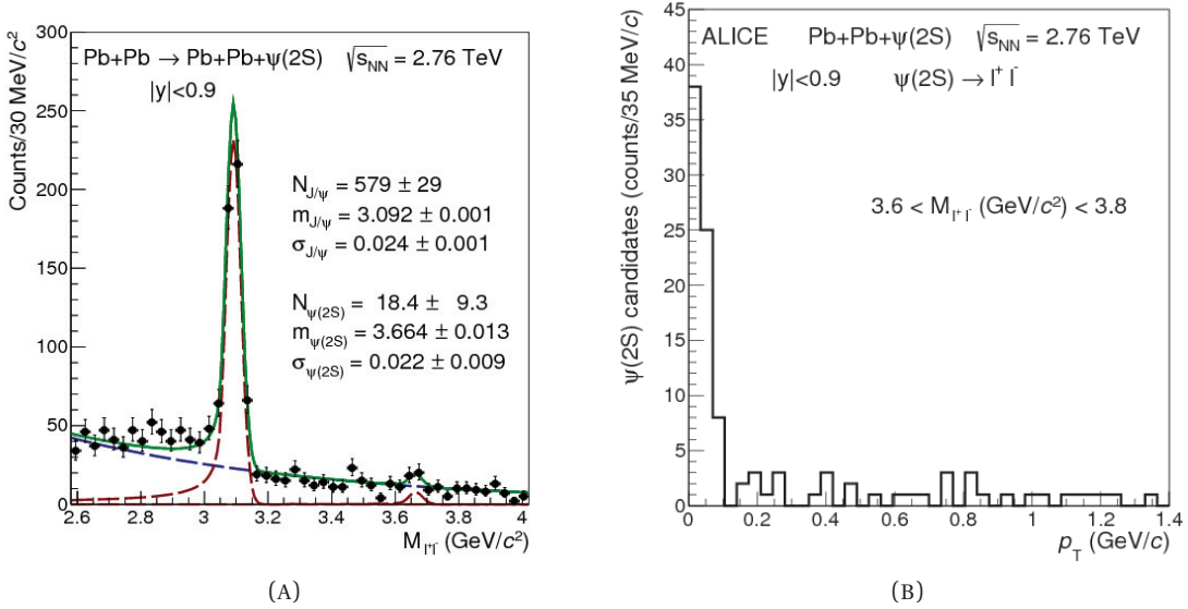
FIGURE 2.22. Invariant mass (left) and p_T distributions (right) of \psi' for ultra-peripheral Pb–Pb collisions at \sqrt{s_{\text{NN}}} = 2.76 \text{ TeV} and 0.9 < y < 0.9 for events satisfying the event selection. The channels \psi' \rightarrow l^+ l^- , are shown ( l^+ l^- = e^+ e^- and \mu^+ \mu^- ), from [103].
