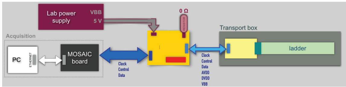
FIGURE 7.1. Overview of the hardware of test bench for ladders qualification without back-bias.
