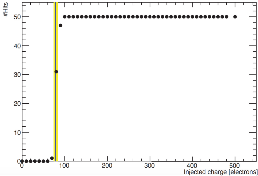
FIGURE 7.7. (Solid black circles) The number of hits digitized as a function of the injected charge for a single pixel (located at row 0, column 0) on chip 7 of ladder 3032. The parameters of the fitted S-curve are also represented, the threshold q_{thr} as a vertical blue line and the temporal noise \sigma as a yellow vertical band.
