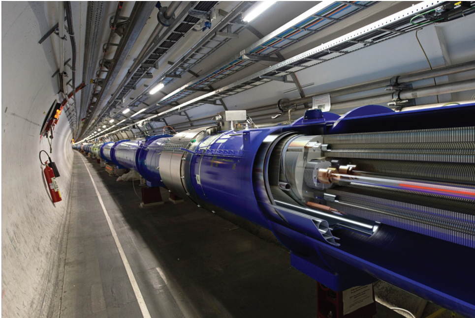
FIGURE 3.1. 3D cut of the LHC dipole, from [107].
