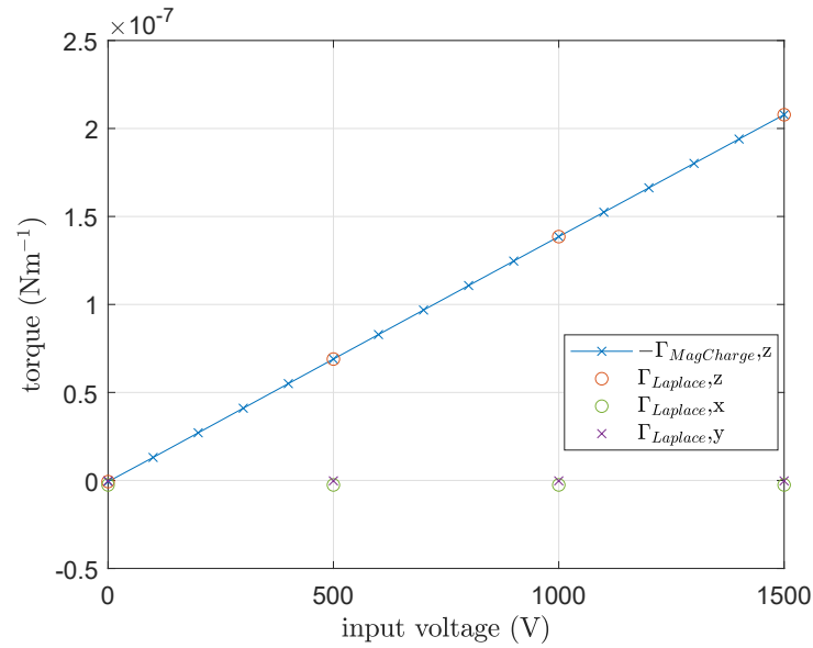
Figure 4.41: Global torque between the Galfenol disk and the magnet vs the voltage applied to the piezoelectric layer. It is computed as a Laplace force in the magnet, and, its (z) component is compared to the torque computed by the magnetic charge method in the Galfenol layer
