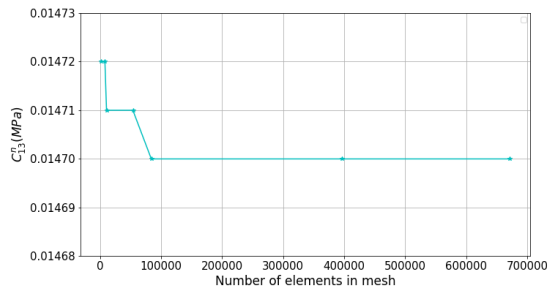
(c) C_{13}^n
