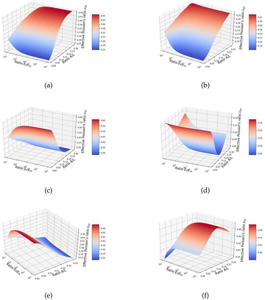
Figure 2.20: Effective Poisson's ratios (a) v_{xy} , (b) v_{yx} , (c) v_{xz} , (d) v_{zx} , (e) v_{yz} , and (f) v_{zy} as a function of fibre crimp level and elastic modulus ratio. The values settings for each parameter are E_m = 10KPa , \nu_f = 0.3 , \nu_m = 0.4 , V_f = 20\% , and \theta = 30^\circ .
