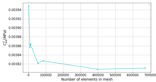
(e) C_{44}^n
