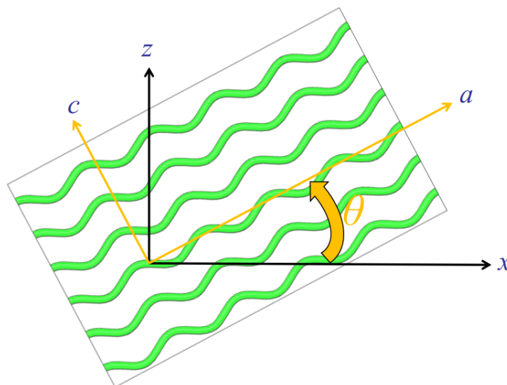
Figure 2.11: Single layer composite orientation in the given coordinate systems.
