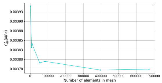
(f) C_{66}^n
