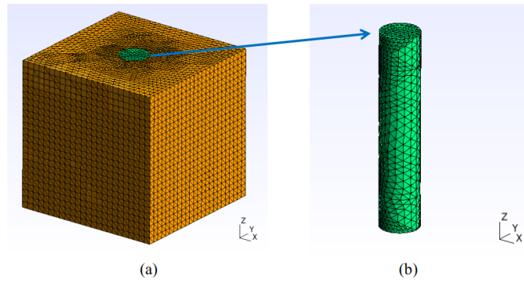
Figure 3.7: Finite element mesh of the REV under consideration here. The number of elements here is 83904. (a) Global view of the REV mesh. (b) Mesh of the fibre embedded in the REV.
