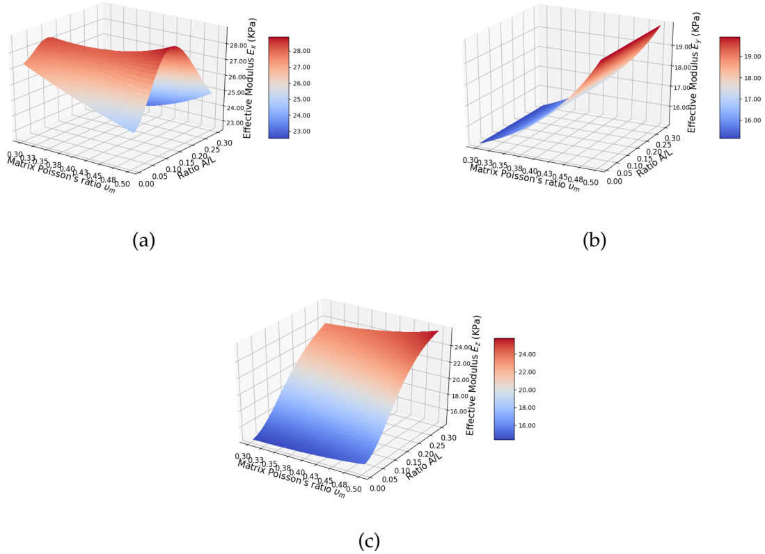
Figure 2.17: Effective axial elastic modulus under load applied along (a) the x-axis, (b) the y-axis, and (c) the z-axis as a function of fibre crimp level and matrix Poisson's ratio. The value settings for each parameter are E_f = 100\text{MPa} , E_m = 10\text{KPa} , \nu_f = 0.3 , V_f = 20\% , and \theta = 30^\circ .
