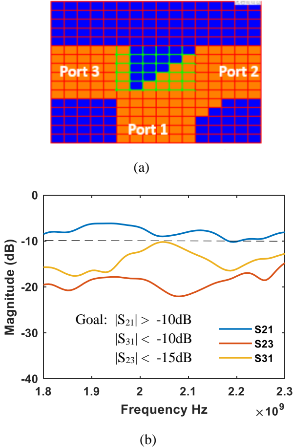
Fig. 3.11. Unequal power distribution from port 1 to ports 2 and 3 (a) Optimized configuration and (b) measured S-parameters.
