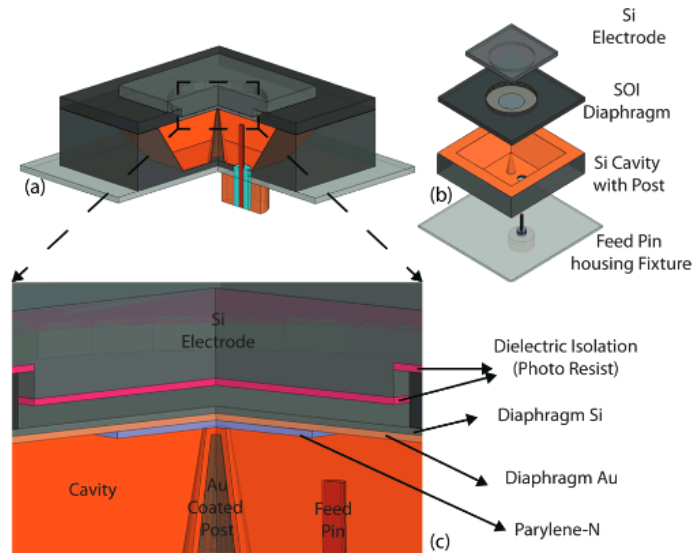
Fig. 1.5. (a) Tunable capacitive-post loaded resonant cavity and (b) parts of assembled resonator [15].
