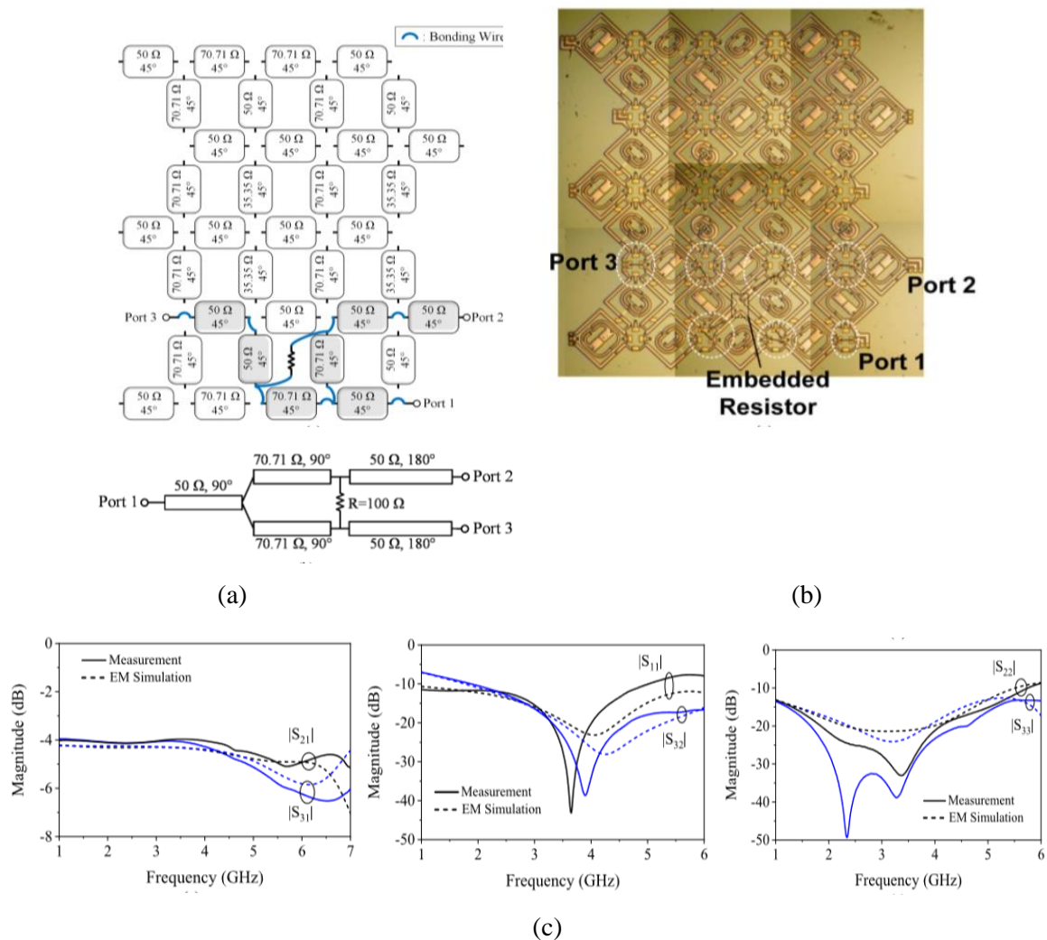
Fig.1.36. (a) Wire-bonding configuration for a power divider at 4 GHz and the corresponding equivalent transmission-line model at 2f_0=4 GHz. (b) Fabricated Chip and (c) Measured and EM simulated results [51].
