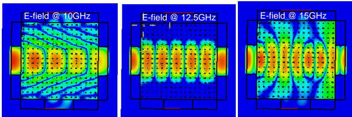
Fig. 4.7. E-field distribution of straight waveguide
