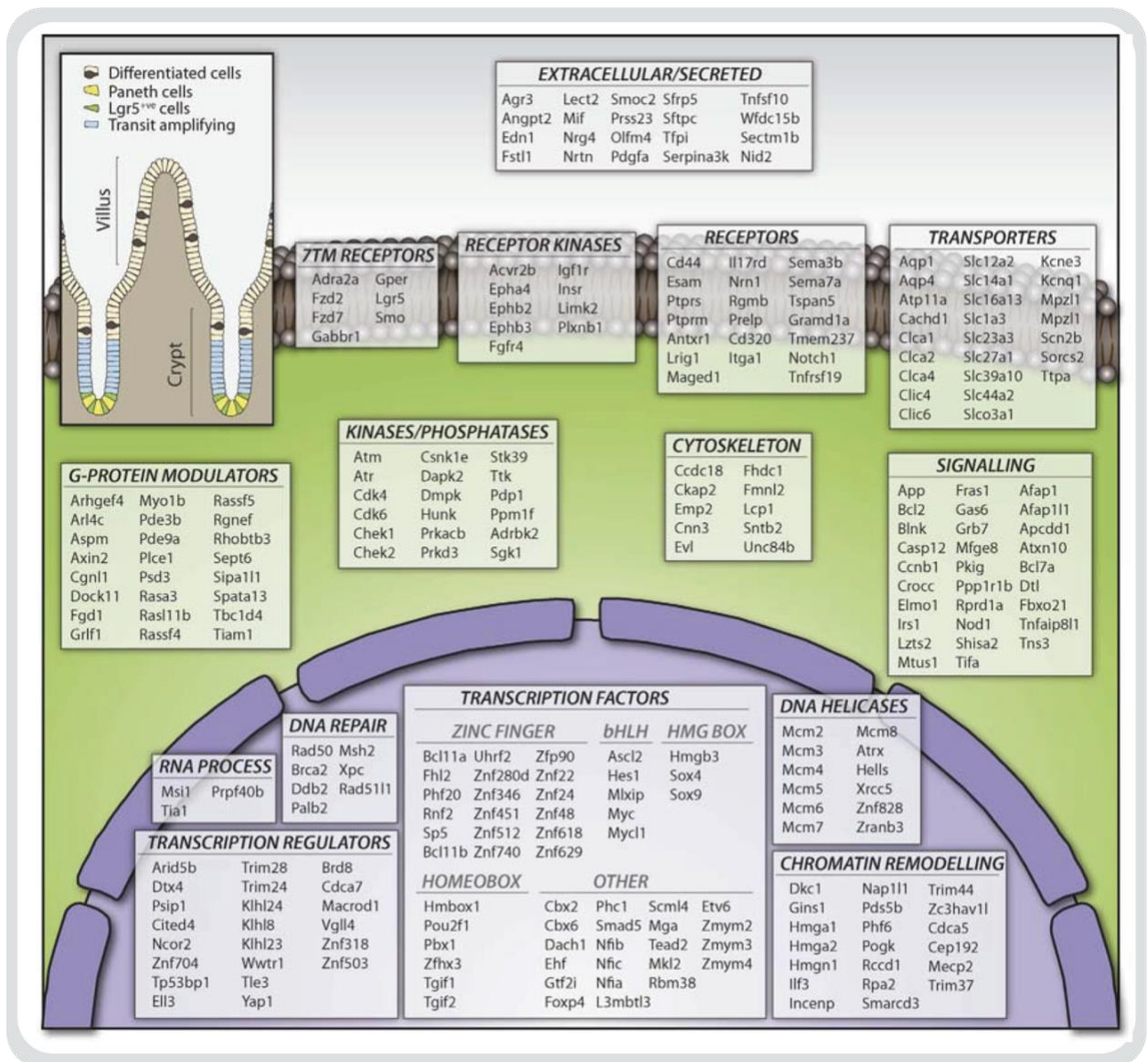
Figure 39. Genes of the Intestinal Stem-Cell Signature and Classification by their Molecular Function
