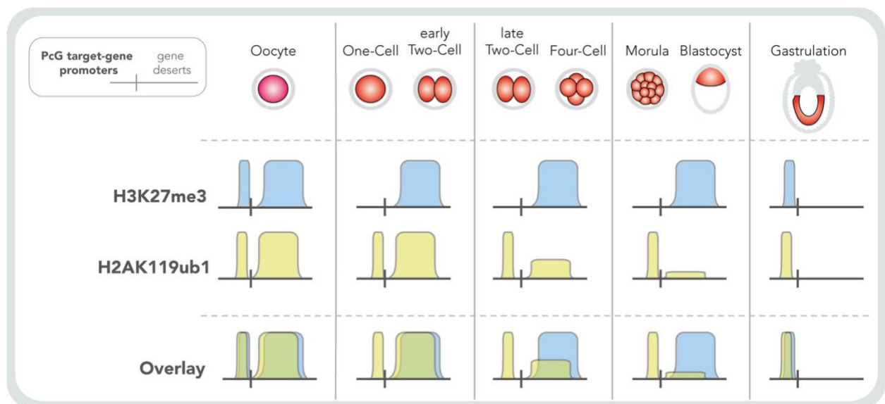
Figure 21. Early Mouse Embryo Histone Modifications and Polycomb
