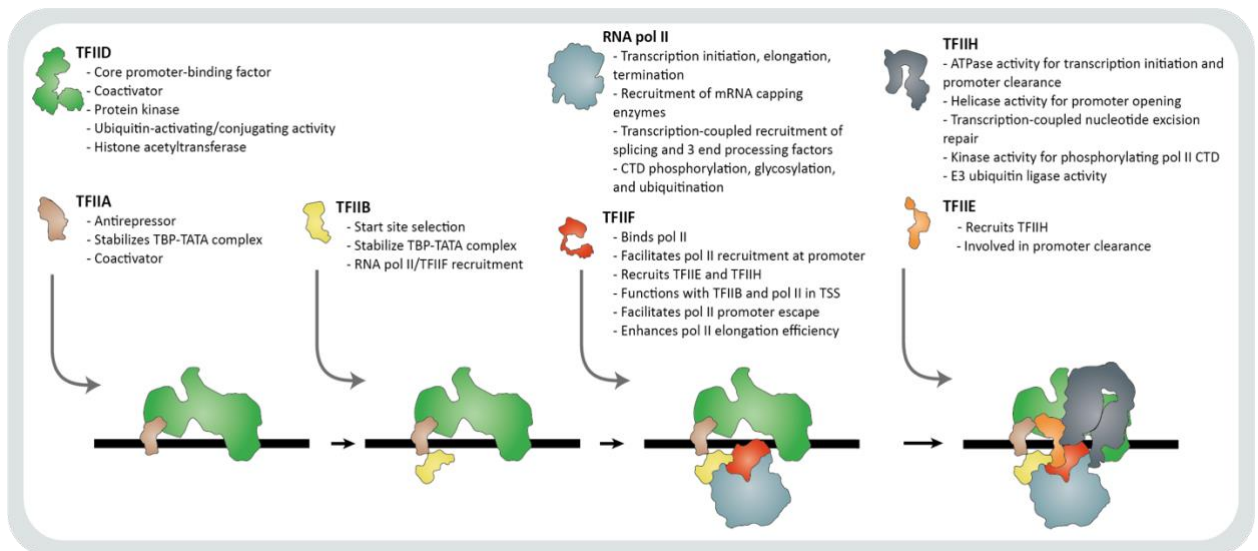
Figure 2. Assembly of the Pre-Initiation Complex (PIC) on Core Promoter
