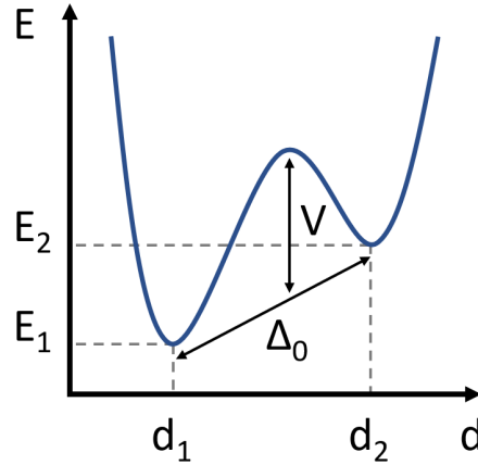
Figure 2.12: Representation of the double-well potential responsible for TLS in amorphous materials. At very low temperatures and weak electric field, a particle with energy \Delta_0 can tunnel between two minima separated by \Delta E = E_2 - E_1 that randomly modifies the dielectric constant and increase the fractional frequency noise in Eq. 2.41
