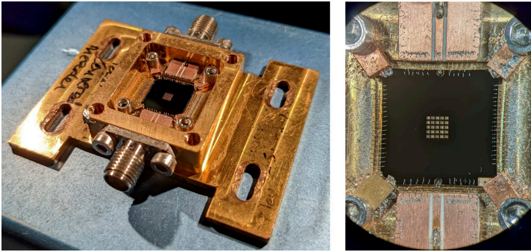
Figure 3.6: The MKIDs chip is mounted inside a gold-plated copper box and held in place by four clamps on each corner. We use aluminium wire bonding to connect the feedline to the two 50 \Omega SMA connectors via CPW stripboards. We also bond aluminium wires all across the chip to define a common ground as well as thermal bridges with the box to ensure an effective thermalisation.
