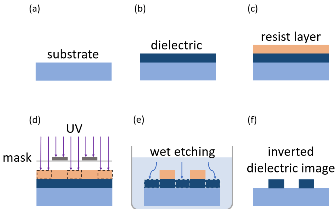
Figure 3.3: (a) On a clean substrate, (b) a dielectric is deposited using Atomic Layer Deposition (ALD). (c) A single resist layer is spin-coated and (d) the undesired structures are exposed to UV light. (e) Once the resist has been developed, the unwanted parts of the dielectric are removed by wet etching and (f) the resulting dielectric image is inverted compared to the photomask.
