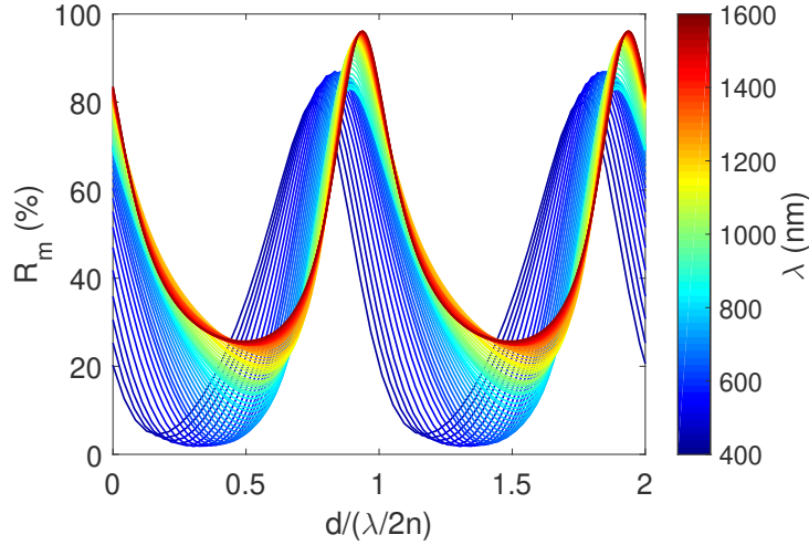
Figure 4.11: Modelled reflectance off the whole optical stack with a 60 nm thick TiN 6 scm layer, an \text{Al}_2\text{O}_3 layer with a variable thickness d and a 40 nm thick aluminium reflector layer. The thickness d is normalized by the guided half-wavelength \lambda/2n with n the \text{Al}_2\text{O}_3 refractive index.
