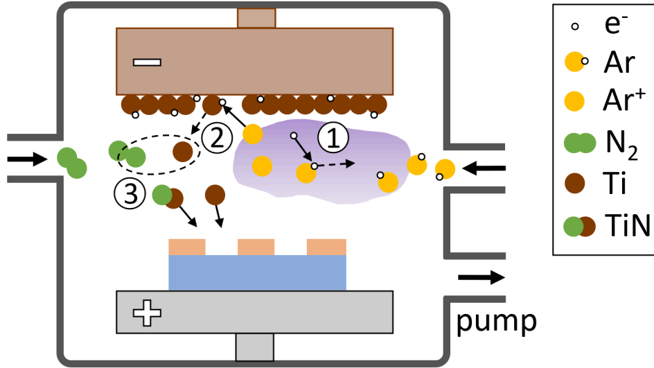
Figure 3.4: Reactive sputtering of TiN: (1) An argon gas fed into the chamber is ionized by electrons from the titanium target and creates a plasma (in purple) kept close to the target thanks to the magnetron. (2) The argon ions are accelerated towards the target and eject titanium atoms outwards where (3) they may or may not react with the nitrogen flow to form a sub-stoichiometric \text{TiN}_x film.
