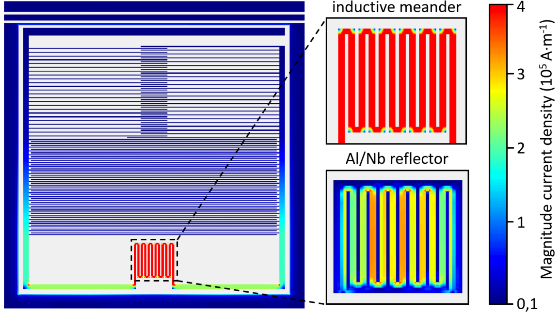
Figure 4.23: Colormap representing the magnitude of the current density J in the pixel at the resonance frequency. Top right: close-up view of the inductive meander where J is the highest. Bottom right: A significant part of the resonator current density is transferred to the reflector where the footprint of the meander is visible.
