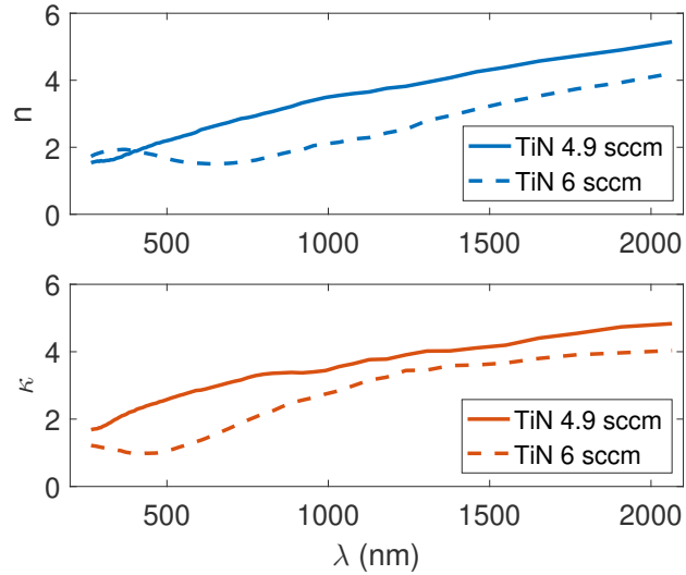
Figure 4.14: Measurements by ellipsometry of the real refractive index n and imaginary extinction coefficient \kappa of a sub-stoichiometric \text{TiN}_x film as a function of wavelength \lambda . The optical constants of TiN 6 sccm first shown in Fig. 4.9 are represented again here in dashed lines for comparison.
