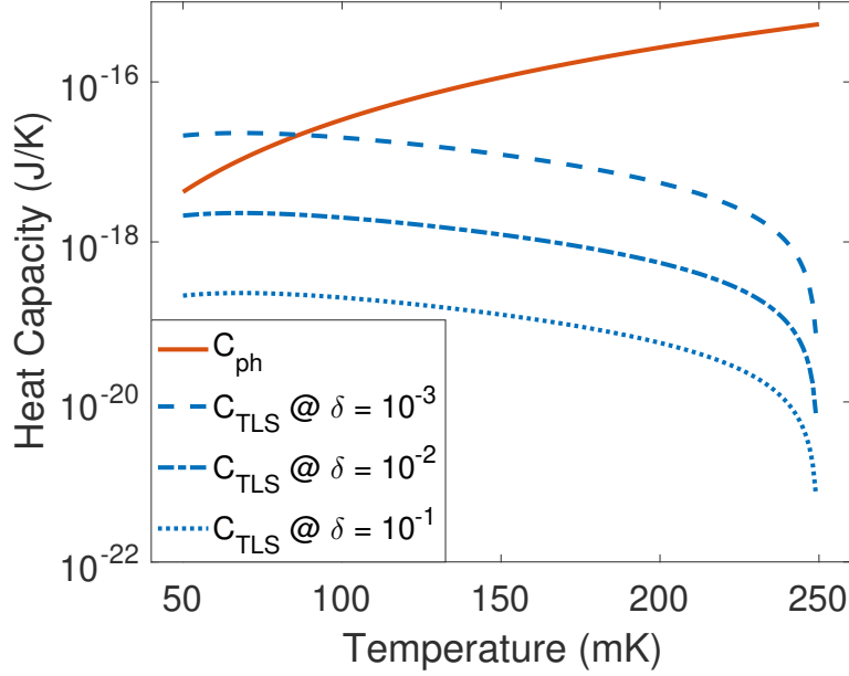
Figure 5.7: Semilog plot of the expected heat capacity of phonons and TLS for different values of dielectric tangent loss. The electron heat capacity is not represented here as it is negligible next to phonons and TLS.
