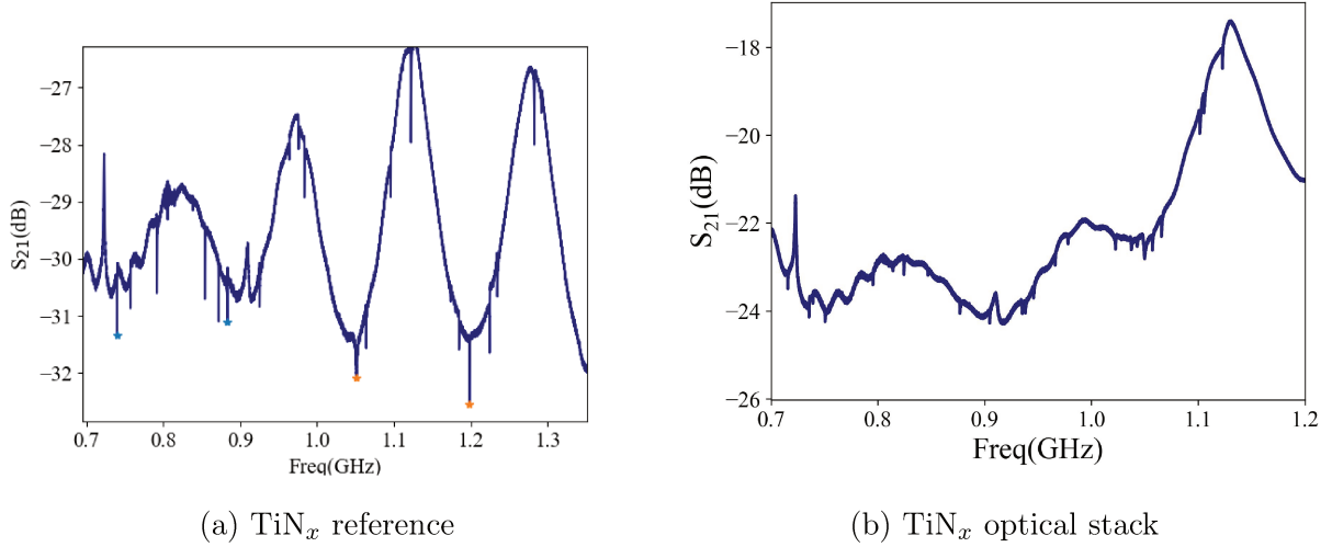
Figure 4.25: Magnitude of S_{21} of (a) the reference sample with TiN x and (b) the optical stack sample with TiN x .
