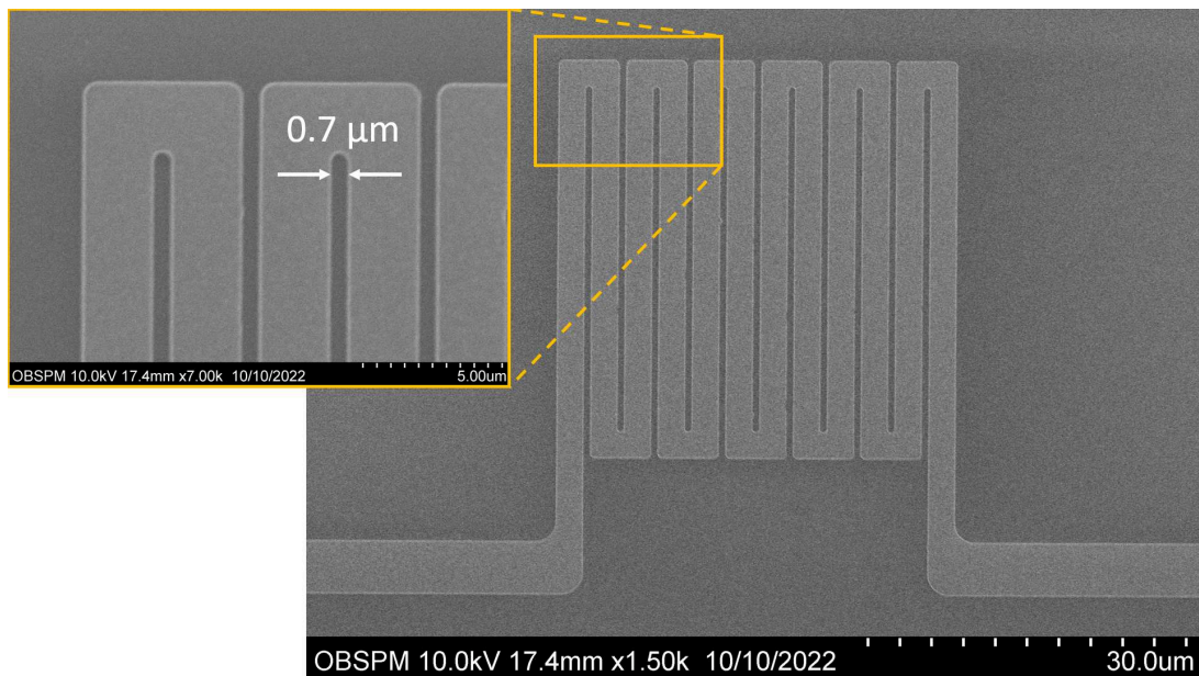
Figure 3.2: Image of an inductive meander taken with a Scanning Electron Microscope (SEM). The photolithographic technique allows us to pattern elements with a resolution down to 0.7\ \mu\text{m} as seen here with the meander gaps.
