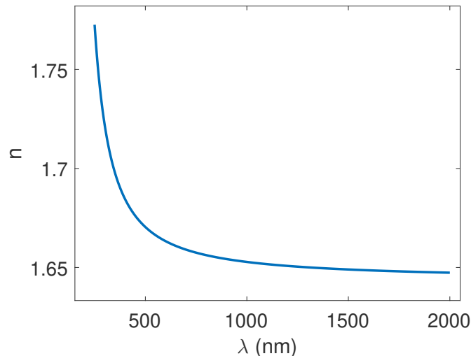
Figure 4.6: Real refractive index of an Al 2 O 3 layer measured by ellipsometry.
