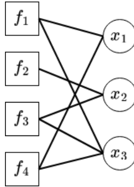
Figure 6.1: Factor graph of an additive decomposition, with n = 4 factors and d = 3 variables.
