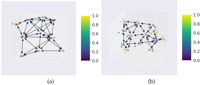
Figure 4.2: Topologies \mathbf{T}_1 and \mathbf{T}_2 . APs are shown as red triangles, conflicts between APs as double-headed arrows, and STAs as colored dots. Their colors show how frequently a given STA has a reasonable throughput ( i.e. is not in starvation) with the 802.11ax default configuration. A cool color means that the STA is often in starvation, while a warm color denotes a STA that is never in such a situation.
