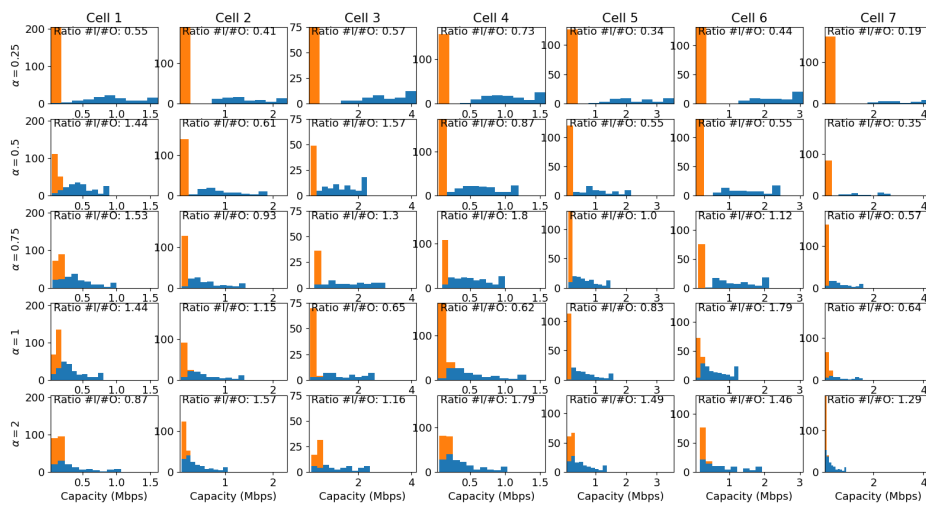
Figure C.1: Throughput distribution of the cells in T_1 and different values of \alpha . The throughput distribution of the users in the inner areas is depicted with a blue histogram, the throughput distribution of the users in the outer area is depicted with an orange histogram. For each cell, the ratio between the number of inner users and outer users is given.
