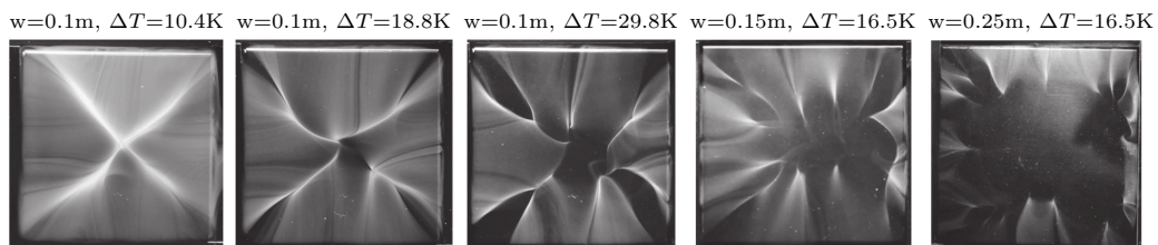
Figure C.9 – Visualized flow fields over upward-facing squared plates [23]
