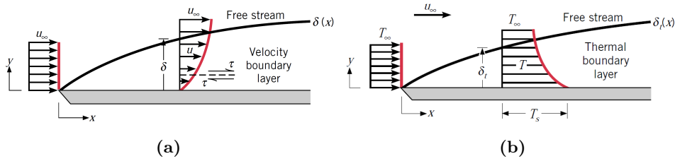
Figure C.2 – (a) Velocity boundary layer (b) Thermal boundary layer [38]
