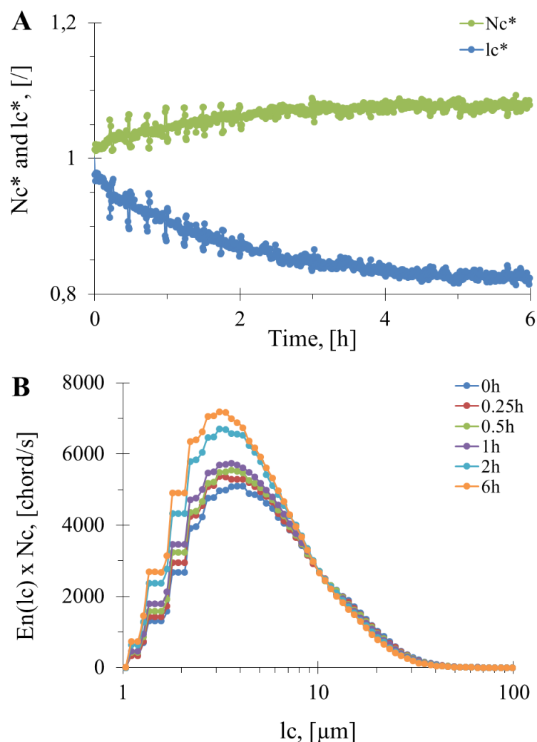
Figure 4-8. Evolution of particle size and number by focusing on the finest population during the deconstruction of milled destarched wheat bran by Rovabio Brussel. This evolution is reported as the normalized number of count per second ( Nc^* ) and the normalized mean chord length ( lc^* ) as a function of the time (A) and the number distribution of chord length multiplied by the number of particle (B). Operating conditions are identical to Fig.4-2.
