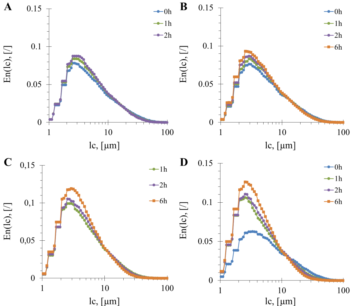
Figure 2-14: Chord length ( l_c ) number distribution of wheat bran suspension during hydrolysis with Rovabio Brussel with 1.1 U/gdm (A), 11 U/gdm (B), 380 U/gdm (C) and 1100 U/gdm (D). Operating conditions identical to Fig.2-9.
