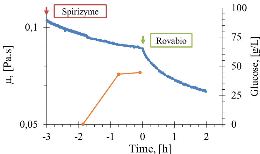
Figure 2-4. Change of in-situ viscosity during the treatment of wheat bran suspension with Spirizyme and then Rovabio (Brussel). Operating conditions: wheat bran suspended in a potassium phosphate 0,1M at 41°C, pH 4.0, initial concentration 157 gdm/L, Spirizyme 5 AGU/gdm and Rovabio Brussel 1.1 Uxylanase visco/gdm.
