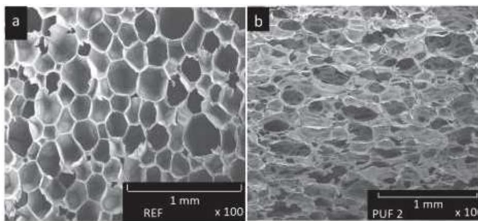
Figure 2.6: SEM images of PUF in the rise direction, a: close cell from the reference foam (REF). b: open cells from biobased PUF (PUF 2)
