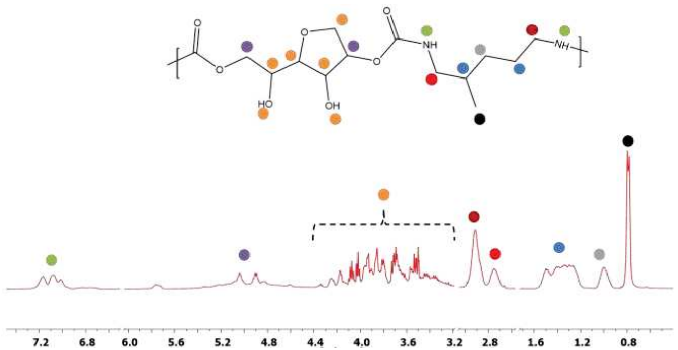
Figure SI 62: ^1\text{H-NMR} of PHU-D sample
