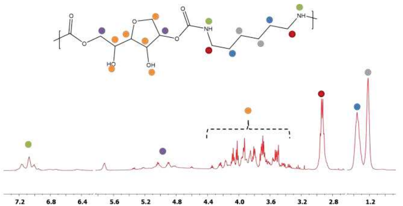
Figure SI 63: ^1\text{H-NMR} of PHU-H sample
