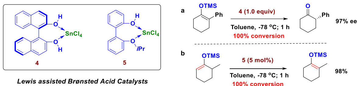
Scheme 1.9. Lewis acid-assisted Brønsted acid catalysis; (a) Enantioselective protonation with chiral LBA; (b) Isomerization of silyl enol ethers.
