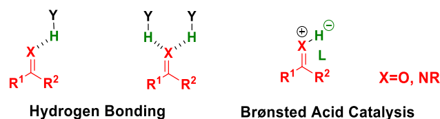
Figure 1.5. Formation of active species.
