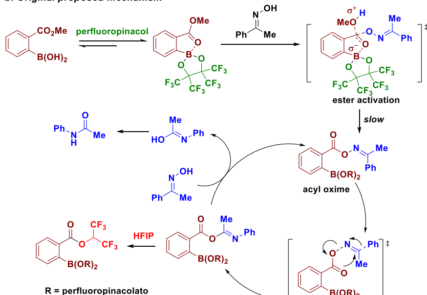
b: Original proposed mechanism
