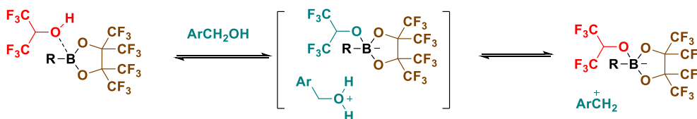
Scheme 2.7. Mechanistic proposal for the activation of the benzyl alcohols.
