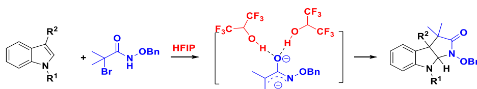
Scheme 1.3. [3+2]-Cycloaddition of indoles with \alpha -haloamides.
