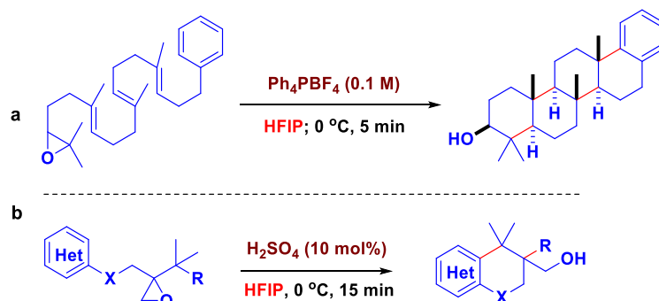
Scheme 1.35. Cyclization of epoxides.
