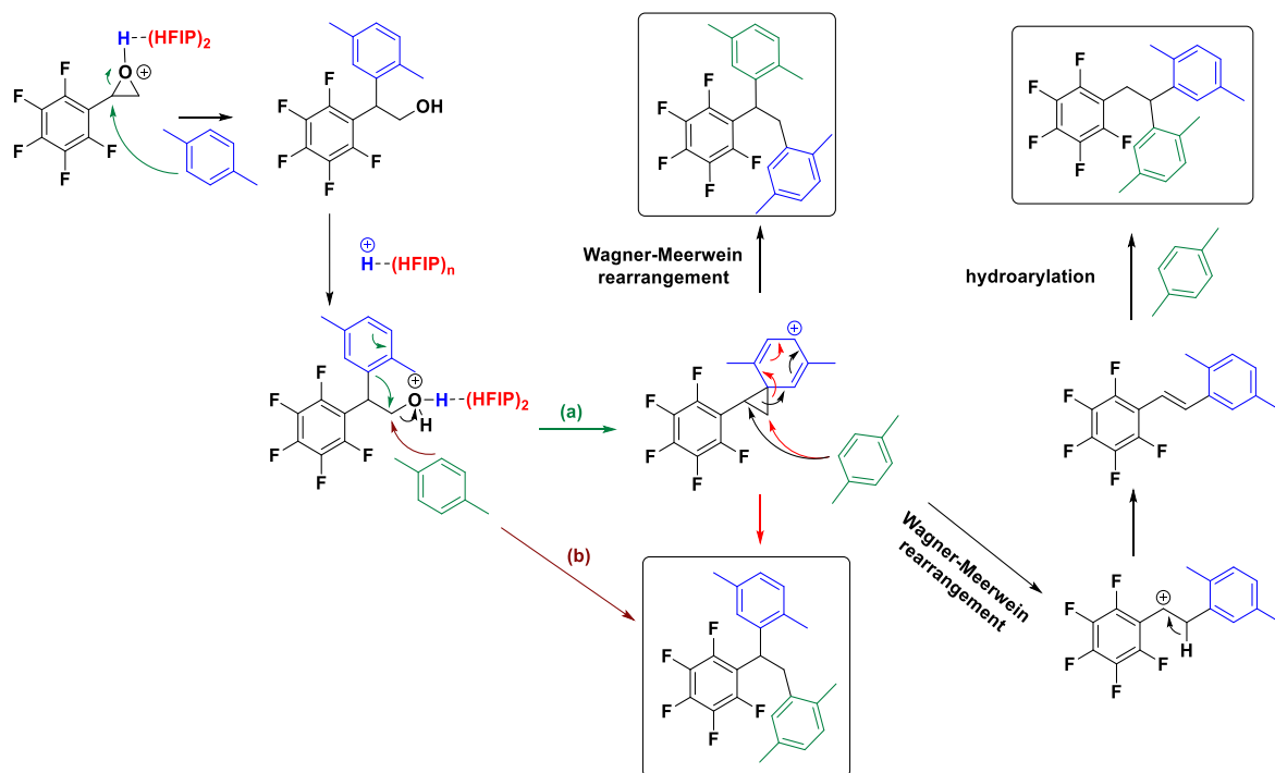
Figure 3.4. Proposed mechanism for 1,2-difunctionalization of epoxides.
