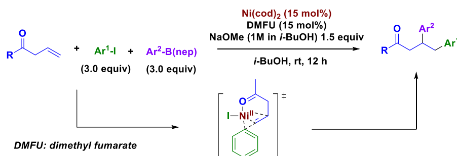
Scheme 1.28. Ni-catalyzed 1,2-difunctionalization of alkenyl ketones with a nucleophile and an electrophile.
