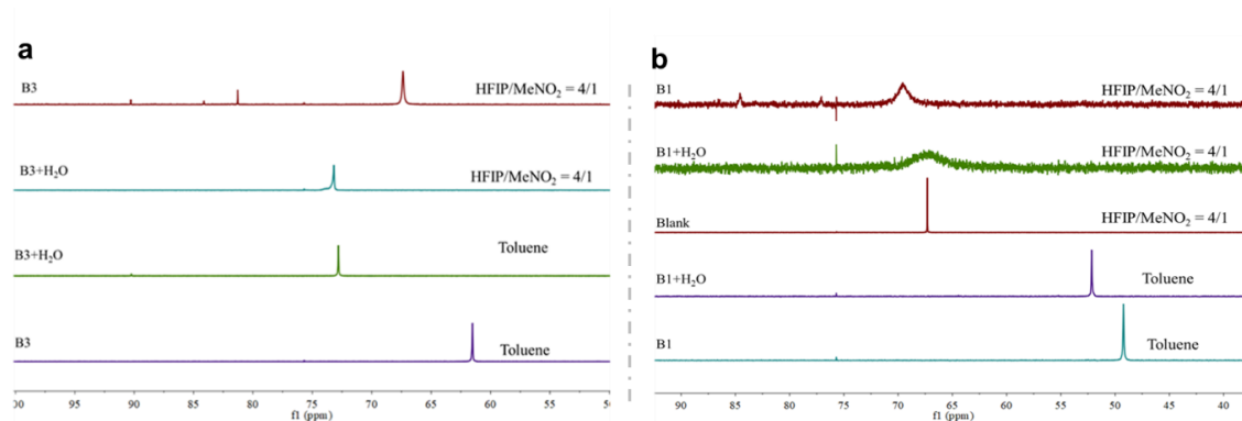
Blank = 0.075 mmol triethylphosphine oxide dissolved in a mixture of hexafluoroisopropanol and nitromethane (4:1); The ^{31}\text{P} NMR of ( B + H 2 O) was done after added water (3.0 equiv) about 4 h.
