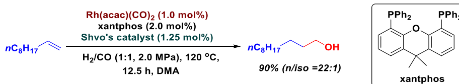
Scheme 4.4. One-pot hydroformylation–hydrogenation of 1-decene with two different catalysts.
