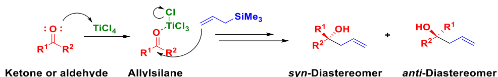
Scheme 1.4. Sakurai allylation. 35
