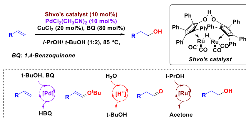
Scheme 4.3. Anti-Markovnikov selective hydration of olefins via triple relay catalysis.
