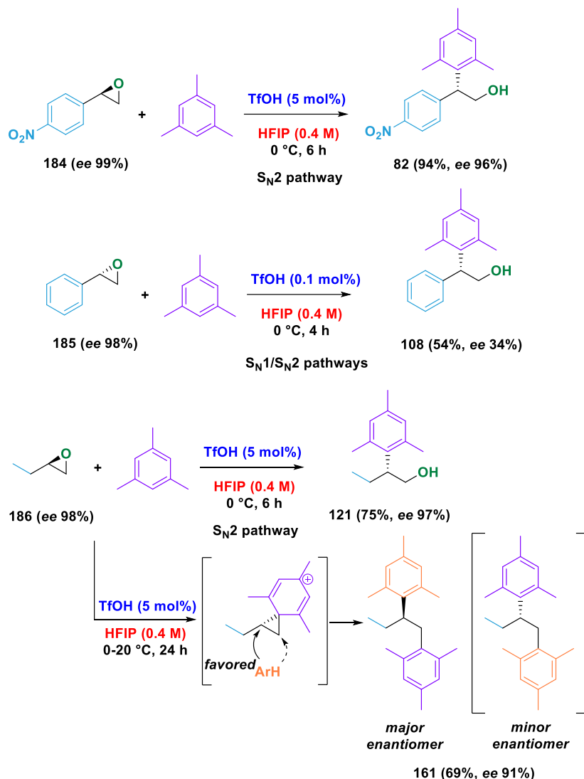
Scheme 3.4. Stereochemical studies.
