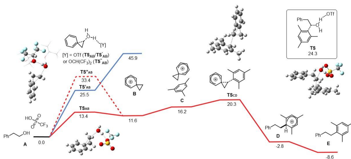
Figure 3.3. Gibbs energy profiles ( \Delta G , kcal mol -1 ) for the addition of mesitylene to 2-phenyl ethanol.
