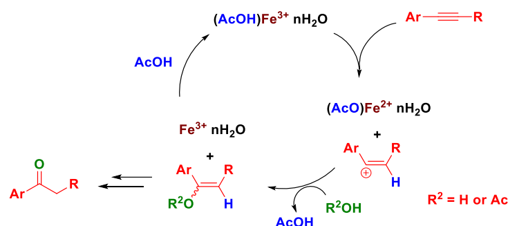
Scheme 1.10. Plausible catalytic cycle.
