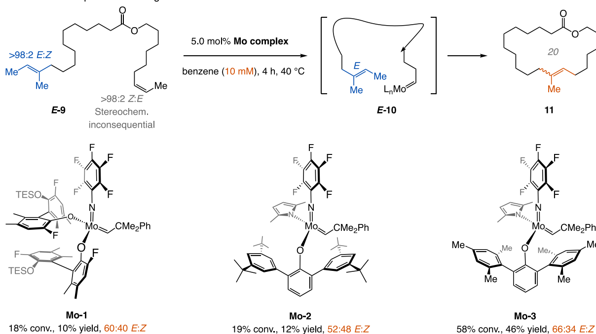
Scheme 5. Unexpected Challenges for Stereoretentive MCRM
