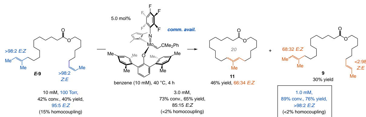
Scheme 6. Problem and Solution for Pre-Metathesis Isomerization
