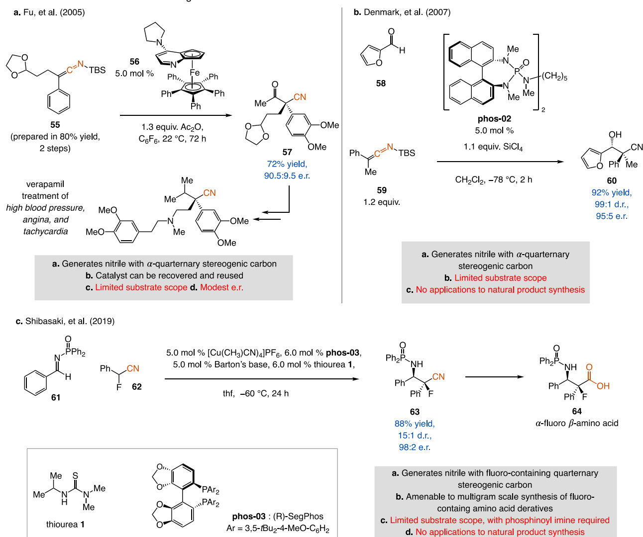
Scheme 13. Transformations Involving Ketene Imines
