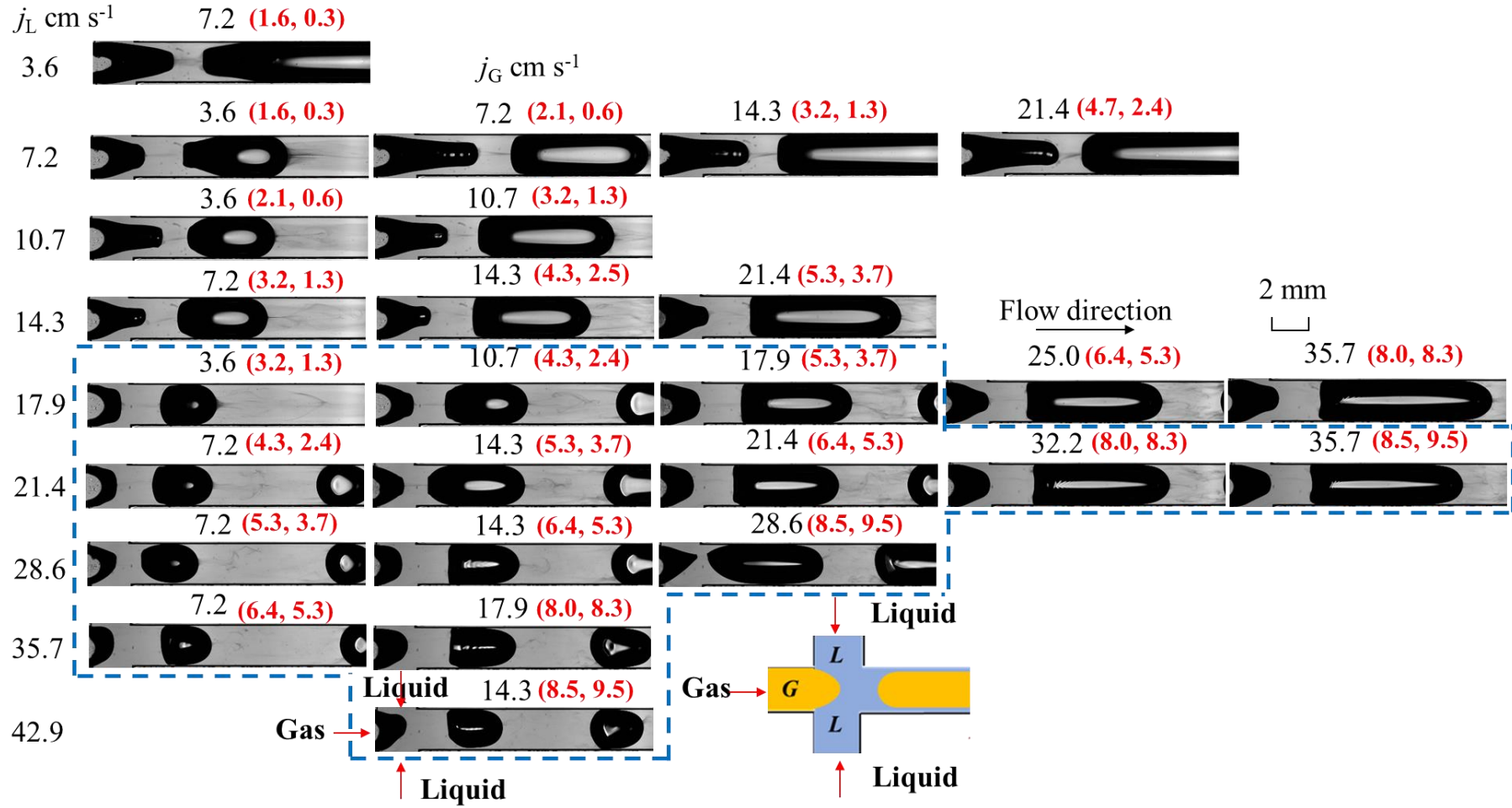
Fig. 5-4 Cartography of the instantaneous gas-liquid Taylor flows (air and RGN colorimetric solution) right after the bubble pinch-off at the cross-junction position X_1 = 0 , for various operating conditions. The dimensionless numbers in the red brackets correspond to (Ca_{TP} \times 10^{-3}, We_{TP}) . Pinch-off patterns I and II are located inside and outside of the dotted blue box respectively.
