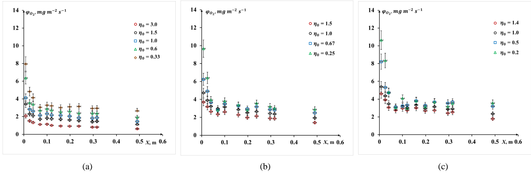
Fig. 6-9 Evolution of mass flux density versus axial positions X under different operating conditions: (a) j_{TP} = 28.6\ cm\ s^{-1} ; (b) j_{TP} = 35.7\ cm\ s^{-1} ; (c) j_{TP} = 42.9\ cm\ s^{-1} .
