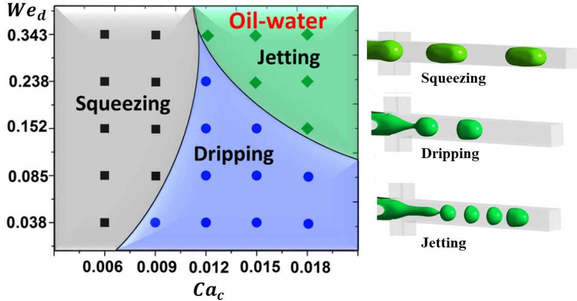
Fig. 1-6 Flow pattern maps of droplet formation in a cross-junction microchannel (600×600 μm) containing for oil–water ( Ca_c and We_d represent the continuous Capillary number and dispersed Weber number). Adapted from Sontti and Atta (2019).
