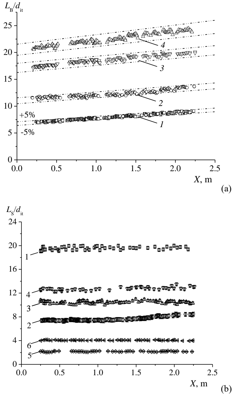
Fig. 3-5 In-plane spiral-shaped milli-reactor (a) dimensionless bubble length versus axial position X at j_L = 1.8 cm s ^{-1} for the ET configuration: (1) j_G = 1.4 cm s ^{-1} ; (2) j_G = 2.8 cm s ^{-1} ; (3) j_G = 5.1 cm s ^{-1} ; (4) j_G = 6.9 cm s ^{-1} ; dash-dotted line: the \pm 5\% confidence interval. (b) Dimensionless liquid slug length versus axial position X at different conditions: (1) j_L = 7.2 cm s ^{-1} , j_G = 0.9 cm s ^{-1} , ET; (2) j_L = 7.2 cm s ^{-1} , j_G = 3.3 cm s ^{-1} , MT; (3) j_L = 3.6 cm s ^{-1} , j_G = 1.1 cm s ^{-1} , ET; (4) j_L = 3.6 cm s ^{-1} , j_G = 0.9 cm s ^{-1} , MT; (5) j_L = 1.8 cm s ^{-1} , j_G = 16.6 cm s ^{-1} , ET; (6) j_L = 1.8 cm s ^{-1} , j_G = 3.2 cm s ^{-1} , MT.
