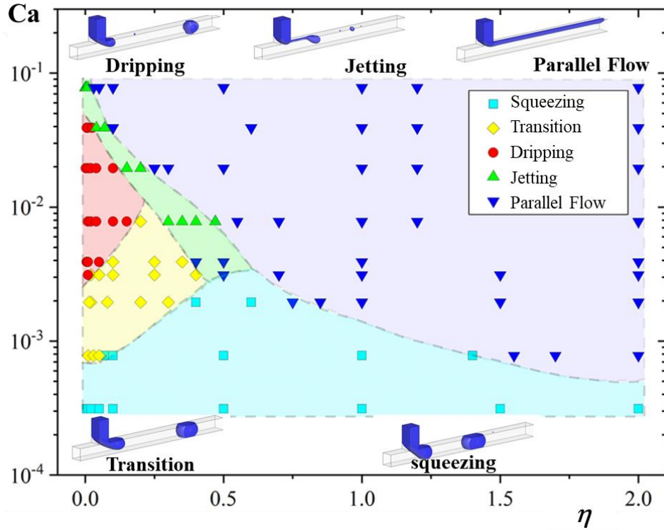
Fig. 1-7 Flow regimes of droplet formation as a function of Capillary number Ca_{TP} and gas-liquid superficial velocity ratio \eta in a T-junction ( 100 \times 100 \mu\text{m} ) with contact angle at 135^\circ .
