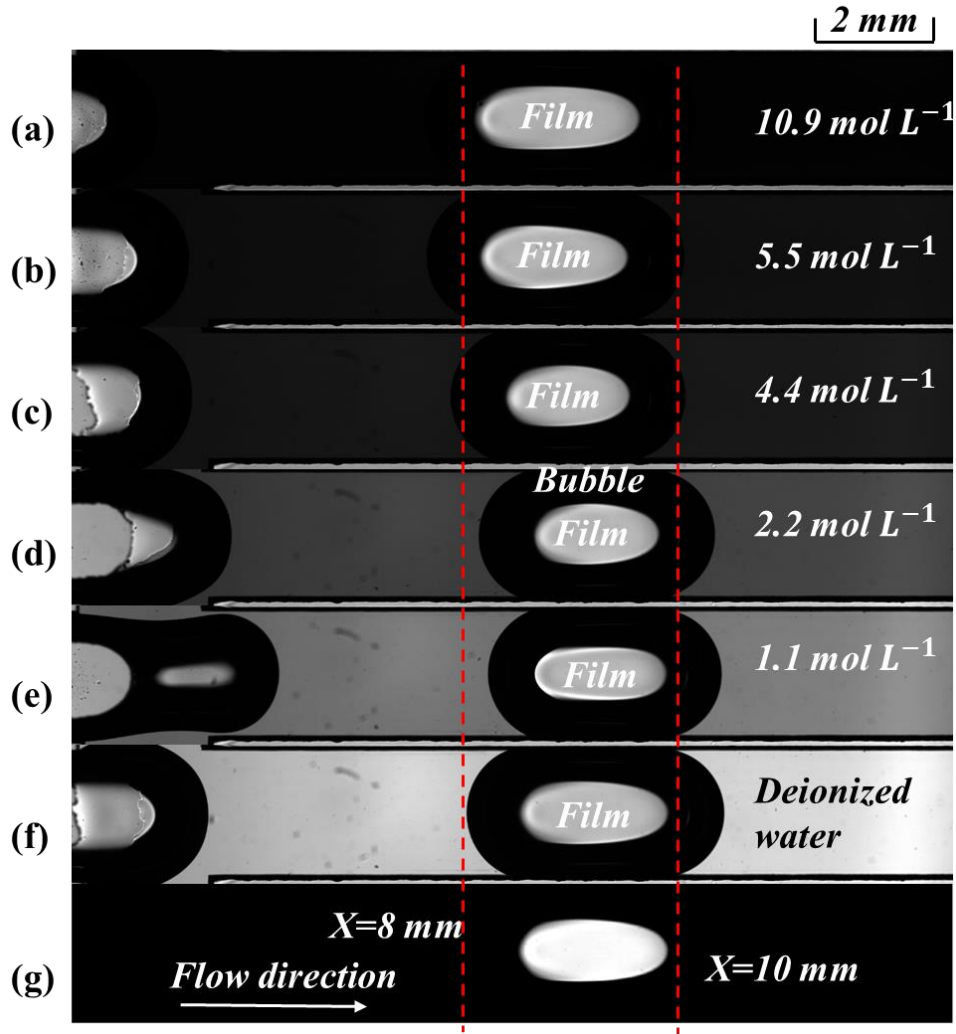
Fig. A 8-2 Bubble formation at the cross-junction in milli-channel: image sequences of developed liquid film for air and various concentrations of RZ dye, (a) to (e): [\text{RZ}] = 10.9, 5.5, 4.4, 2.2, 1.1\text{ mol L}^{-1} and deionized water; (g) extracted liquid film by Matlab for image (f). Operating condition: j_L = 10.7 and j_G = 3.6\text{ cm s}^{-1} , \text{Ca} = 2.3 \times 10^{-3} , \text{Re}_{\text{TP}} = 277 .
