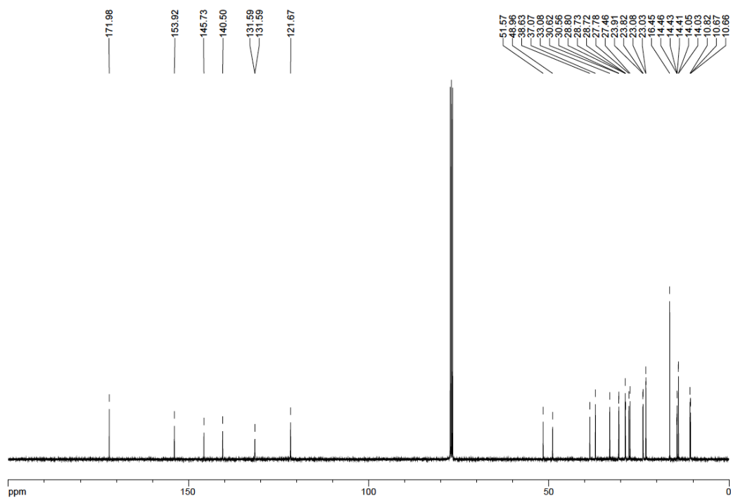
13 C NMR spectrum of BDP-2C 8
