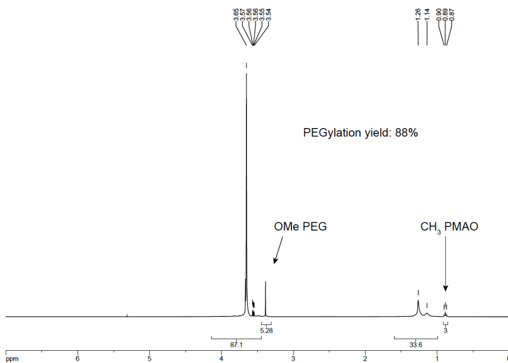
1 H NMR spectrum of FP1 (CDCl 3 , 400 MHz)
