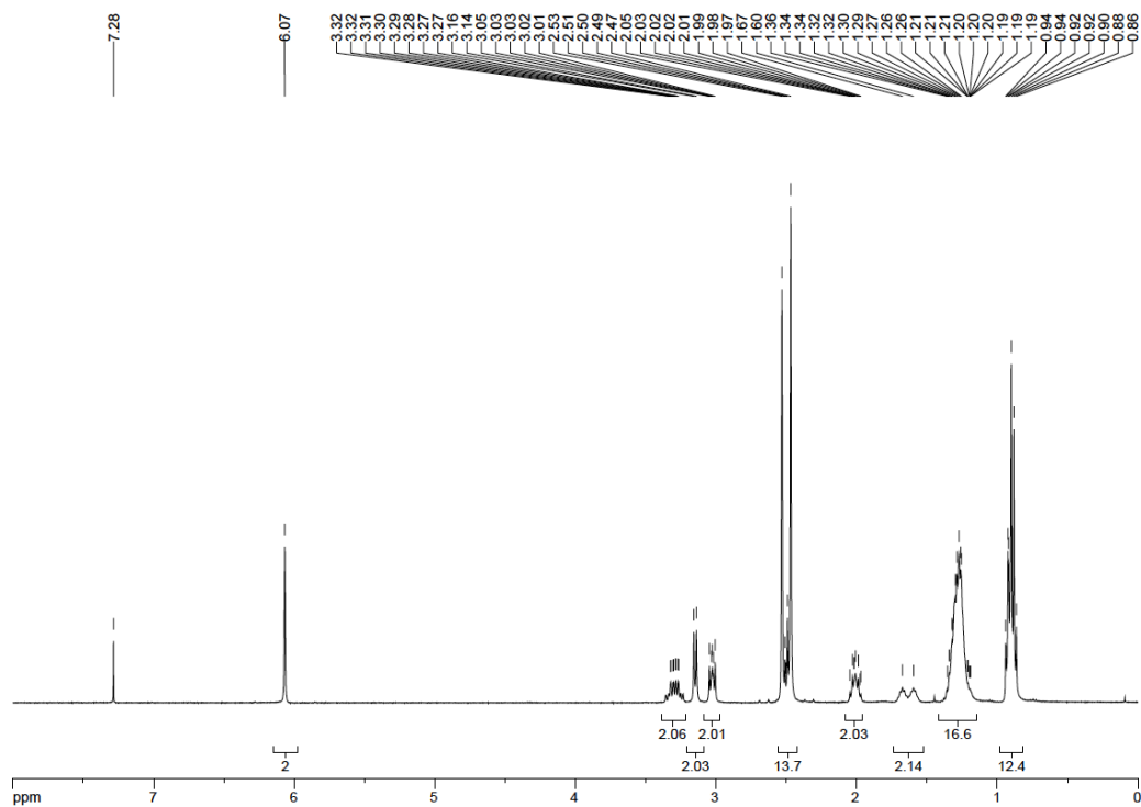
1 H NMR spectrum of BDP-2C 8
