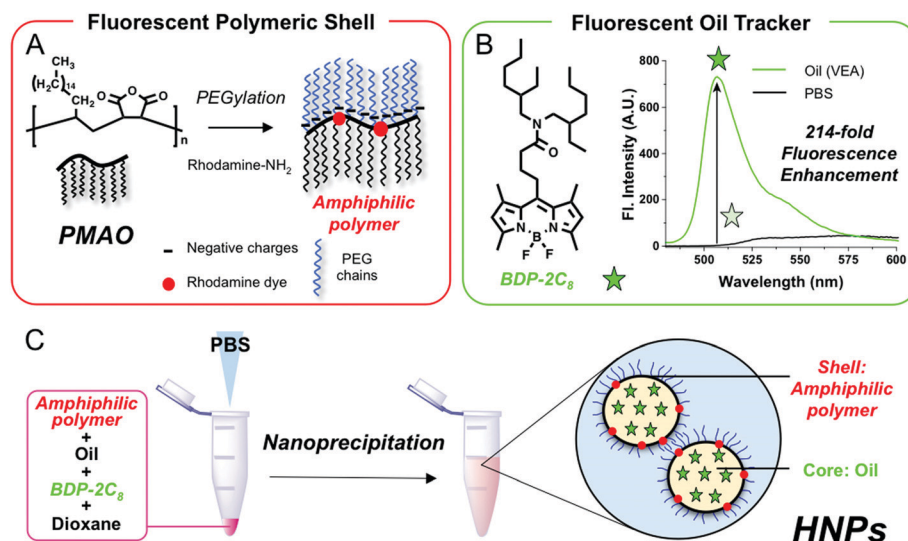
Fig. 1 (A) Synthesis of fluorescently labeled amphiphilic polymers. (B) Development of the fluorescent oil tracker based on BODIPY BDP-2C 8 and its fluorescent spectra at 1 μM in PBS and in oil. (C) Formulation of HNPs by nanoprecipitation and their schematic representation.
