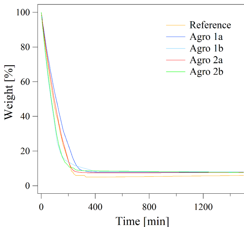
Figure 8 – Dehydration (50 °C) kinetics of sEPS hydrogels obtained according to different protocols.
