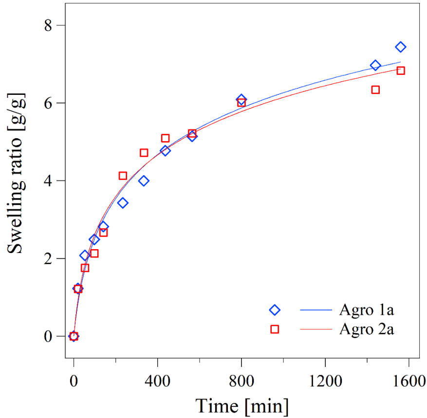
Figure 11 – Experimental swelling kinetics in 2 % (w/v) KNO 3 aqueous solution of sEPS hydrogels obtained according to different protocols and related fits via Elovich model. The swelling ratios are related to the weight of hydrogel dehydrated at 50 °C.
