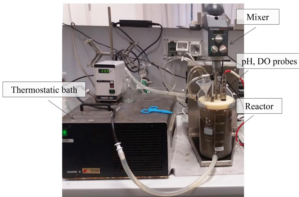
Figure A.1 – Apparatus used for the respirometric experiments carried out on AGS-extracted sEPS and derived hydrogels.
