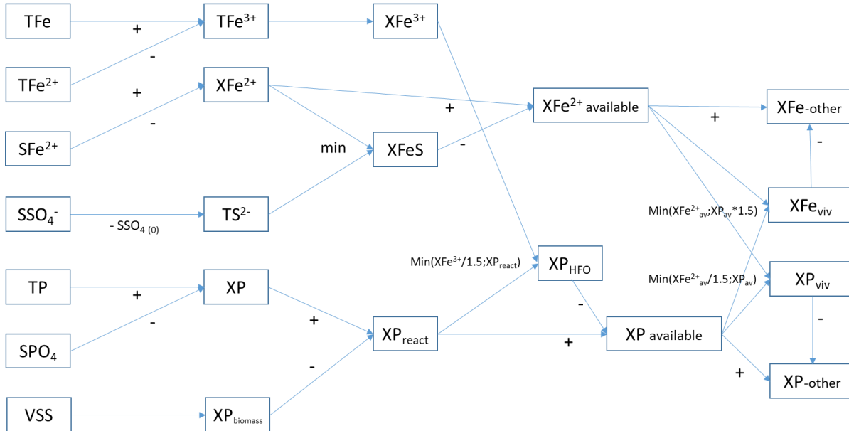
Figure S3. 1. Schematic diagram of the calculation method for determination of Fe, P fractionation. Notation: T for total concentrations particulate with X and soluble with S. Measured components: Total iron (TFe); Total iron(II) (TFe 2+ ); soluble Fe(II) (SFe 2+ ); Total phosphorus (TP); orthophosphate (SPO 4 ); sulphate (SSO 4 ). Calculated components: Ferric iron (XFe 3+ ); particulate ferrous (XFe 2+ ); consists of FeS (XFeS), vivianite (XFe viv ), and other precipitates, and Particulate phosphorus (XP) consists of Fe 3+ bound Phosphorus, P in biomass (assumed to be constant); vivianite bound P and other P particulates.
