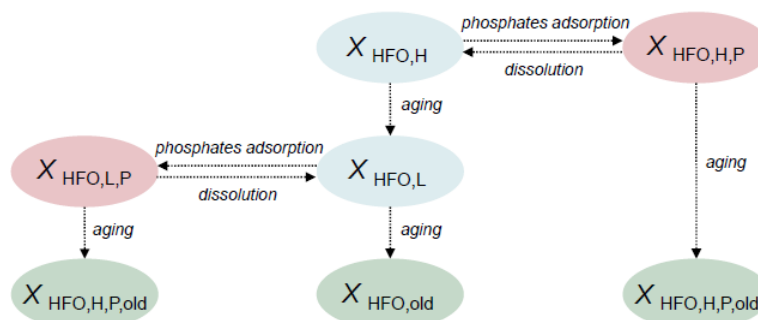
Figure 1.3-4 A simplified version of the HFO model coupled to ASM2d (Solon thesis, 2017)
