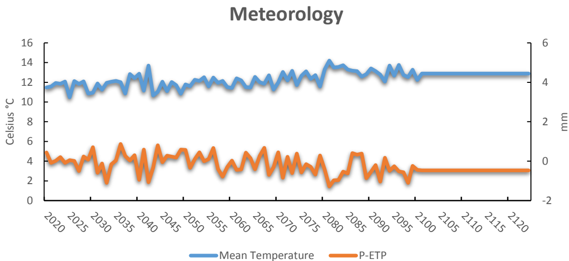
Fig. S1 Temperature and P-ETP inputs for AMG model, P-ETP is the difference of precipitation P and potential evapotranspiration ETP. Data from Drias(DRIAS les futurs du climat, 2014).
