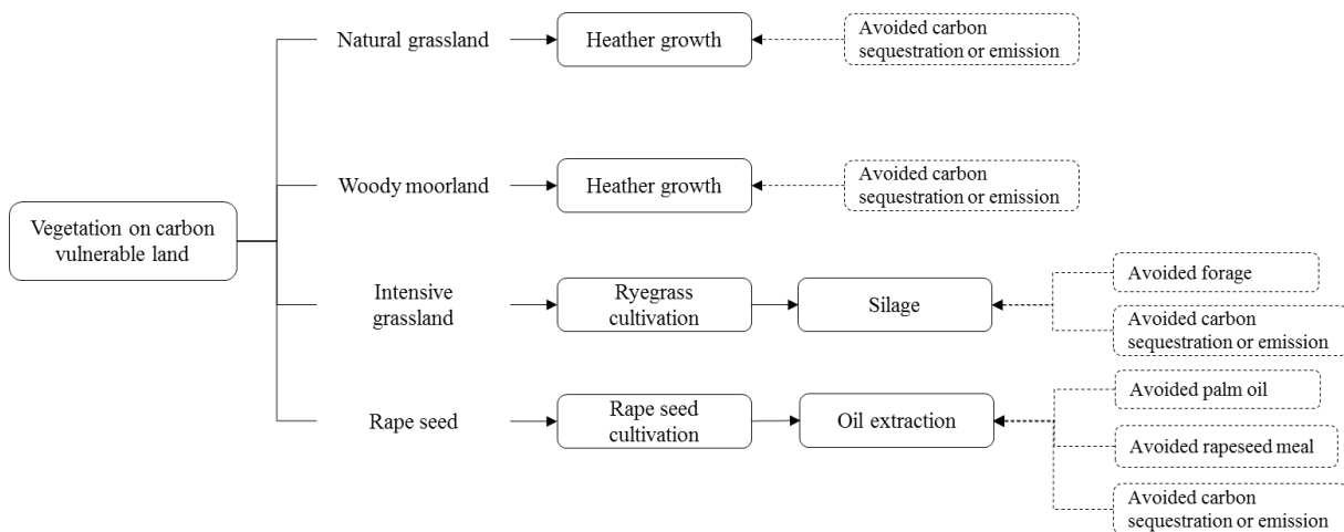
Fig. S3 Diagram of carbon vulnerable land use.
