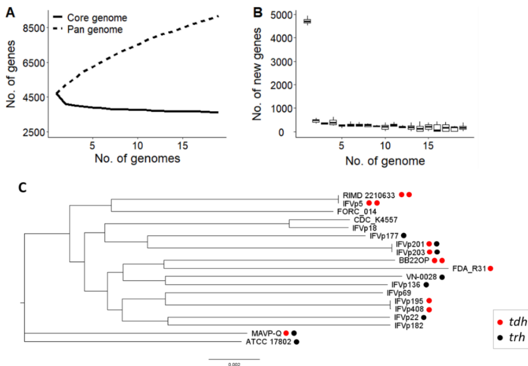
Fig 2. Pan-genome analysis and core-genome phylogenetic tree of the 19 Vp strains. (A) Estimated number of the core (3,616 genes) and pan-genomes (9,161 genes), and (B) number of new genes. (C) Maximum-likelihood tree obtained from concatenated nucleotide sequence alignment of core genes using RaxML with 100 bootstraps.
