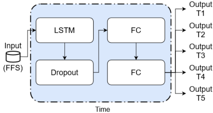
Figure 5.2: “ Full Interaction-LSTM ” (FI-LSTM) architecture. It uses the FFS features as input and integrates time dependencies between the thin slices of the last 2mn of each task using an LSTM layer.
