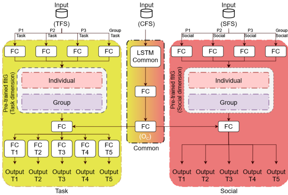
Figure 5.6: “ Common to Specific ” (CTS) architecture. It is composed of three modules (i.e., Task , Social and Common ). Social and Task modules independently process features from Social- and Task-specific subsets, respectively to learn a dimension-specific representation of behavior, enriched by the Common module. CTS predicts, for each task, both dimensions in a multitask setting.
