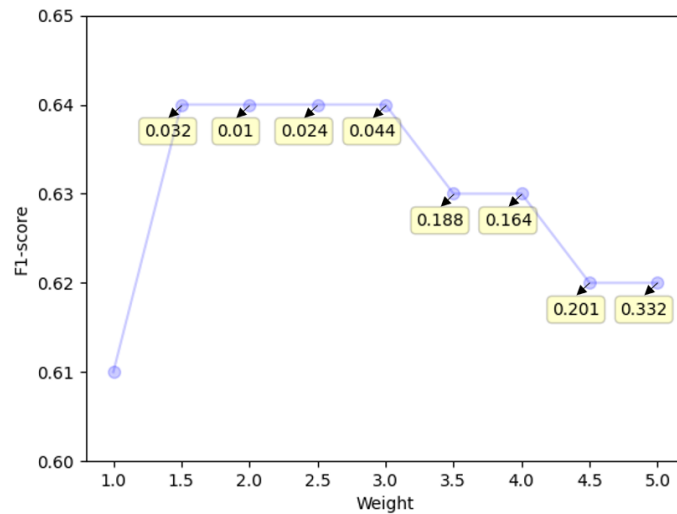
Figure 6.5: Average F1-score over 15 randomly extracted seeds of the fltG model, for the prediction of the Task dimension of cohesion with the Weighting approach. Weights ranging from one to five are applied to the features. For each weight, p-values (in yellow) indicate whether or not there is a significant difference with the baseline (weight 1).
