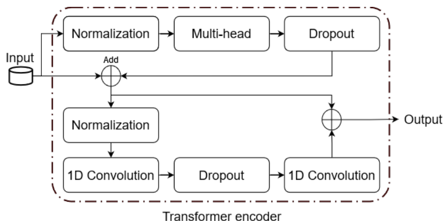
Figure 5.5: Architecture of the transformer-encoder (Vaswani et al., 2017).
