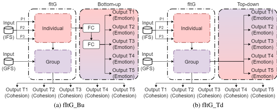
Figure 6.2: FltG_Bu (Figure 6.2a) predicts group valence emotion after the Individual module of the fltG and reflects a Bottom-up approach (i.e., individuals influence the group). FltG_TD (Figure 6.2b) predicts group valence emotion after the Group module of the fltG and implements a Top-down approach (i.e., the group influences each individual).
