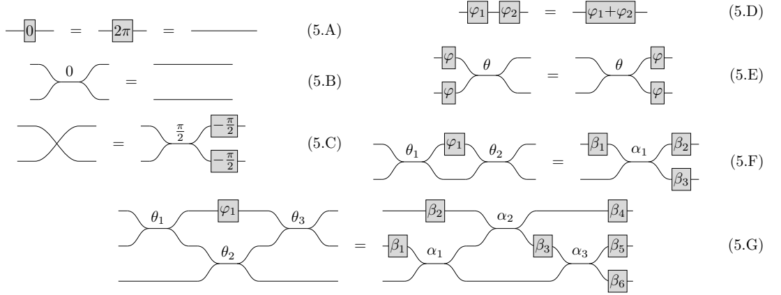
Figure 5.12: Axioms of the \text{LO}_{\text{PP}} -calculus. The equations are valid for arbitrary parameters \varphi, \varphi_i, \theta, \theta_i \in \mathbb{R} . In Equations (5.F) and (5.G), the angles on the left-hand side can take any value while the right-hand side is given by Lemma 5.13 and Lemma 5.12 respectively.
