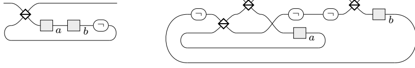
Figure 7.1: Two examples of bare PBS-diagrams, with the same word path semantics: (D, \mathbf{H}, 0) \xrightarrow{abab} (\mathbf{H}, 0) and (D, \mathbf{V}, 0) \xrightarrow{c} (\mathbf{V}, 0) .
