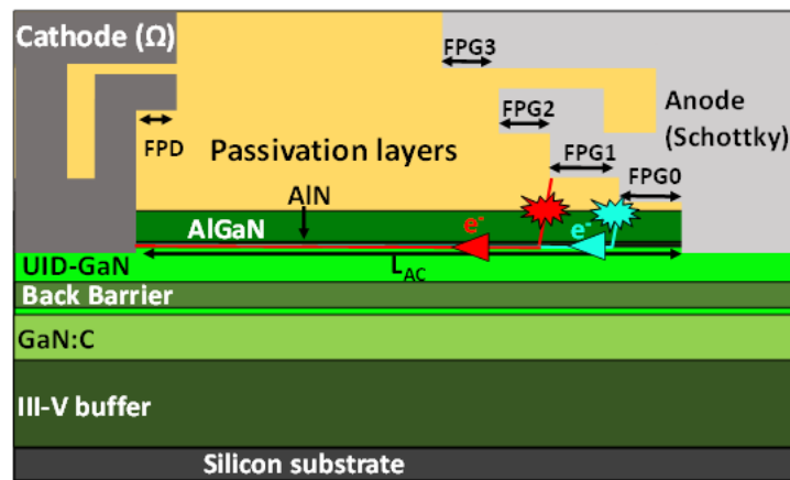
Figure 70: Schematic cross-section of the diode representing the post-breakdown electron flow for two layout categories: 1/ long anode-to-cathode layouts in red ( L_{AC} > 20 \mu\text{m} ) and 2/ Layouts having a sixteen-micrometer anode-to-cathode distance in cyan.
