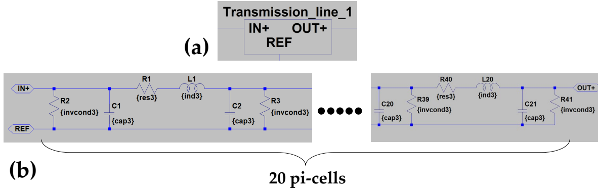
Figure 172: Lossy transmission line implemented model with 20 pi-cells (a) symbol and (b) real implementation ( \text{res3} = R_L \times L/20 ; \text{ind3} = L_L \times L/20 ; \text{invcond3} = G_L \times L/21 ; \text{cap3} = C_L \times L/21 ).
