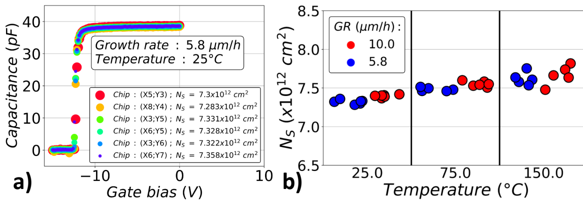
Figure 92: (a) Gated Van Der Pauw capacitance versus voltage characteristic [301] (b) Electron density (extracted from the Gated Van der Pauw measurements) as a function of the temperature for two different growth rates [301].
