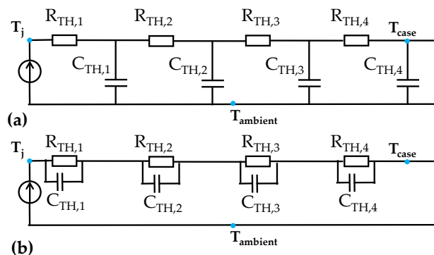
Figure 180: Thermal models: (a) Cauer model (b) Foster model.
