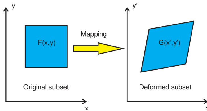
Figure 2-5. Principle of DIC
