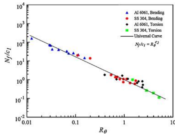
Figure 1-21. Universal curve of N_f/c_1 versus R_\theta [148]
