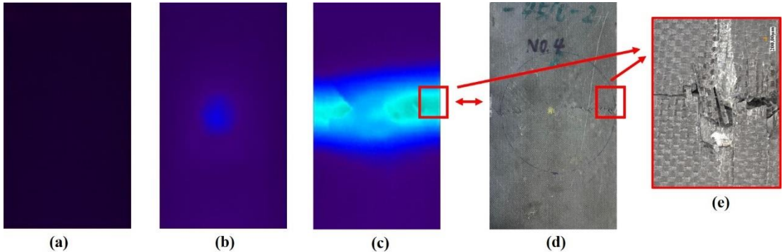
Figure 5-23. Thermographic images and damage characteristics: (a) - (c): thermographic images in different stages; (d) specimen profile after failure (front impacted surface); (e) fracture at one edge of the specimen observed by optical microscope
