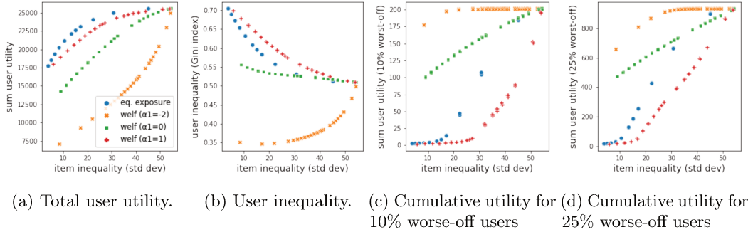
Figure A.8: Results on Movielens when measuring inequalities between items with the standard deviation.
