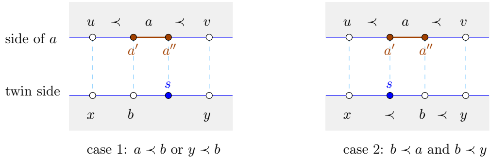
Figure 1.15: The twin splitting operation for an anchor a : it combines a splitting anchor operation on a (in brown) and an edge subdivision (in blue) incident to its twin b . Twin relations are with dotted lines. In this representation, the focus on the twin sides creates the illusion that the inside part of the embedding (in gray) is a disconnected region, which is not true. However, in this representation choice, the inside part, that is locally planar, may appear twisted if fully represented in the non-oriented surface case.
