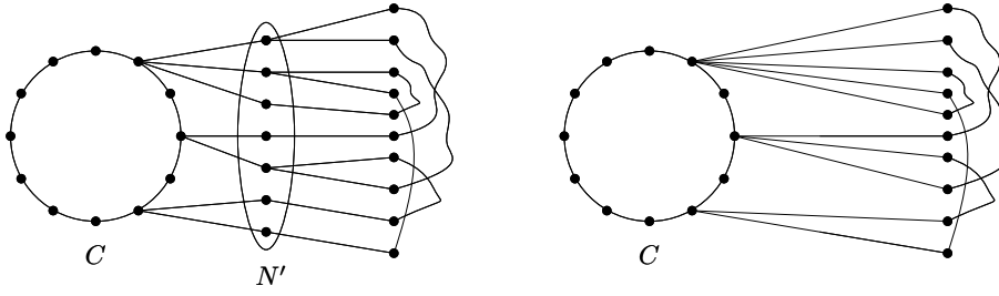
Figure 2.8: The graphs G_3 (left) and G_4 (right) in the proof of Claim 2.3.43.
