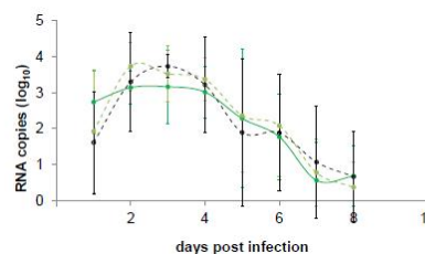
Avian influenza Virus shedding pattern in the turkey model
