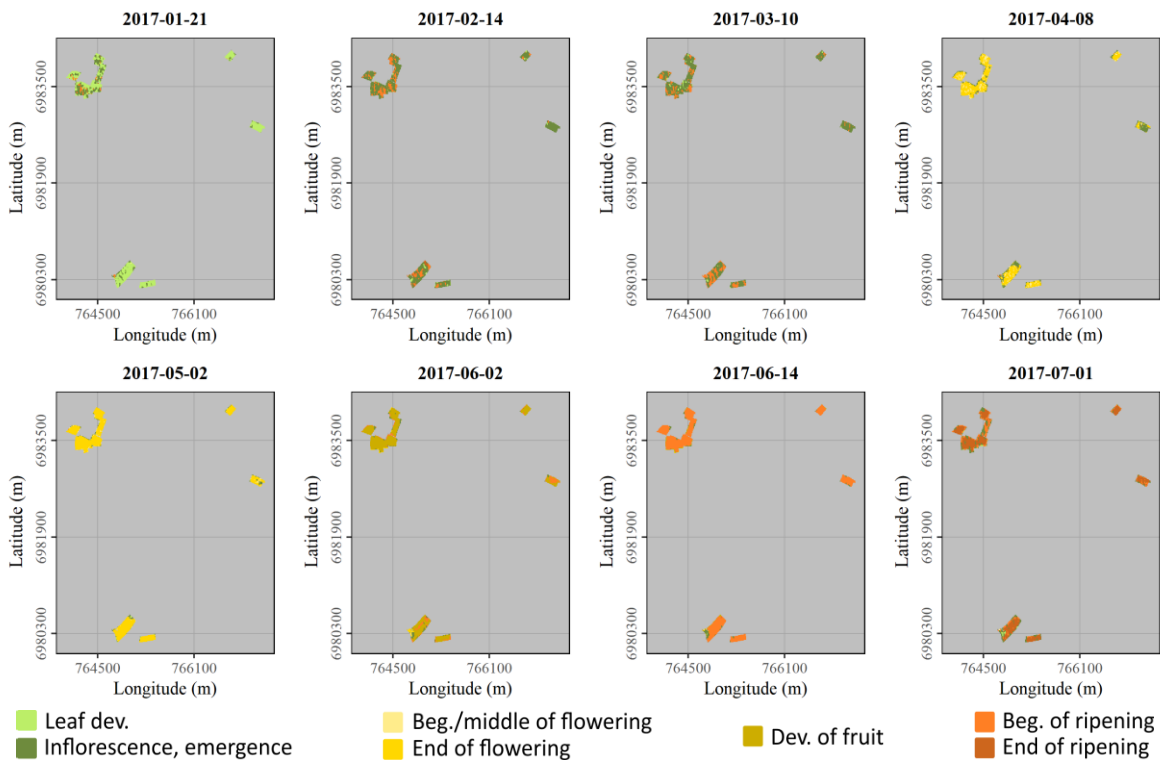
Appendix D-8. Classification of the 7 secondary phenological stages of rapeseed in the bocage study site using combined Sentinel-1 & 2 data.
