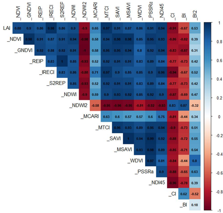
Appendix A-2. Correlation matrix of features derived from S-2 images for wheat
