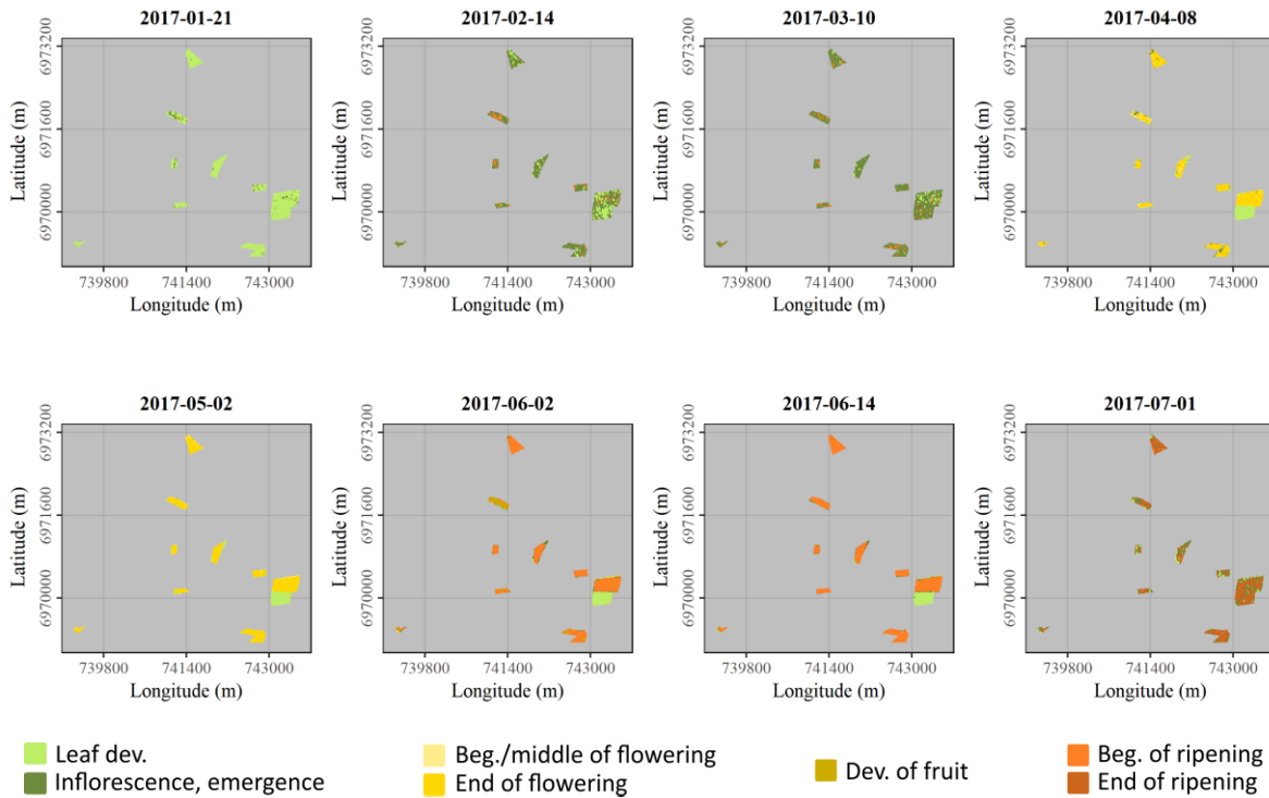
Appendix D-8. Classification of the 7 secondary phenological stages of rapeseed in the bocage study site using combined Sentinel-1 & 2 data.
