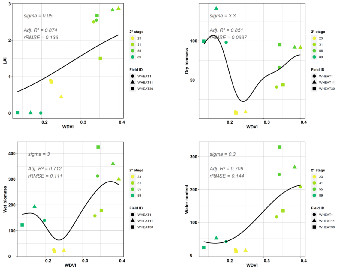
Appendix H-1. Relationships between wheat leaf area index, dry biomass, wet biomass, and water content and WDWI derived from S-2. .
