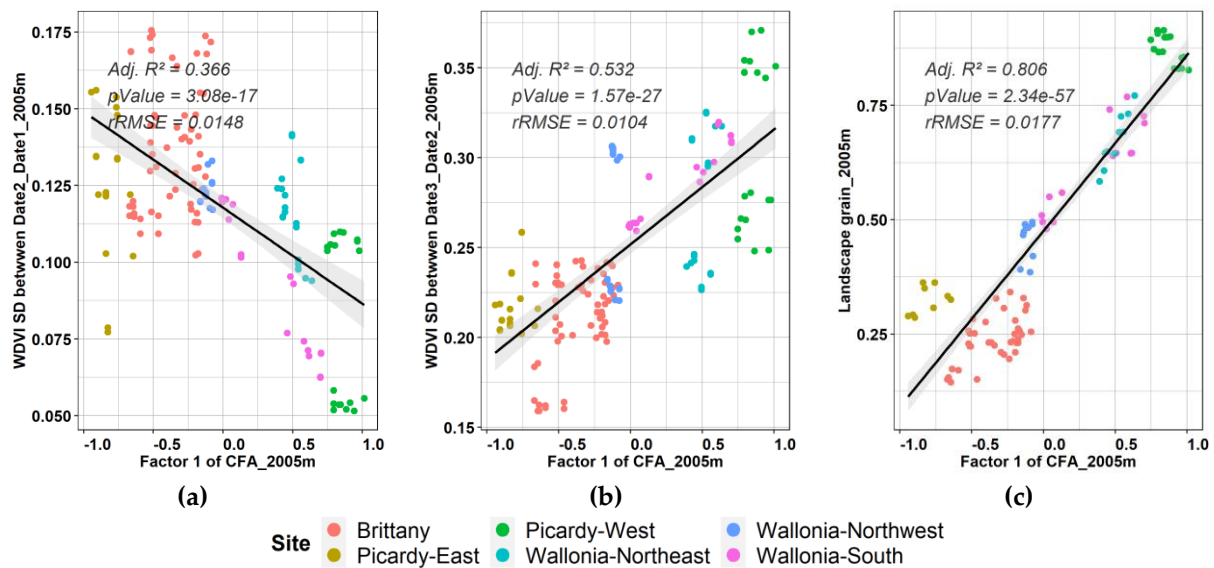
Figure 7-6. Best linear regressions between WDVI SD and factor 1 of the CFA at the 2005 m scale for the six study landscapes during (a) stem extension (Date2_Date1) and (b) ripening (Date3_Date2) of wheat, and (c) between landscape.
