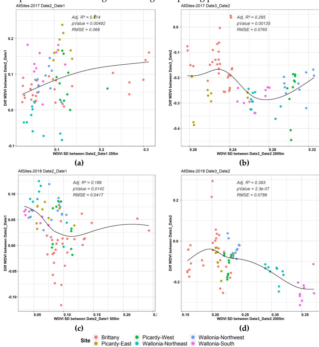
Figure 7-8. The best relationships (i.e. highest adj. R^2 ) between Diff WdVI and WdVI SD for the six study landscapes during the (a, c) stem-extension (Date2_Date1) and (b, d) ripening (Date3_Date2) periods of wheat in (a, b) 2017 and (c, d) 2018.
