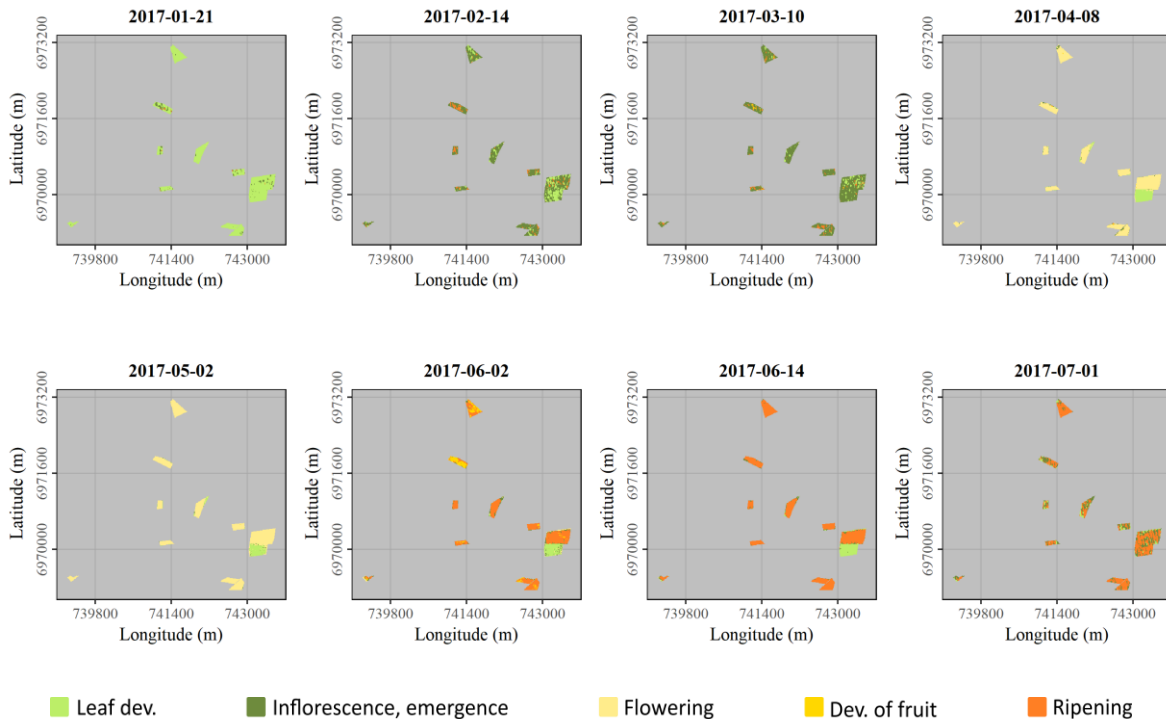
Appendix D-6. Classification of the 5 principal phenological stages of rapeseed in the bocage study site using combined Sentinel-1 & 2 data.
