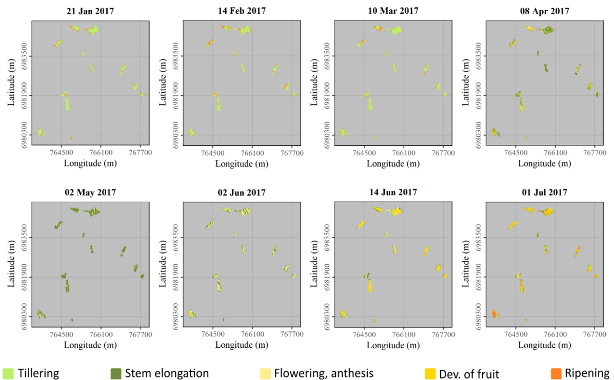
Appendix D-2. Classification of the 5 principal phenological stages of wheat in the bogage study site using combined Sentinel-1 & 2 data.
