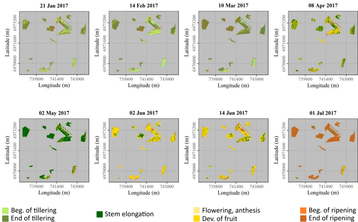
Appendix D-3. Appendix D-3. Classification of the 7 secondary phenological stages of wheat in the open field study site using combined Sentinel-1 & 2 data.
