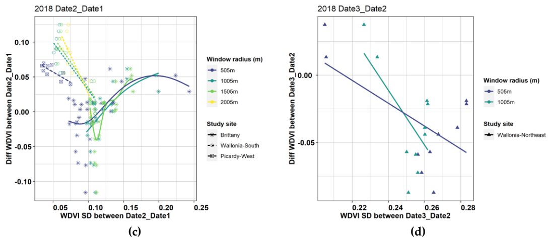
Figure 7-9. Significant relationships between Diff WDV and WDV SD per study area during the (a, c) stem-extension (Date2_Date1) and (b, d) ripening (Date3_2) periods in (a, b) 2017 and (c, d) 2018.
