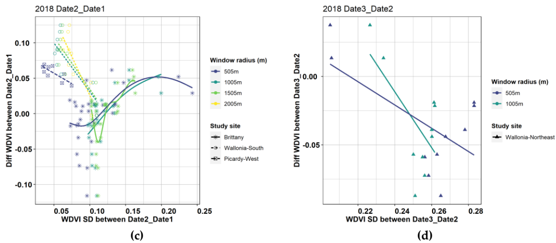
Figure 7-9. Significant relationships between Diff WDVl and WDVl SD per study area during the (a, c) stem-extension (Date2_Date1) and (b, d) ripening (Date3_2) periods in (a, b) 2017 and (c, d) 2018.
