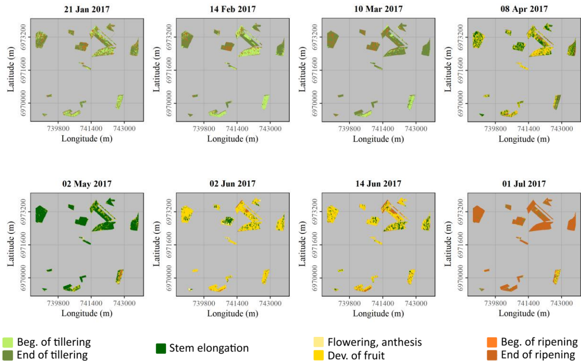
Appendix D-3. Appendix D-3. Classification of the 7 secondary phenological stages of wheat in the open field study site using combined Sentinel-1 & 2 data.
