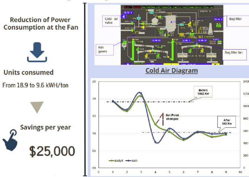
Figure 4.12. Cold Air Diagram during burning operation
