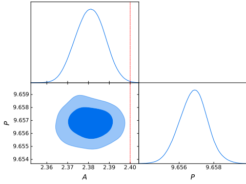
Figure 6.17: Results obtained by running SGWBinner with the MCMC option, starting from 10 initial bins, for data including noise and a broken power law SGWB signal . The SciRD noise model, characterized by 2 parameters ( A, P ), is adopted for the data analysis, while we use the 3 parameters ( A, P, C ) model for the data generation pipeline. Subfigure (a) is the reconstruction plot showing a signal detection. The SGWBinner merges the 10 initial bins into 6 bins. In 5 of the merged bins, the code detects a power law signal for each. For the first bin, the parameter distribution is compatible with the no signal detection. Subfigure (b) presents the marginal probability distributions for the 2 noise parameters, A, P , with the red dashed lines indicating the true values used in the data generation pipeline presented in table 6.1. The red dashed line corresponding to the P parameter is not visible since its true value is out of range of the plot's axes. Subfigure (c) presents the contour plots of the cross correlation between the two parameters of the detected power law signals in every bin.
