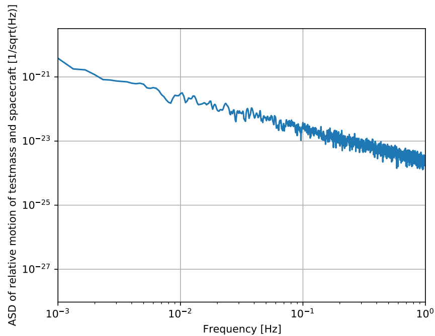
Figure 5.4: Results for fixed MOSAs case with the drag-free axis projection. The data are generated from LISANode simulator, duration of 10^4 seconds, with LISA Dynamics implementation for one spacecraft with a fixed angle between two MOSAs . All quantities are computed in ASD and expressed in fractional frequency deviation units. Two top plots present the motions of the spacecraft w.r.t. inertial Galilean frame (a) and of the test-mass 1 w.r.t. to the containing spacecraft (b). The bottom plot (c) shows the residual relative motion of the test-mass by subtracting the test-mass-to-spacecraft motion to the spacecraft-to-inertial motion.
