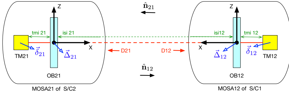
Figure 2.6: Conventions for direction of beams and motions for MOSA 12 and MOSA 21 . Note that the unit vector along x -axis of local reference frame for MOSA 12 is \hat{\mathbf{n}}_{21} , inverse the two indices w.r.t MOSA convention.
