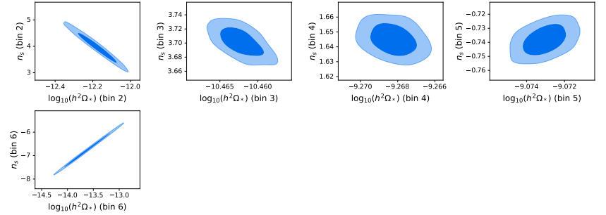
Figure 6.17: Results obtained by running SGWBinner with the MCMC option, starting from 10 initial bins, for data including noise and a broken power law SGWB signal . The SciRD noise model, characterized by 2 parameters ( A, P ), is adopted for the data analysis, while we use the 3 parameters ( A, P, C ) model for the data generation pipeline. Subfigure (a) is the reconstruction plot showing a signal detection. The SGWBinner merges the 10 initial bins into 6 bins. In 5 of the merged bins, the code detects a power law signal for each. For the first bin, the parameter distribution is compatible with the no signal detection. Subfigure (b) presents the marginal probability distributions for the 2 noise parameters, A, P , with the red dashed lines indicating the true values used in the data generation pipeline presented in table 6.1. The red dashed line corresponding to the P parameter is not visible since its true value is out of range of the plot's axes. Subfigure (c) presents the contour plots of the cross correlation between the two parameters of the detected power law signals in every bin.
