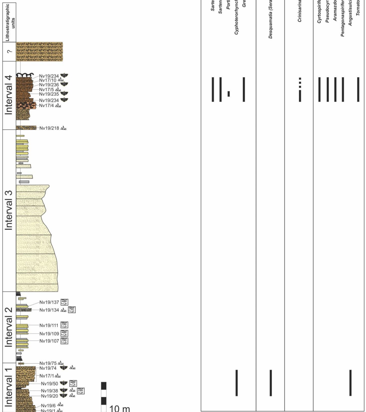
Figure 51. Diversity and stratigraphic distribution of brachiopods of the Noravank section.
