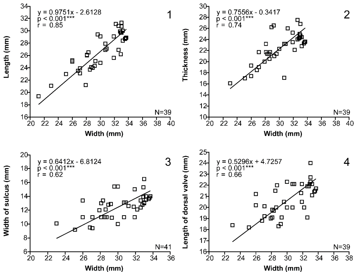
Figure 48. Scatter diagrams of Tornatospirifer armenicus (Abrahamyan, 1974). 1, Relation between shell width and length. 2, Relation between shell width and thickness. 3, Relation between shell width and width of sulcus. 4, Relation between shell width and length of dorsal valve. Abbreviations: N , number of specimens measured; y=ax+b , linear model; r , coefficient of correlation; p^{***} , significant probability value.
