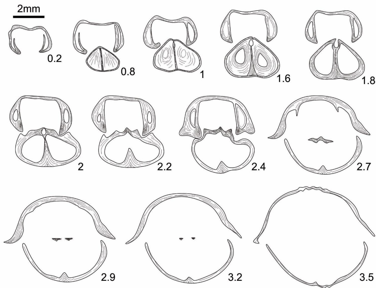
Figure 29. Transverse serial sections of Ripidiorhynchus djravankensis n. sp. (IGSNASRAGM 3928/PS 3034) from the lowest Famennian Noravank Regional Stage, Djravank section. Numbers refer to distances in mm from the tip of the ventral umbo.
