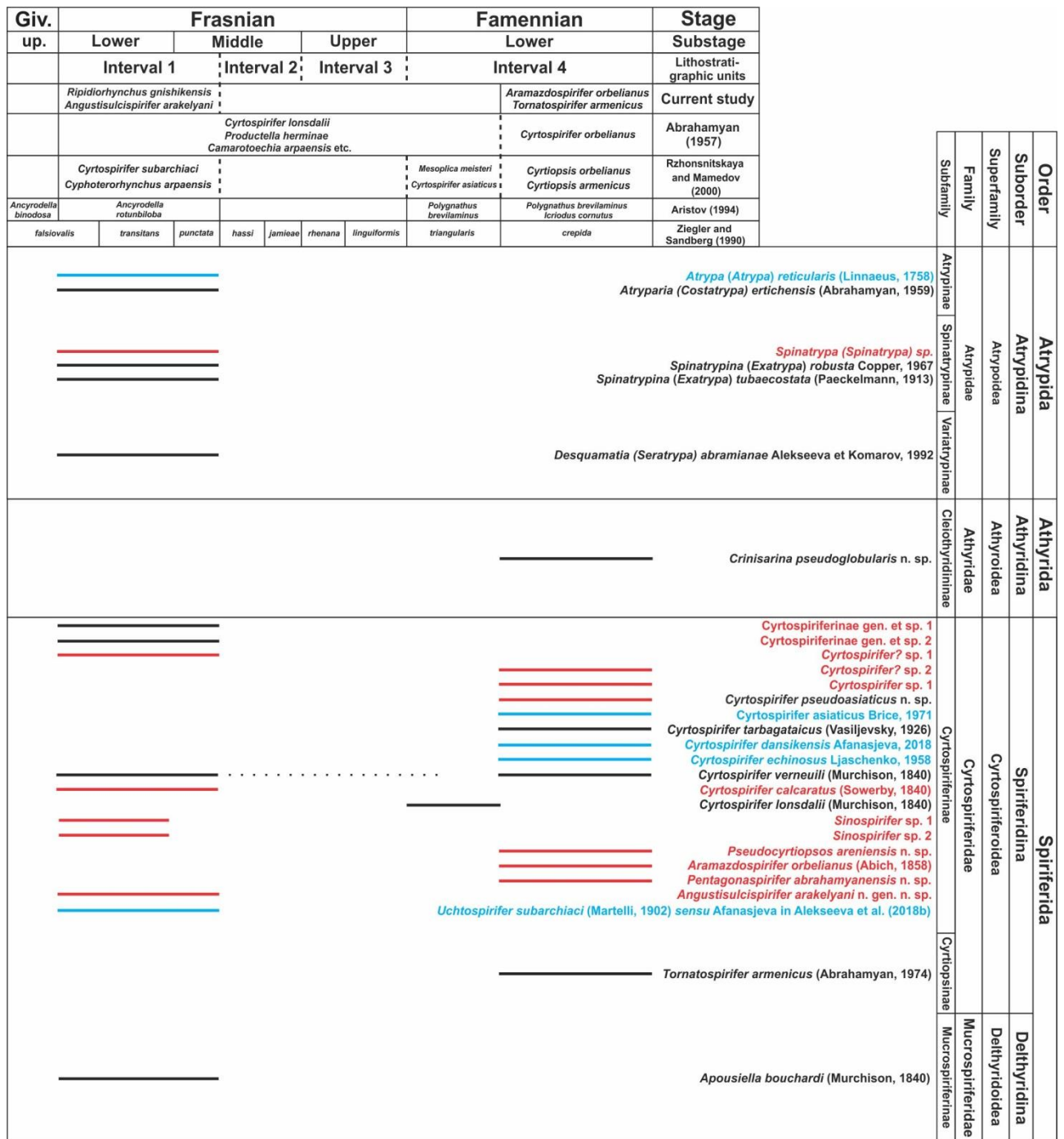
Figure 56. Biostratigraphic distribution of brachiopod species belonging to the orders Atrypida, Athyrida and Spiriferida, reported from the Frasnian–lower Famennian sedimentary sequences in the Lesser Caucasus. Red color indicates species which are known from Armenia based on the data of Abrahamyan (1957, 1974) and Arakelyan (1964); blue color indicates species reported from Nakhichevan (Alekseeva et al., 2018a, b); black color points those species that are known both from Armenia and Nakhichevan.
