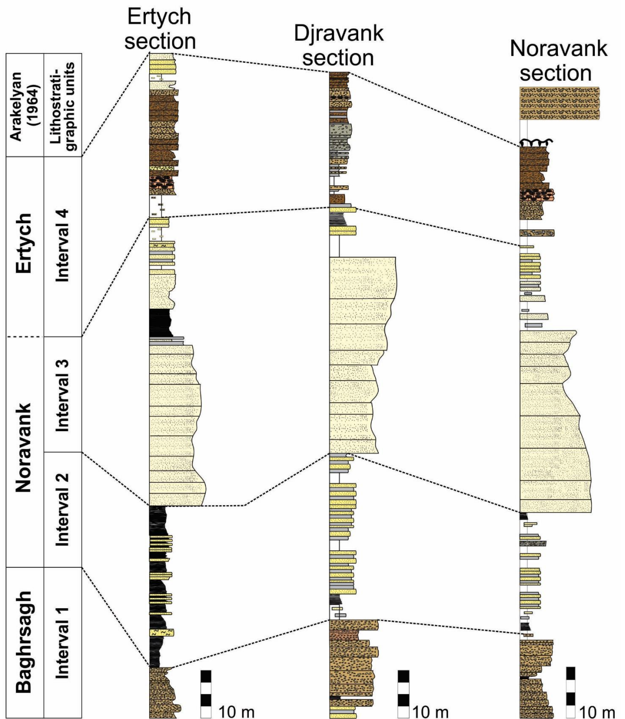
Figure 26. Lateral correlation between the three studied sections.
