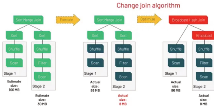
Figure 4.8 Adaptive query execution [4]
