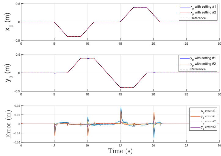
Figure 4.23: x_p and y_p trajectories tracking and error with \mathcal{H}_\infty control with with our two four-bloc synthesis
