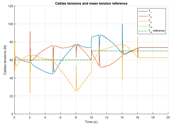
Figure 4.13: Cables tensions and mean tension reference
