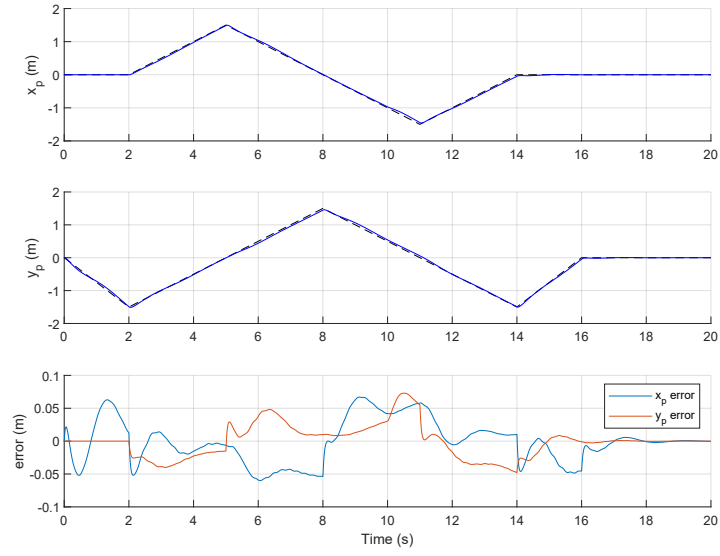
Figure 4.12: x_p and y_p trajectories tracking and error with \mathcal{H}_\infty control
