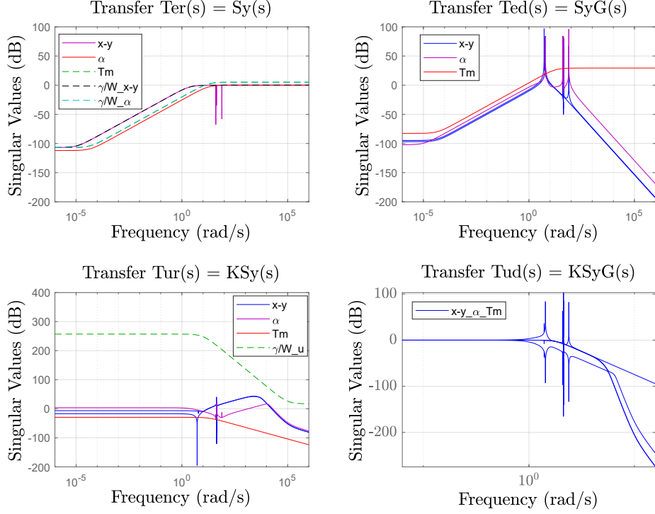
Figure 4.16: Closed-loop transfers (plain) and the corresponding templates (dashed) with two-block synthesis scheme
