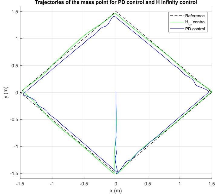
Figure 4.14: Trajectories of the mass point for PD control and \mathcal{H}_\infty control
