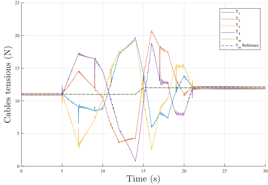
Figure 4.26: Cables tensions and mean tension reference with the second synthesis
