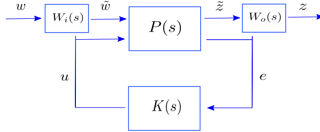
Figure 4.3: Standard \mathcal{H}_\infty synthesis scheme with introduction of weighting functions
