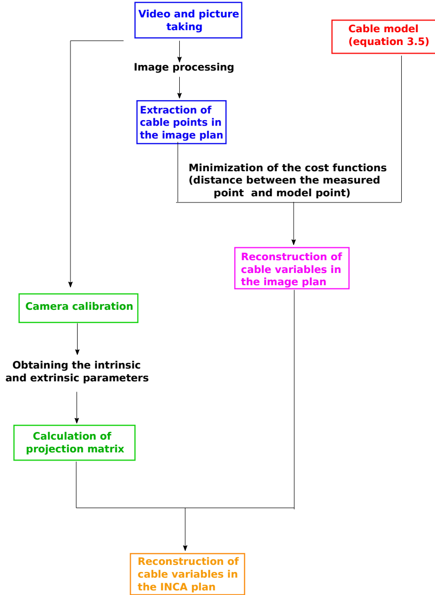
Figure 3.7: Steps of the algorithm of model geometric validation.
