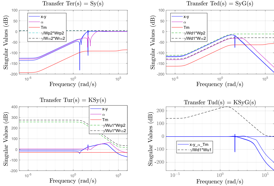
Figure 4.19: Closed-loop transfers (plain) and the corresponding templates (dashed) with four-block synthesis with setting #2
