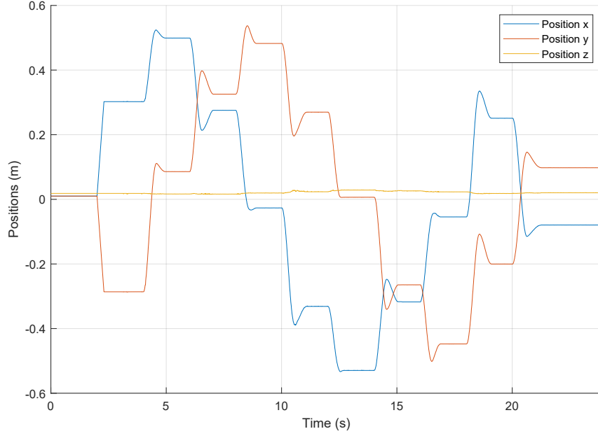
Figure 2.7: Open-loop trajectories of the platform positions ( x - y - z ).
