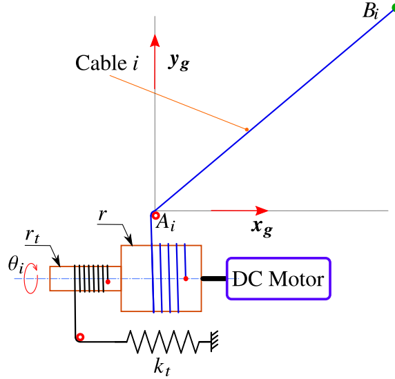
Figure 2.10: Working principle of a transmission unit for straight-line segment cable i .
