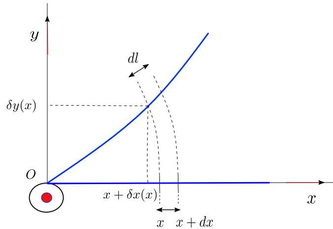
Figure A.1: Cable displacement
