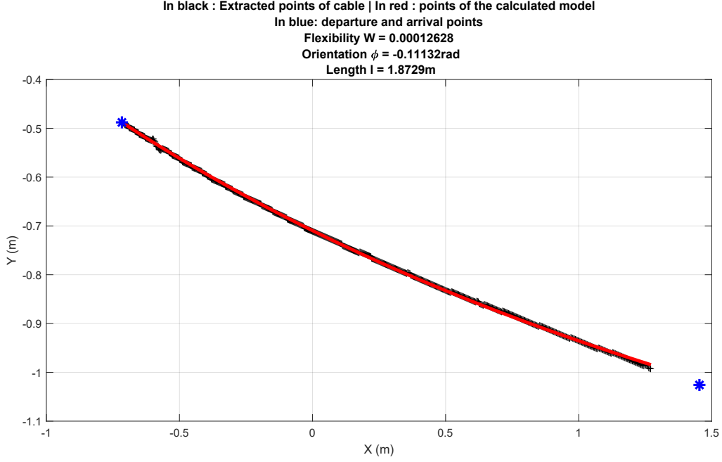
Figure 3.12: The validation of the geometric model of flexible cable from the video stream.
