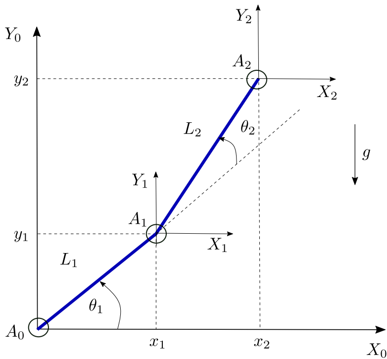
Figure A.4: Double pendulum system
