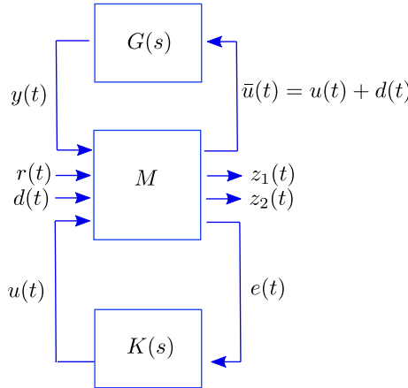
Figure 4.5: The interconnection for the \mathcal{H}_\infty synthesis
