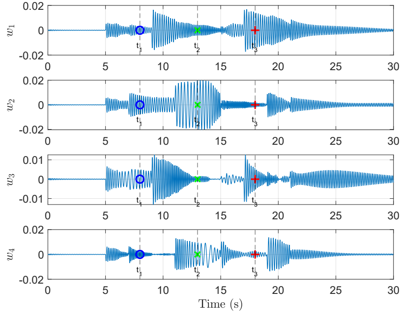
Figure 4.25: Modal coordinates for the flexibility of the cables with the second synthesis
