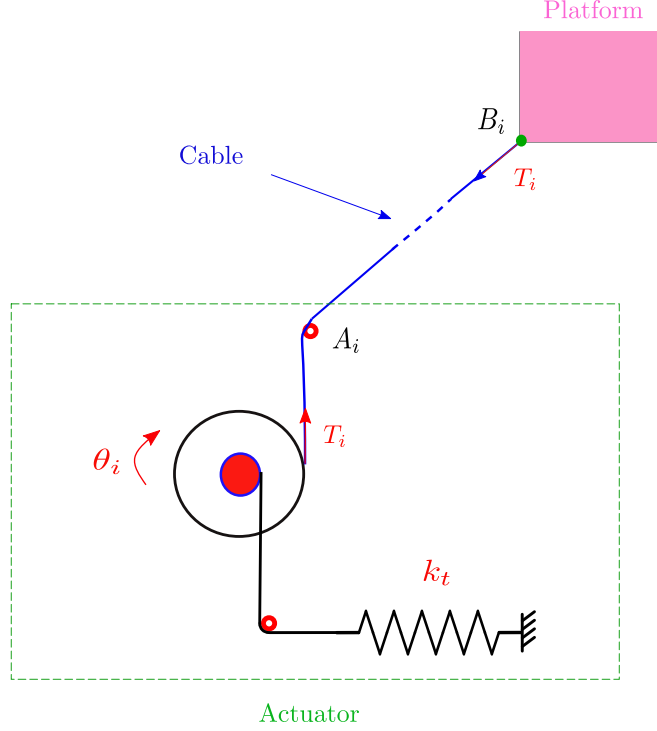
Figure 2.11: A global dynamic diagram of a 3 DOFs CDPR.
