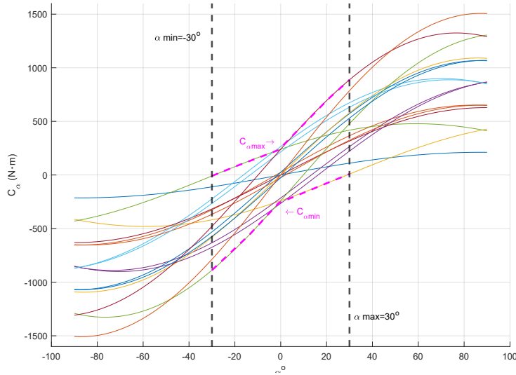
Figure 2.13: The external torque c_\alpha for different values of \alpha for geometry (2).
