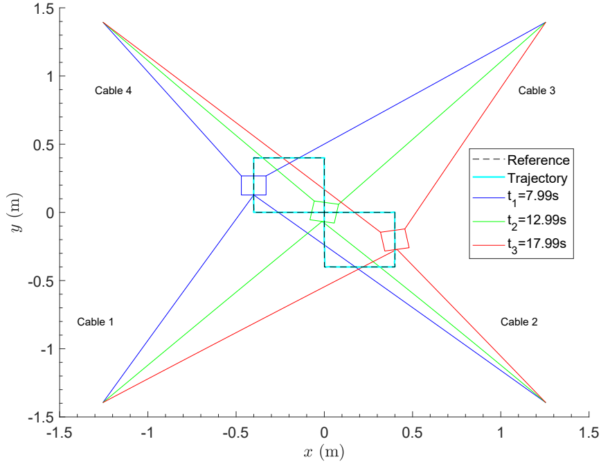
Figure 4.24: Trajectories of the platform and cables in the x-y plan with the second synthesis
