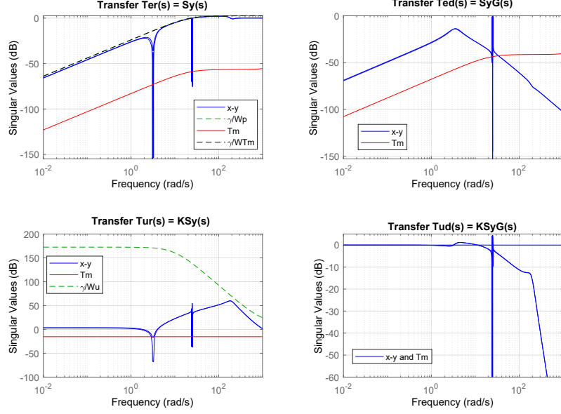
Figure 4.9: Closed-loop transfers (plain) and the corresponding templates (dashed)
