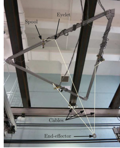
(c) The Laval university prototype (Gosselin (2013))
