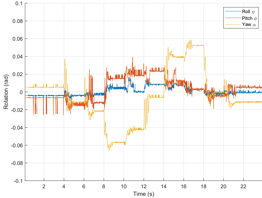
Figure 2.8: Open-loop trajectories of the platform orientations about axis ( x - y - z ).
