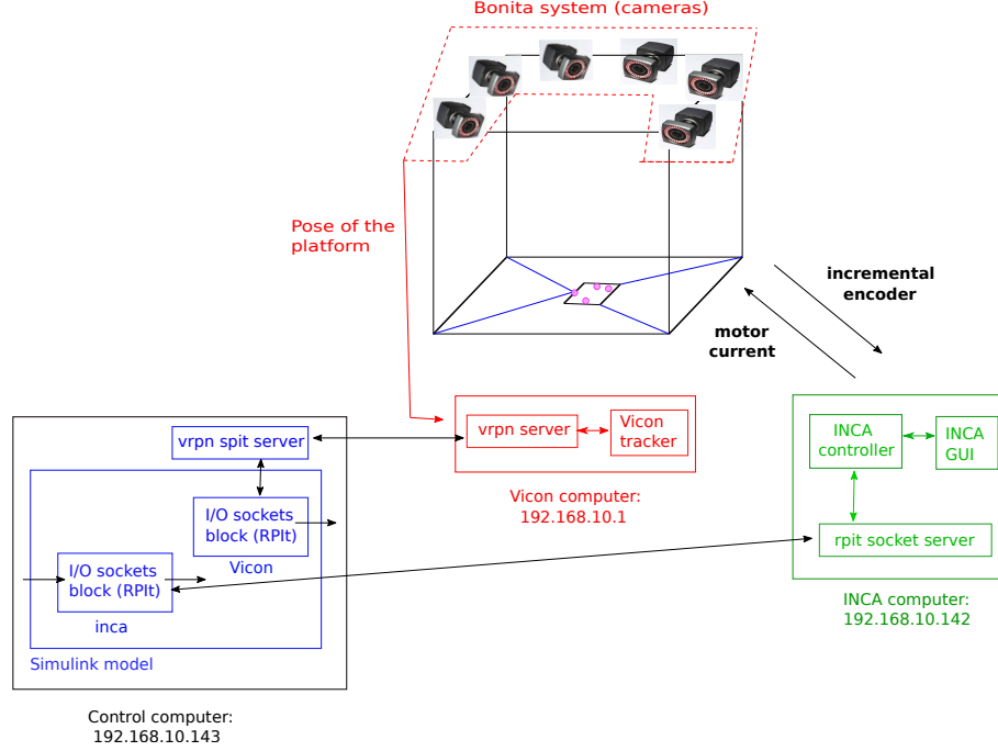
Figure 2.4: Real-time control architecture of the INCA.
