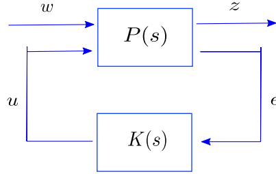
Figure 4.2: Standard scheme of the \mathcal{H}_\infty synthesis
