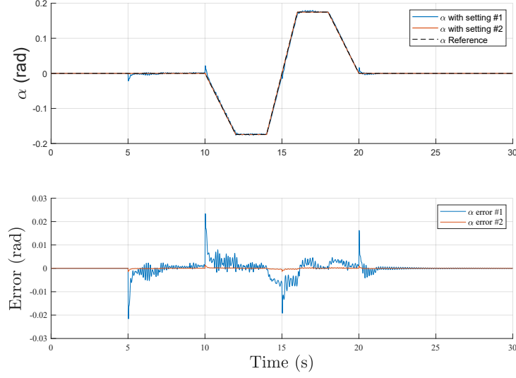
Figure 4.22: Orientation trajectory of the platform for \mathcal{H}_\infty control with our two four-bloc synthesis
