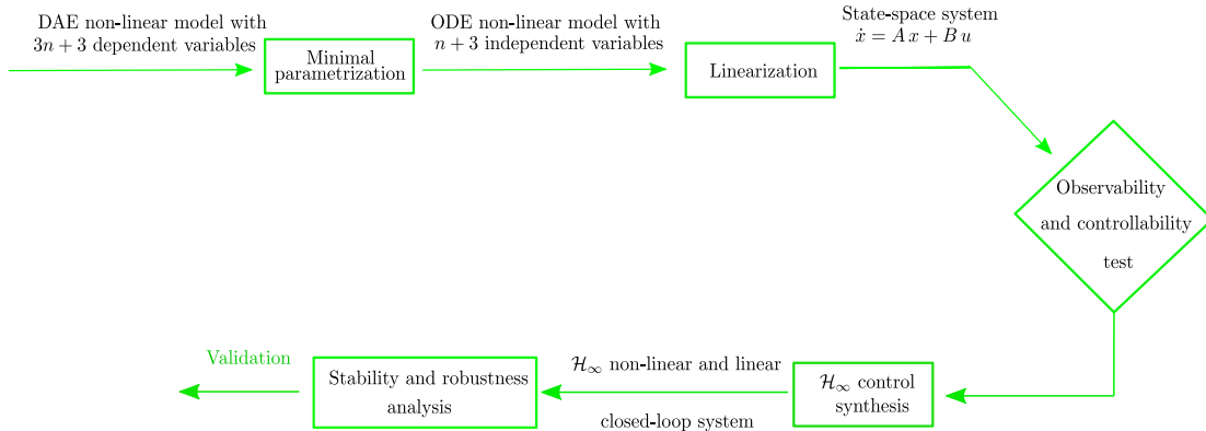
Figure 3.6: Control and linearization methodology for the ODE model.
