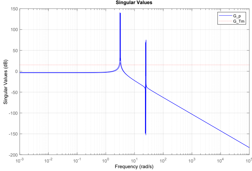
Figure 4.7: Frequency behavior of the open-loop nominal system
