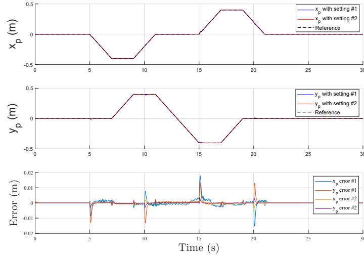
Figure 4.23: x_p and y_p trajectories tracking and error with \mathcal{H}_\infty control with our two four-bloc synthesis
