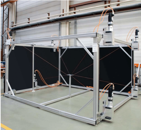
(a) IPAnema robot (Pott et al. (2013))
