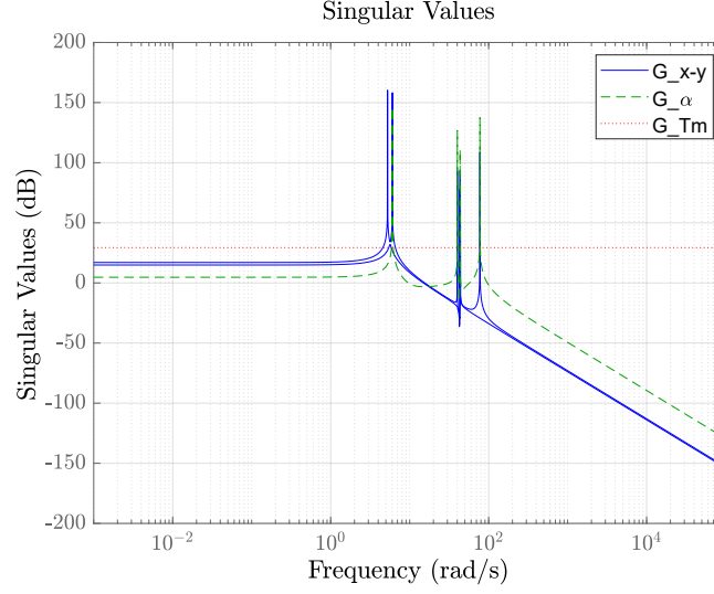
Figure 4.15: Open-loop frequency response of the linear system
