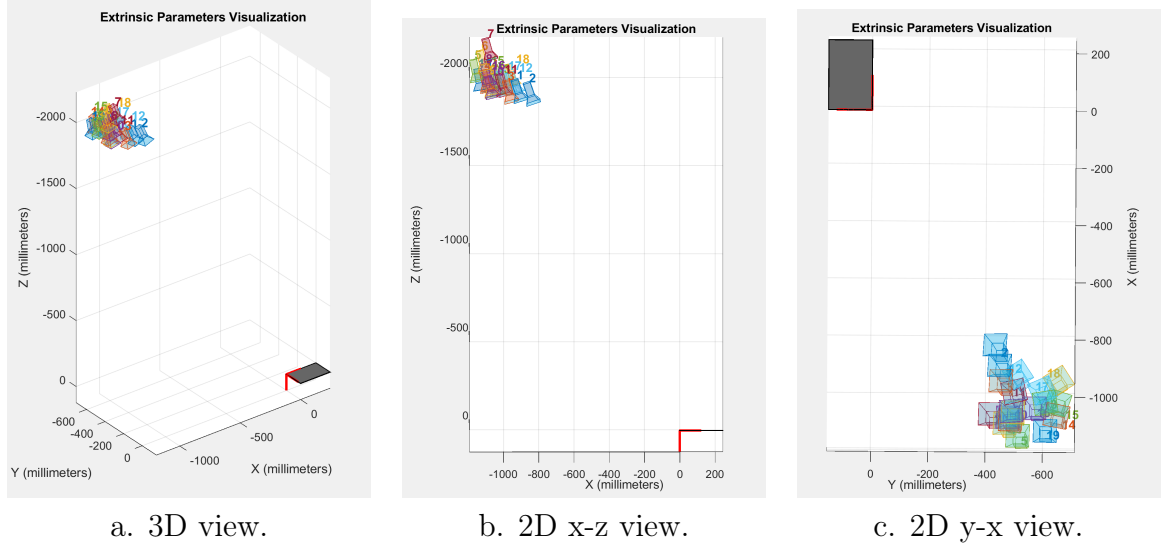
Figure 3.11: 3D representation of the position of our mobile camera in relation to the different views of the fixed calibration pattern.
