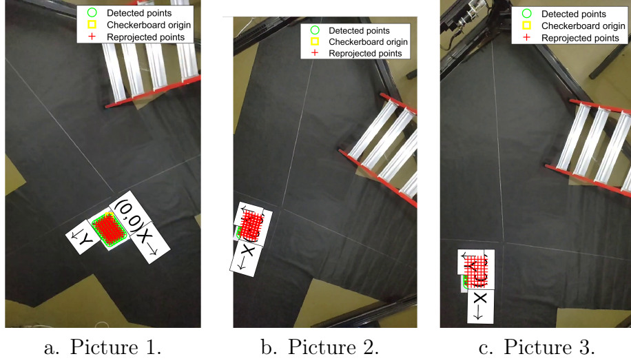
Figure 3.10: Set of pictures used for the calibration.
