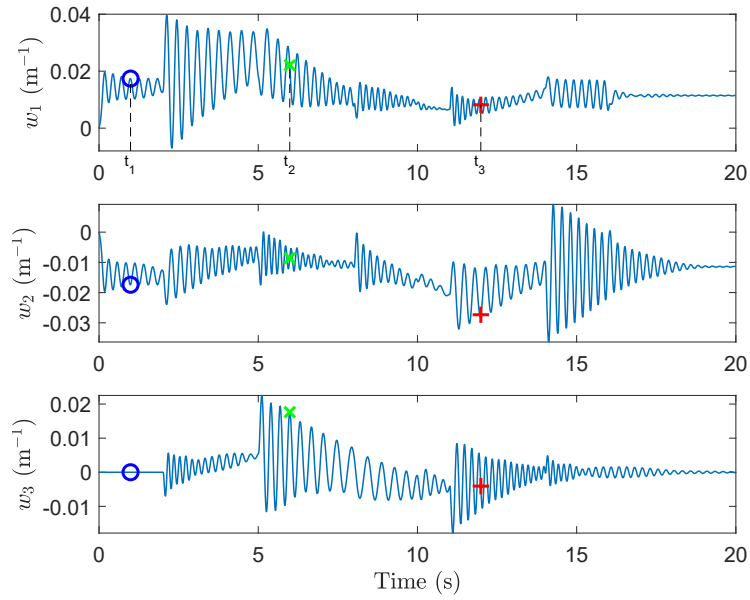
Figure 4.11: Modal coordinates for the displacements of the cables
