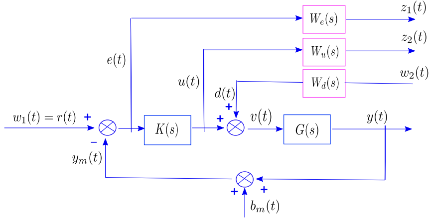
Figure 4.4: Four-block standard \mathcal{H}_\infty synthesis scheme with weighting functions
