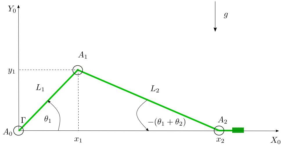
Figure A.3: Slider-Crank Mechanism
