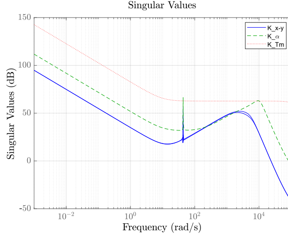
Figure 4.20: Frequency response of the controller
