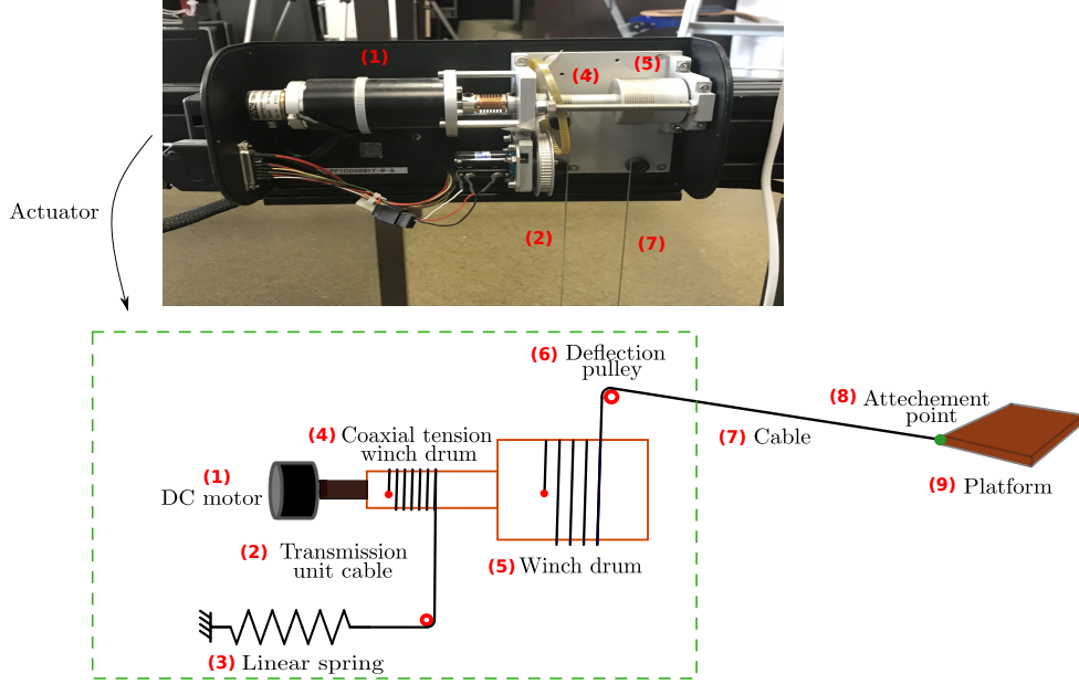
Figure 2.3: Actuator scheme of the INCA robot prototype.
