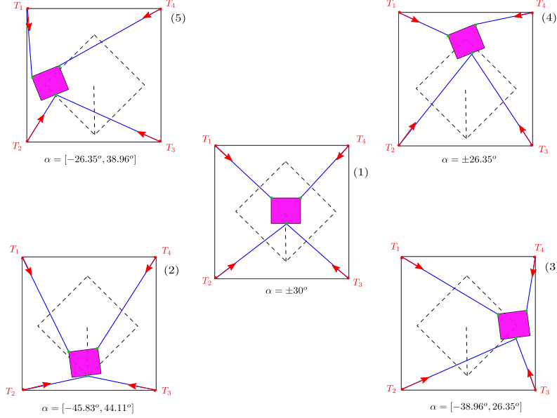
Figure 2.14: The platform's possible orientation in different locations in the workspace.
