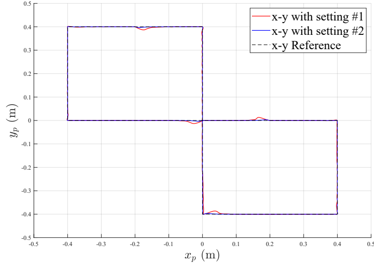
Figure 4.21: Translation trajectories of the platform for \mathcal{H}_\infty control with our two four-bloc synthesis
