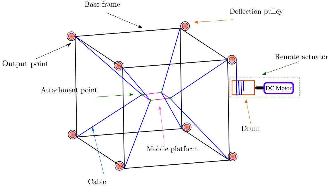
Figure 1.3: Elements of cable-driven parallel robot.
