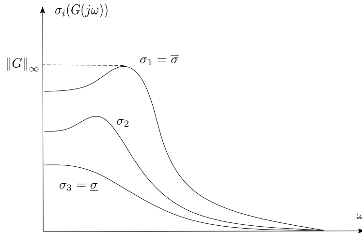
Figure B.1: Singular values and \mathcal{H}_\infty -norm of a transfer matrix (Toscano (2013))
