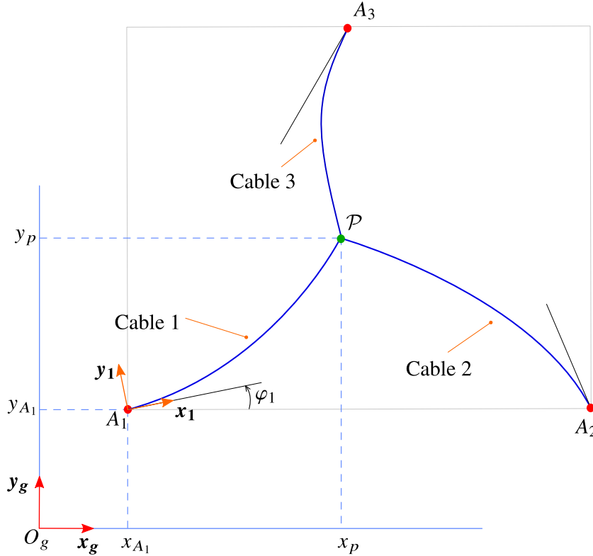
Figure 4.6: Schematic representation of a planar three flexible cable robot.
