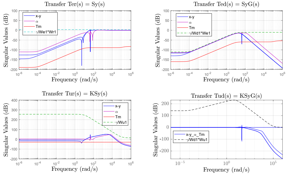
Figure 4.18: Closed-loop transfers (plain) and the corresponding templates (dashed) with four-block synthesis with setting #1
