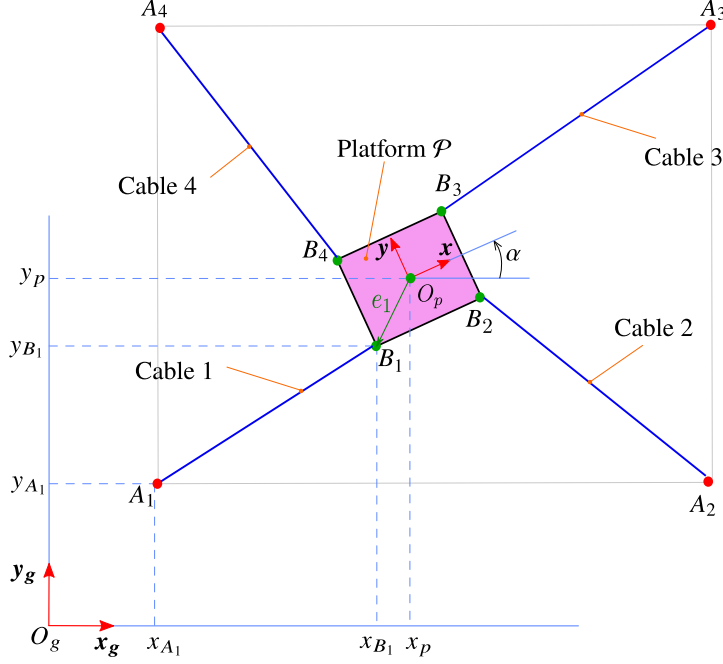
Figure 2.9: Schematic representation of a planar four straight-line segment cable robot.
