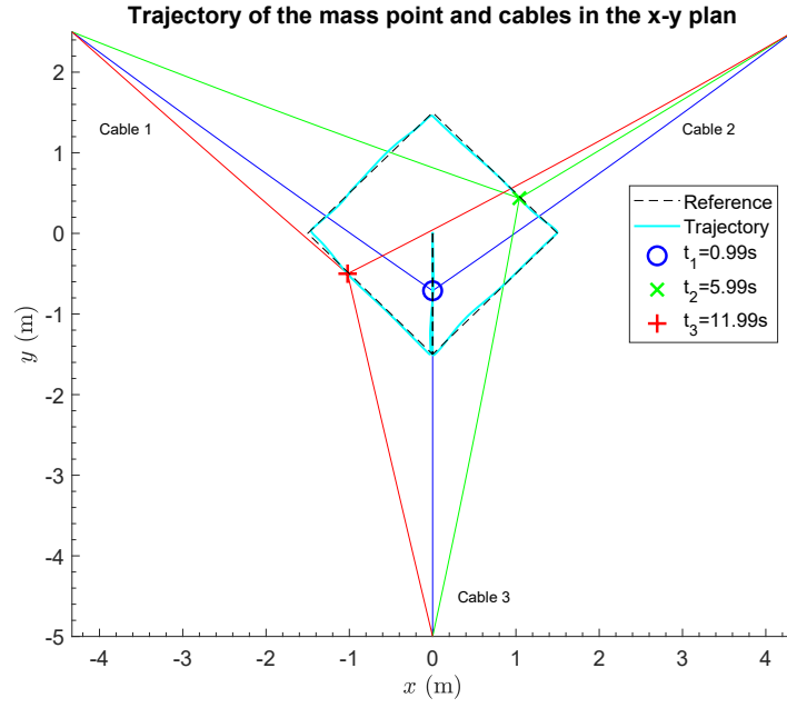
Figure 4.10: Trajectory of the mass point and cables in the x - y plan
