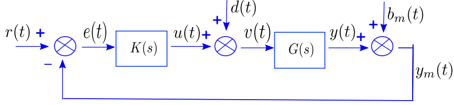
Figure 4.1: Standard control feedback scheme
