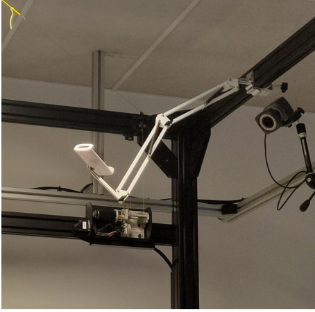
(a) The camera stand.
