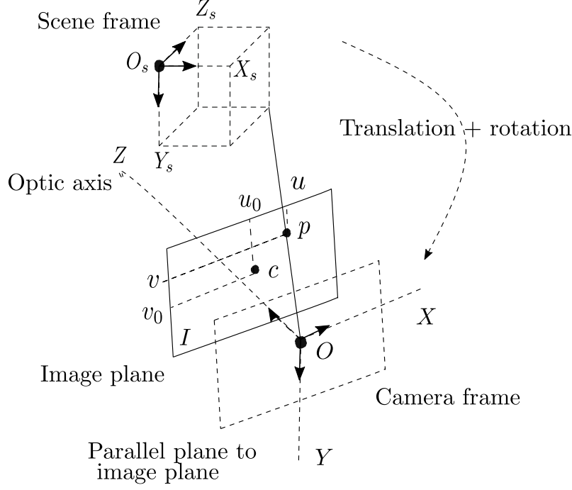
Figure A.5: Pinhole model Habed (2022)
