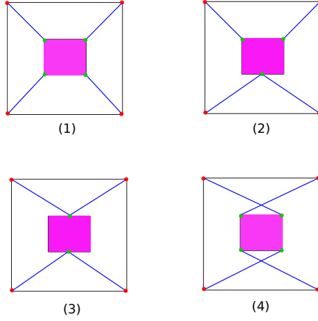
Figure 2.12: Different scenarios for different cable attachment points locations.
