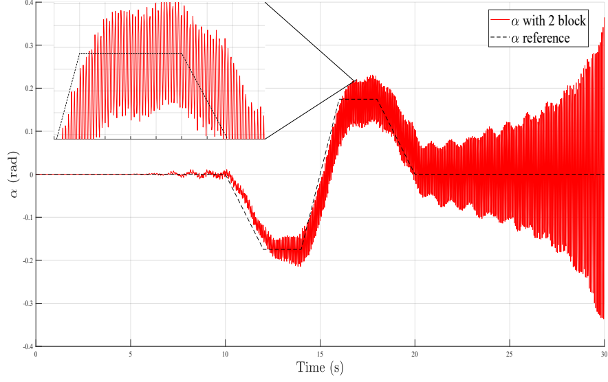
Figure 4.17: Orientation trajectories with two-block synthesis scheme
