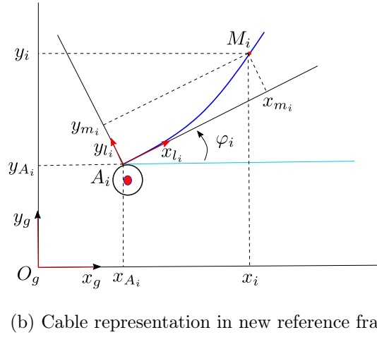
Figure 3.3: Displacement of the flexible cable.
