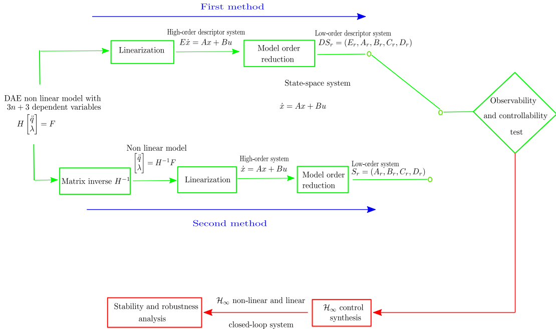
Figure 3.4: Control and linearization methodology for the DAE model.
