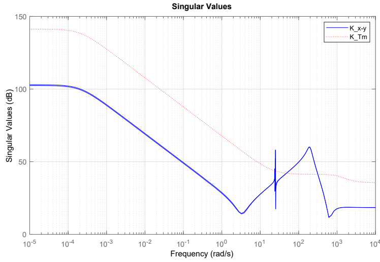
Figure 4.8: Frequency behavior of the controller
