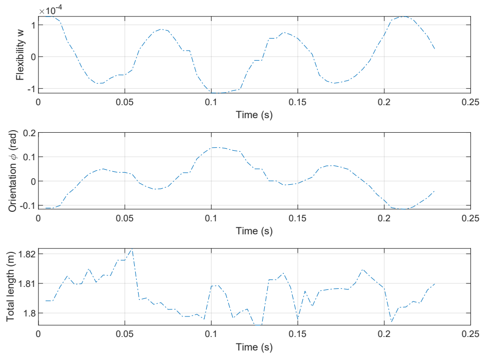
Figure 3.13: The time evolution of the estimated cable's variables (l, \varphi, w)
