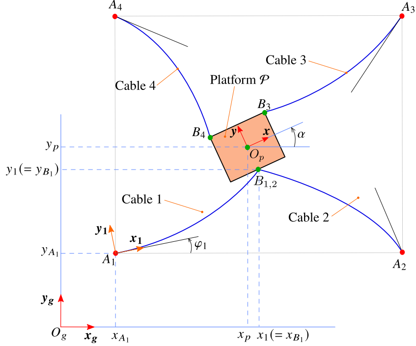
Figure 3.2: Schematic representation of a planar four flexible cable robot.
