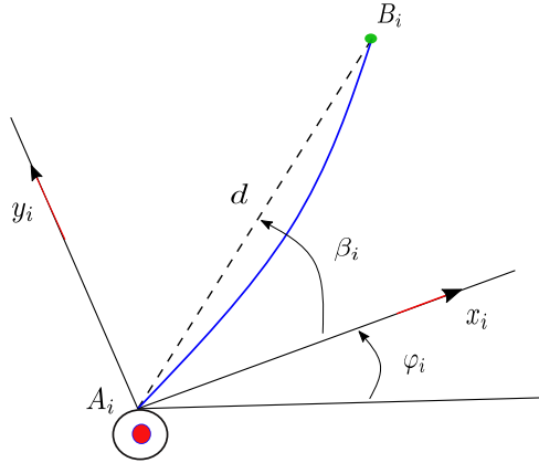
Figure 3.5: Geometry of the cable \#i .
