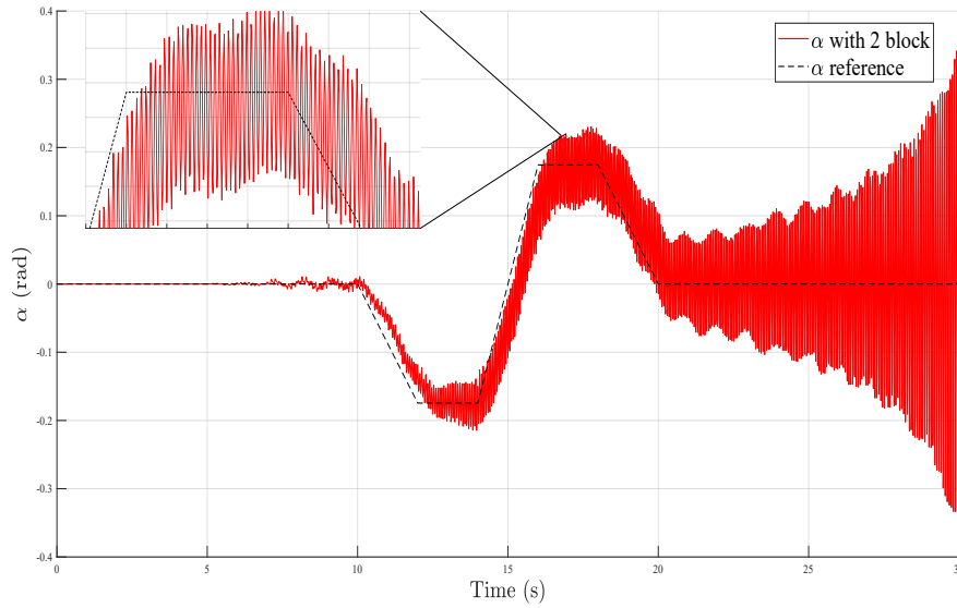
Figure 4.17: Orientation trajectories with two-block synthesis scheme
