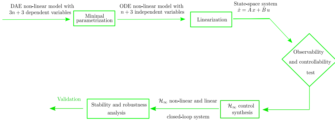
Figure 3.6: Control and linearization methodology for the ODE model.
