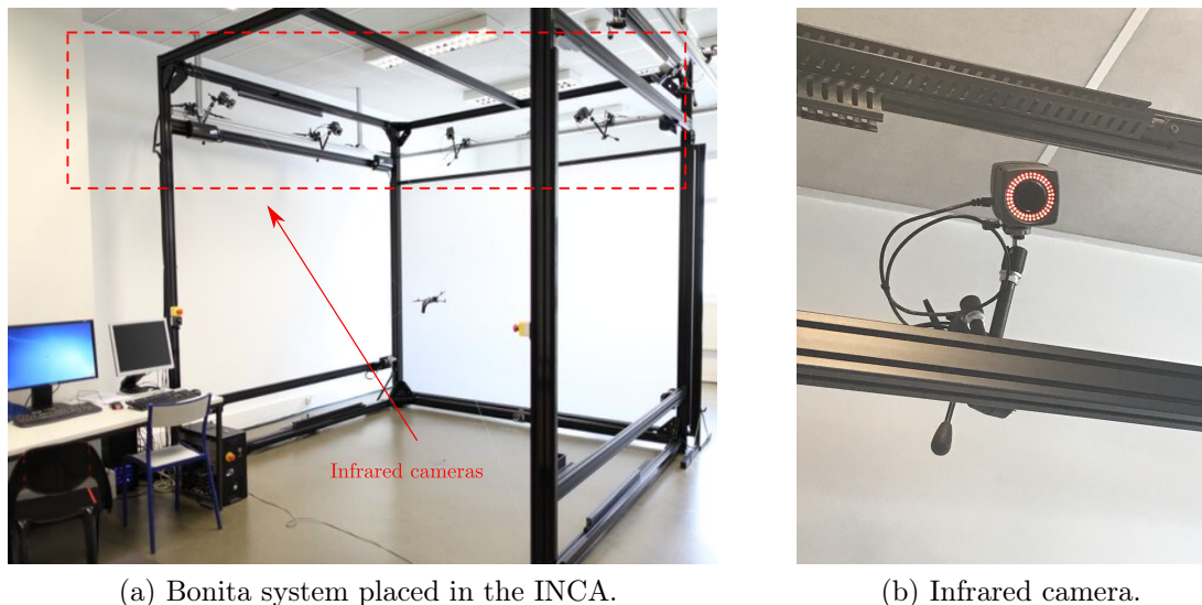
Figure 2.5: Bonita motion capture system.
