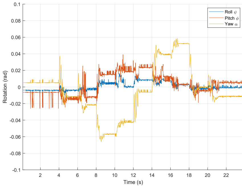
Figure 2.8: Open-loop trajectories of the platform orientations about axis ( x - y - z ).
