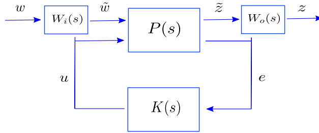
Figure 4.3: Standard \mathcal{H}_\infty synthesis scheme with introduction of weighting functions
