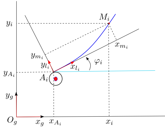
Figure 3.3: Displacement of the flexible cable.
