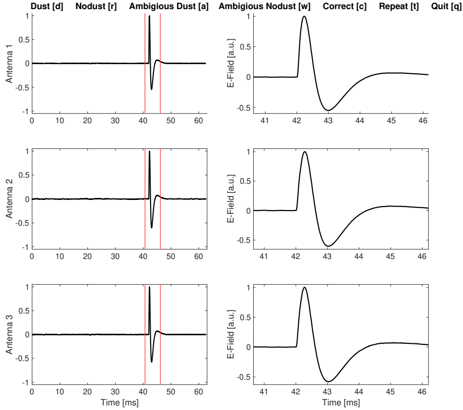
Figure A1. The manual labeling user interface showing a signal observed December 19, 2020. The left column displays the full snapshot (from 0 to \sim 63 ms) at all antennas. An area of interest is selected by adjusting the red vertical lines. The right column displays the signal within the area of interest. The signal can be labeled as dust by pressing the [d] key on the keyboard and no dust by pressing the [r] key. The signal is indicated to be ambiguous if the waveform do not fit clearly into either of the two labels, note however that signals indicated to be ambiguous were also labeled into either dust or no dust using the [a] and [w] keys. There is also an option to correct [c] the previously labeled signal (in case of an error), repeat [t] the area of interest selection and quit [q] the manual labeling user interface.
