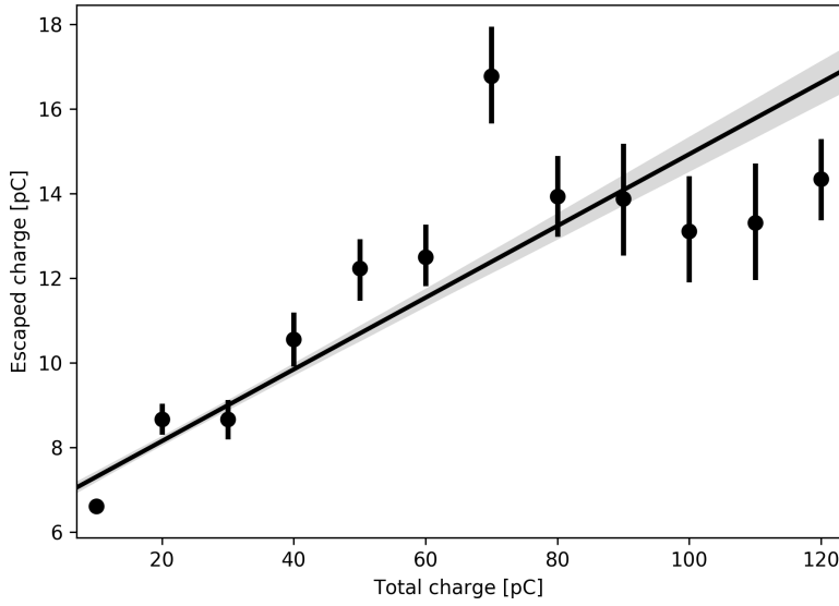
Figure 15: Escaping charge, \epsilon Q , as a function of the total charge released in the cloud, Q . The points show the average of the values of \epsilon Q per bins of values of Q . The binwidth is 10 pC. The error bars show the standard deviation of the distribution of \epsilon Q in each bin.
