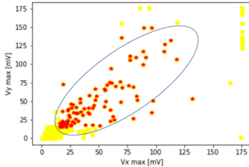
Figure 9: Maximum signal amplitude recorded on X and Y monopoles in the period from 2008 October 1 to 2008 December 31. Red stars represent only the dust signal.
