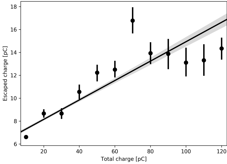
Figure 15: Escaping charge, \epsilon Q , as a function of the total charge released in the cloud, Q . The points show the average of the values of \epsilon Q per bins of values of Q . The binwidth is 10 pC. The error bars show the standard deviation of the distribution of \epsilon Q in each bin.
