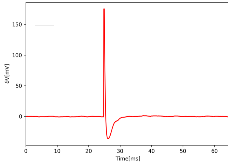
Figure 8: An example of a voltage impulse recognized as dust impact detected by the TDS on-board STEREO.
