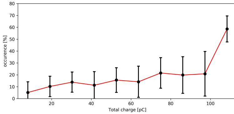
Figure 16: Histogram of the occurrence of events with precursor amplitude larger than 5mV with respect to the total charge amount. The error bars show the standard deviation of the distribution. The binwidth is 12 pC.
