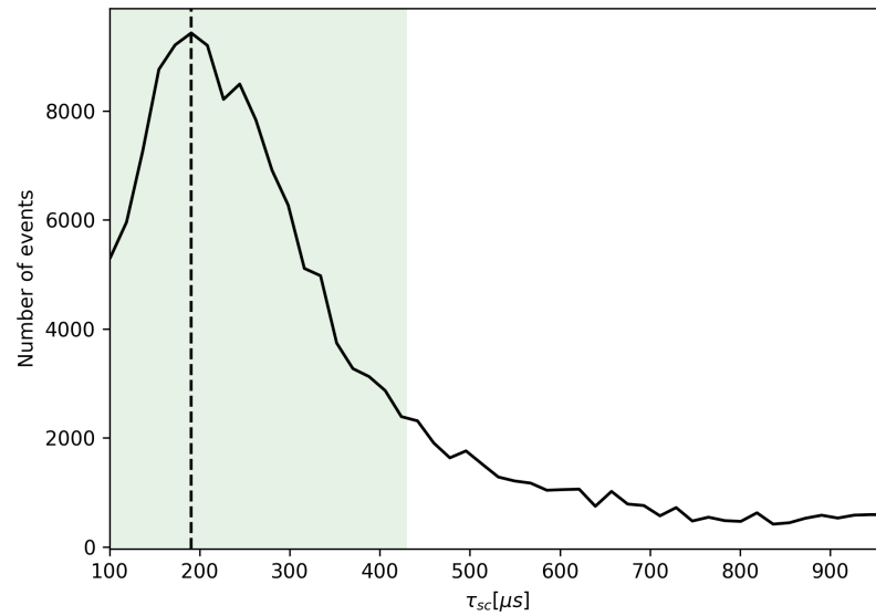
Figure 12: Histogram of the parameter \tau_{sc} . The green section on the histogram indicates the extreme values of the parameter calculated from Eq. (19) (see text for details). Around 80% of the obtained values for \tau_{sc} are inside the green section. The dashed vertical line represents the most probable obtained value for the parameter, \tau_{sc} \sim 190 \mu\text{s} . The median value of the distribution is 270 \mu\text{s} .
