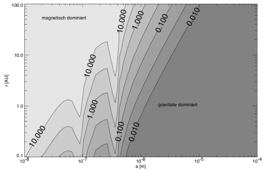
Figure 19: For several particle sizes and different distances from the Sun, the Lorentz force is compared with "effective gravitation".
