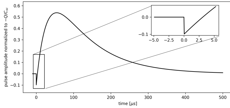
Figure 7: Simulation of the signal shape through proposed models for the effect on the spacecraft potential of a transient dust impact. The curve is obtained from the simple model, assuming the electron collection (escape) to be instantaneous, \tau_e \approx 0 (Eq. 25). The ratio between escaped charge and total charge is \epsilon = 0.1 , and timescales parameters are \tau_{sc} = 100\mu s and \tau_{ion} = 30\mu s . The zoomed-in portion of the plot (top right) provides an insight into the pre-shoot signal shape.
