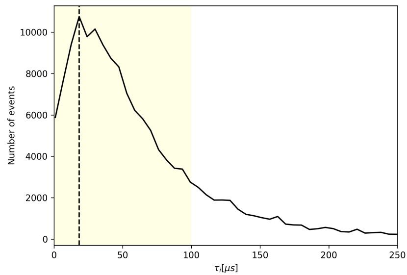
Figure 13: Histogram of the parameter \tau_i . The yellow section includes all the obtained values below 100 \mu s (the threshold for the \tau_{sc} ). More than 80% of the obtained \tau_i is inside the yellow section. The vertical dashed line represents the most probable obtained value for the parameter, \tau_i \sim 18 \mu s .
