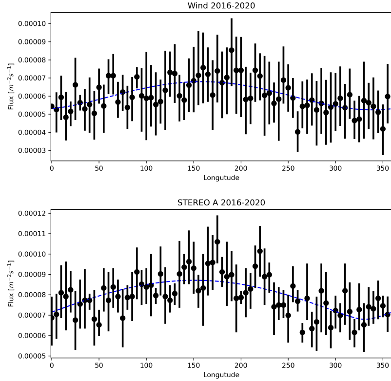
Figure 23: The averaged flux measured over five years (2016-2020) on the WIND (top) and STEREO A (bottom), respectively and the corresponding error bars as a function of the probes' ecliptic longitude. The averaging is performed on 5 degrees bins and the error bars show the standard deviation of the distribution. The blue curve is the result of the fitting model as described in the text.
