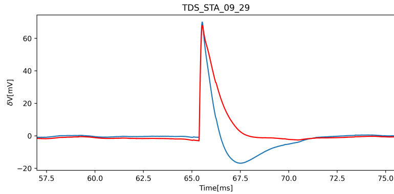
Figure 11: Effect of calibration; the blue line represents raw data, and the red line is the signal after calibration.
