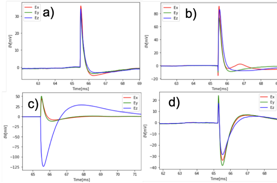
Figure 10: Main categories of dust impact signal obtained by S/WAVES/TDS:
