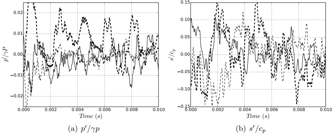
Figure 6.25: a) Dimensionless pressure fluctuations and b) dimensionless entropy fluctuations within the flame tube (last plane of the region \mathbf{P} in Fig. 6.24) for low power (- -), intermediate power (-) and high power conditions (- .-).
