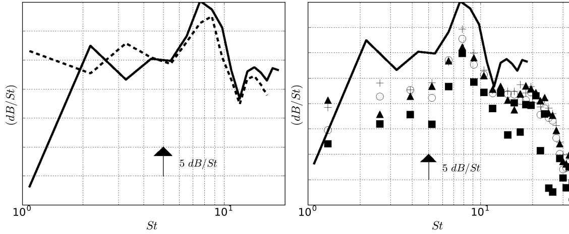
Figure A.8: PSD of a pressure probe localized at 4 D_s in the jet axis. AVSP-f results with a velocity condition (- -) and with a pressure condition (-). LES results with K_{sec} = 1000 ( \blacktriangle ), K_{sec} = 225000 ( \circ ), K_{sec} = 1550000 ( \blacksquare ) and K_{sec} = 1550000 with K_{prim} = 100 ( + ).
