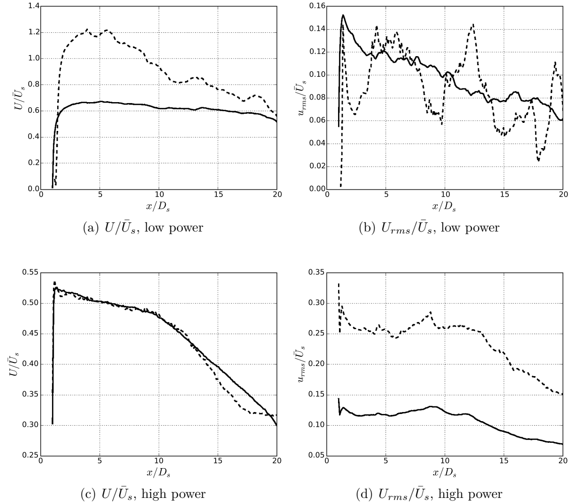
Figure 8.19: Profiles of the axial velocity U/\bar{U}_s and the axial fluctuating velocity U_{rms}/\bar{U}_s on the lip-line of the secondary stream (Fig. 8.2). With M_1 grid (—) and M_2 grid (---).
