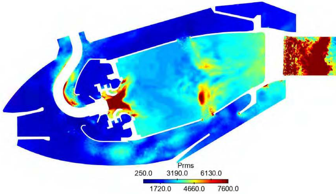
Figure 6.13: Root-mean-squared pressure (Pa) at intermediate power
