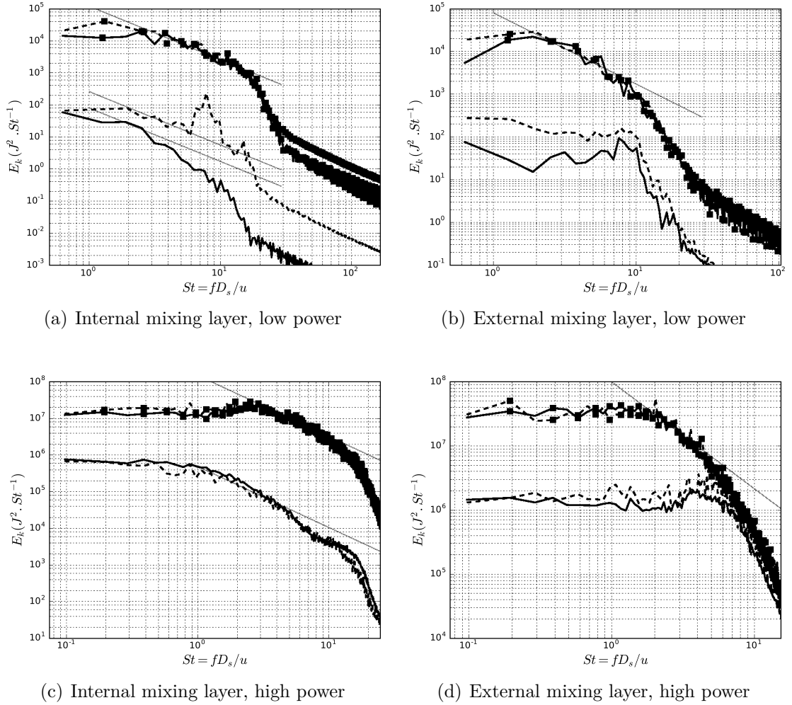
Figure 8.45: PSD of the kinetic energy k . With M_1 grid, jet simulation without combustion noise forcing (—) and with combustion noise forcing (---). At the lips of the primary ( P_1 in Fig. 8.2, internal mixing layer) and secondary ( S_1 , external mixing layer) nozzles (no symbol). At 2 D_s of the primary nozzle exit ( P_2 in Fig. 8.2) in the internal mixing layer and at 0.45 D_s of the secondary nozzle exit ( S_2 ) in the external mixing layer (■). -5/3 power law (---).
