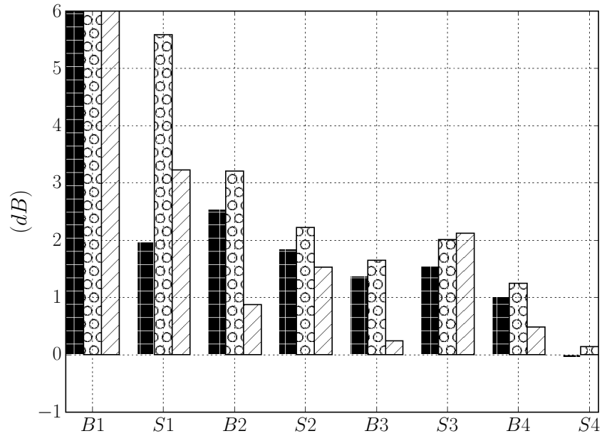
Figure 6.57: Acoustic power losses across the turbines, for low power (■), intermediate power (○) and high power conditions (/ /).
