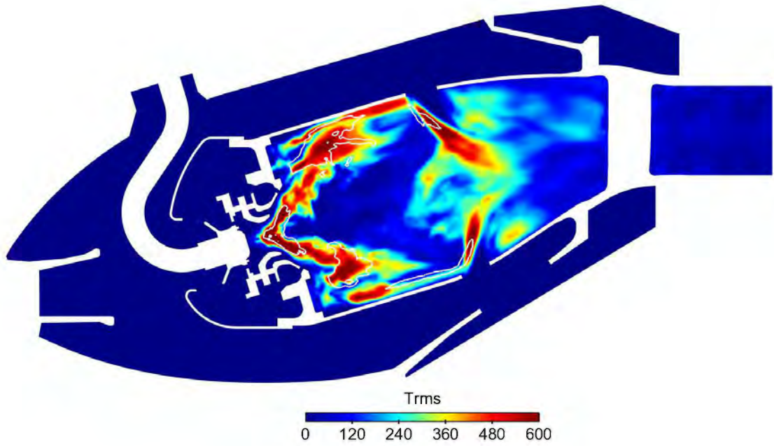
Figure 6.15: Root-mean-squared temperature (K) with white isoline of mean heat release rate ( \text{W}/\text{m}^3 ) at low power
