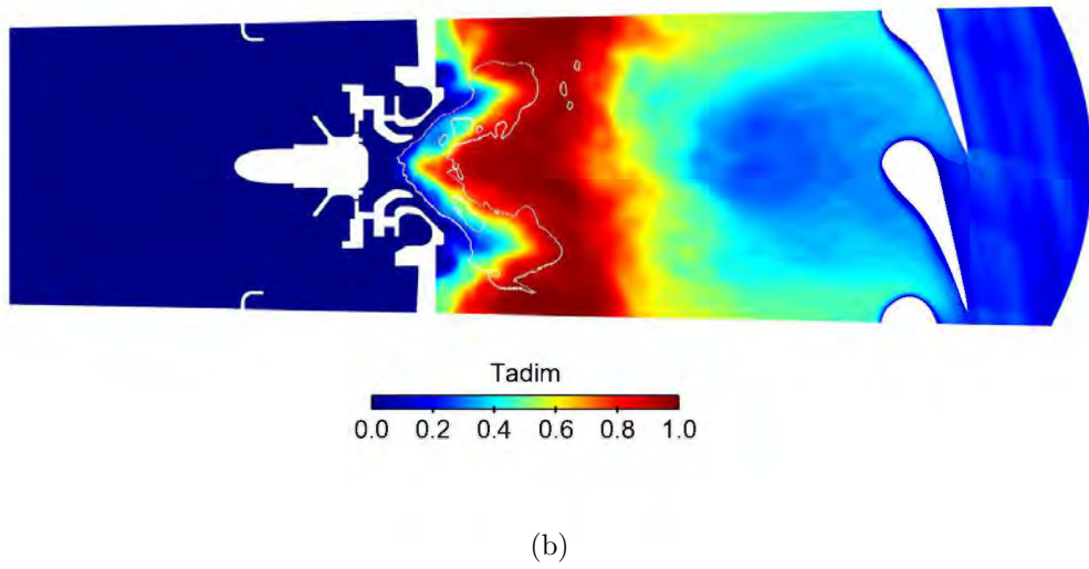
Figure 6.7: Mean dimensionless temperature field \frac{T - T_{inlet}}{T_{max} - T_{inlet}} with white isolines of mean heat release rate ( W/m^3 ) at intermediate power. a) Longitudinal plane at \vec{z} = 0 , b) longitudinal plane parallel to the swirler axis.
