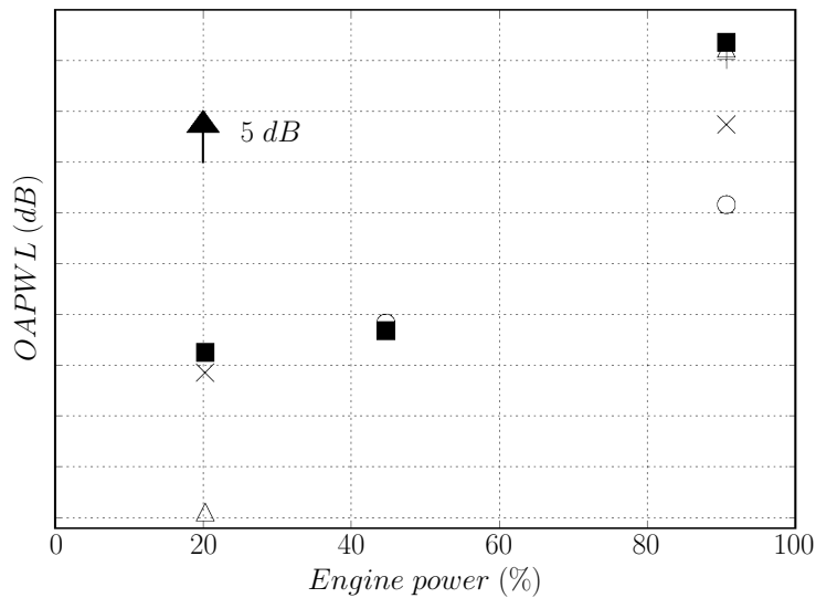
Figure 8.48: Over All Power Level (OAPWL) in far field (45.72 m). CONOCHAIN combustion noise (○), jet noise with M_1 ( \Delta ) and with M_2 (+), jet noise and combustion noise from M1FL and M1FH in Table 8.3 ( \times ), experimental OAPWL of downstream engine noise (■).
