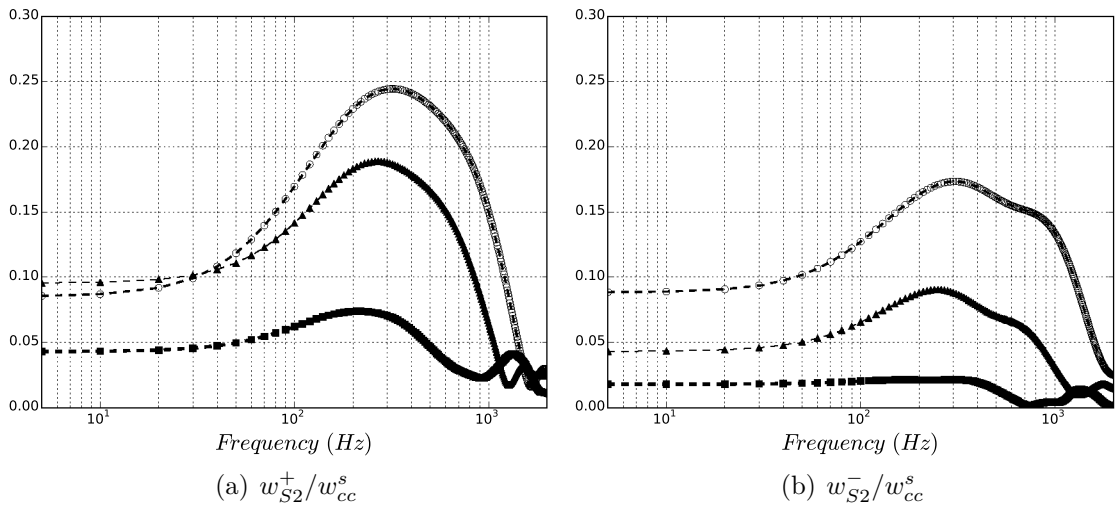
Figure 6.41: Analytical entropy-to-acoustic transfer functions (Eq. 2.75) at position S2 in Fig. 5.4, for low power ( \blacksquare ), intermediate power ( \blacktriangle ) and high power conditions ( \circ ).
