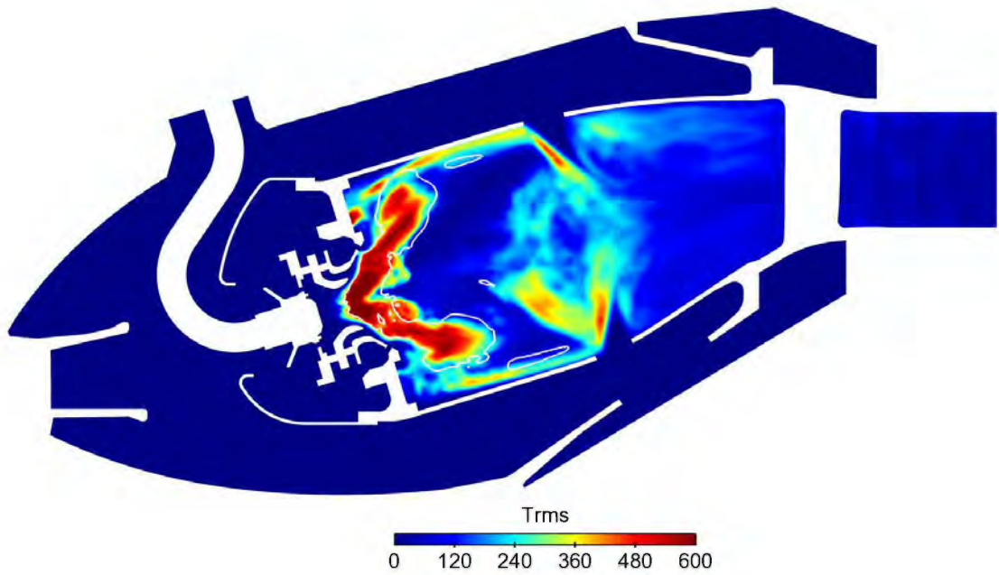
Figure 6.16: Root-mean-squared temperature (K) with white isoline of mean heat release rate ( \text{W}/\text{m}^3 ) at intermediate power
