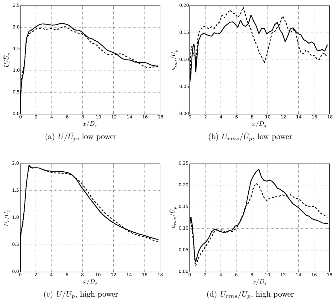
Figure 8.20: Profiles of the axial velocity U/\bar{U}_p and the axial fluctuating velocity U_{rms}/\bar{U}_p on the lip-line of the primary stream (Fig. 8.2). With M_1 grid (—) and M_2 grid (- -).
