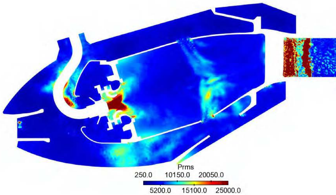
Figure 6.14: Root-mean-squared pressure (Pa) at high power
