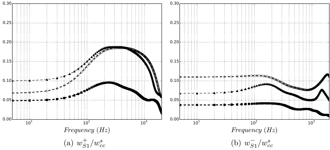
Figure 6.40: Analytical entropy-to-acoustic transfer functions (Eq. 2.75) at position S1 in Fig. 5.4, for low power ( \blacksquare ), intermediate power ( \blacktriangle ) and high power conditions ( \circ ).
