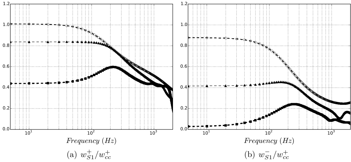
Figure 6.32: Analytical acoustic-to-acoustic transfer functions (Eq. 2.75) at position S1 in Fig. 5.4, for low power (■), intermediate power (▲) and high power conditions (○).
