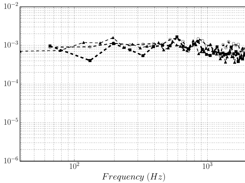
Figure 6.30: Power spectral density of vorticity wave amplitude w^v within the flame tube (position \mathbf{P} in Fig. 6.24) for low power ( \blacksquare ), intermediate power ( \blacktriangle ) and high power conditions ( \circ ).
