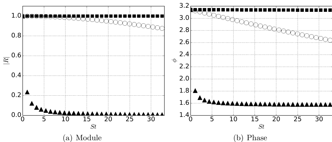
Figure A.2: Theoretical coefficient reflection modulus a) and phase b), in function of the Strouhal number for several relaxation coefficient values, K_{sec} = 1000 (▲), K_{sec} = 225000 (○) and K_{sec} = 1550000 (■).
