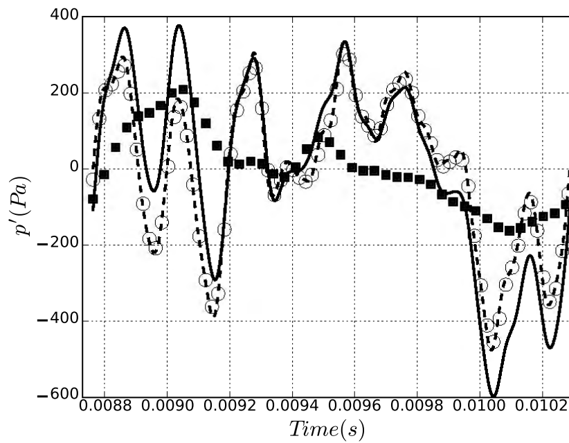
Figure 4.9: Pressure fluctuations (—), A^+ (○) and A^- (■) at the outlet compared with the incoming forced wave originated from combustion process (--)
