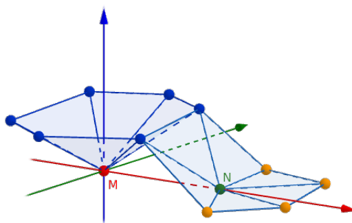
Figure 6.16: Constraint on the link
