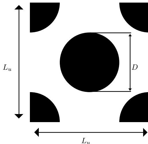
Figure 3.5: Top view of the 3D Representative Elementary Volume (REV) used in [68] to evaluate \mathbf{D}_{\beta\sigma} the fluid-solid force within the porous medium.
