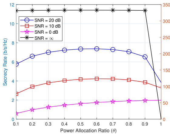
(a) Zero-Forcing.
