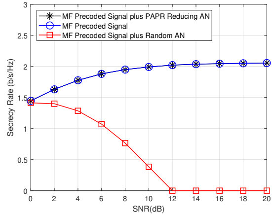
(b) Matched Filter à \theta = 0.6 .
