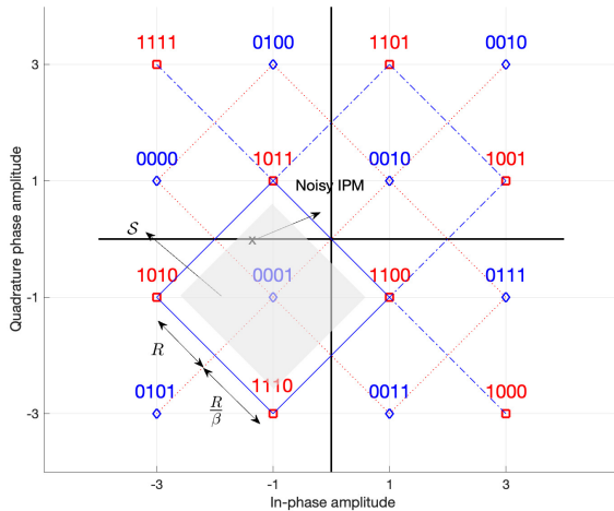
(a) Noisy IPM: one-bit partitioning \Lambda_0 \rightarrow \diamond and \Lambda_1 \rightarrow \square .
