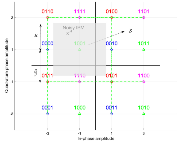
(b) Noisy IPM: two-bit partitioning \Lambda_{00} \rightarrow \diamond , \Lambda_{01} \rightarrow \square , \Lambda_{10} \rightarrow \triangle and \Lambda_{11} \rightarrow \circ .
