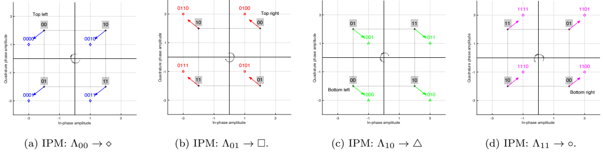
Figure 5.4: Binary mapping with respect to \mathcal{C}_2(k) in (5.6)
