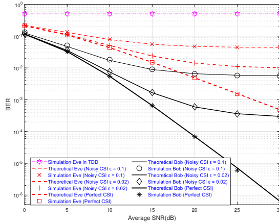
Figure 4.4: BER performance with imperfect CSI.
