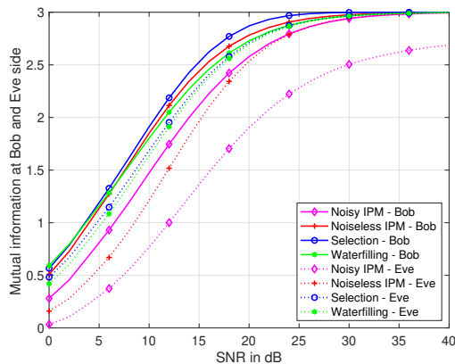
(c) 16-QAM(3bpcu)
