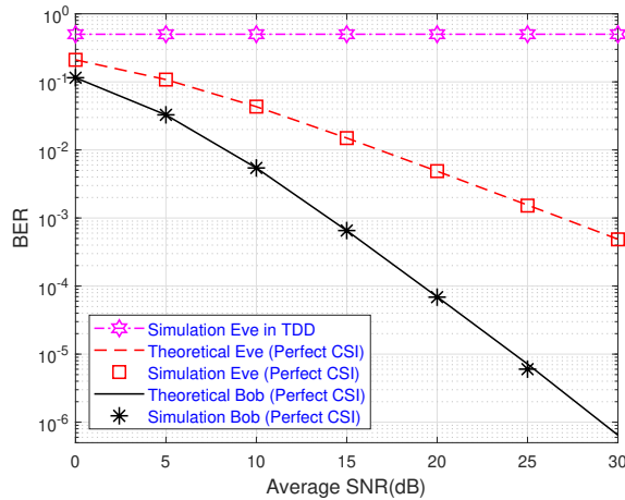
Figure 4.2: BER performance with perfect CSI.
