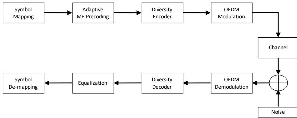
Figure 4.1: OFDM system model employing diversity and adaptive PLS technique.
