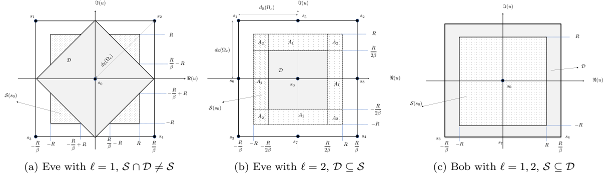
Figure 5.6: Error detection zones: the detection \mathcal{D} zone is in gray and the uniform noise domain space \mathcal{S} is filled with a dot pattern
