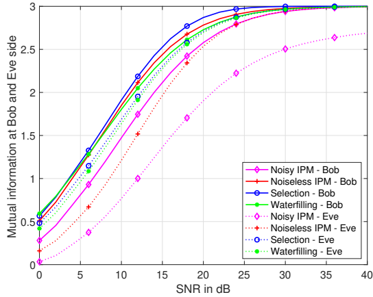
(a) 16-QAM(3bpcu)
