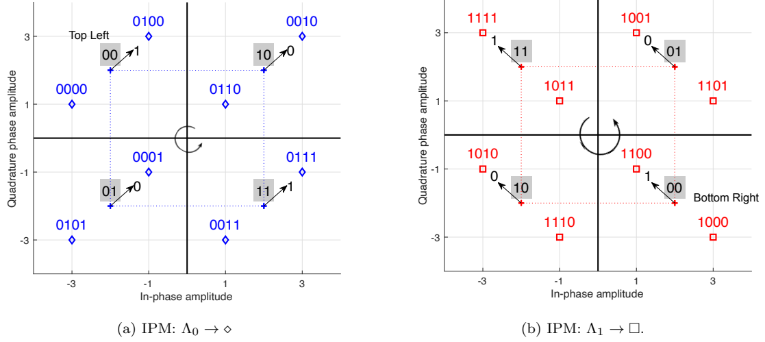
Figure 5.3: Binary mapping with respect to \mathcal{C}_1(k) in (5.5)
