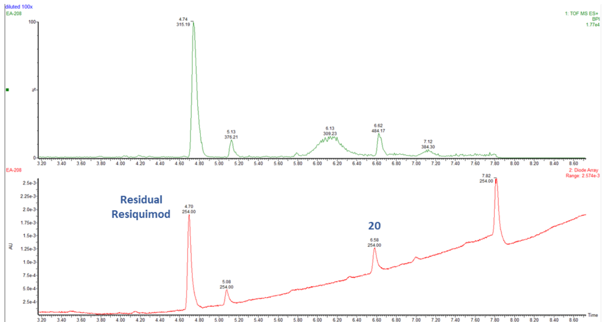
Figure 2S: LC-MS analysis of 20 showing degradation of the compound by Resiquimod decoupling. Mass on the top part, UV on the bottom part.
