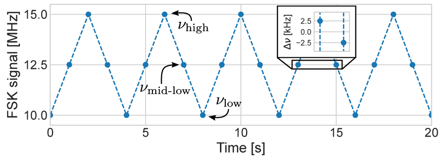
FIGURE 5.10: Frequency-shift keying (FSK) signal measured by the frequency counter in \Lambda -mode, over the duration of 20 s. Small insert shows the frequency difference between the two central values around 12.5 \text{ MHz} \pm 2.5 \text{ kHz} .
