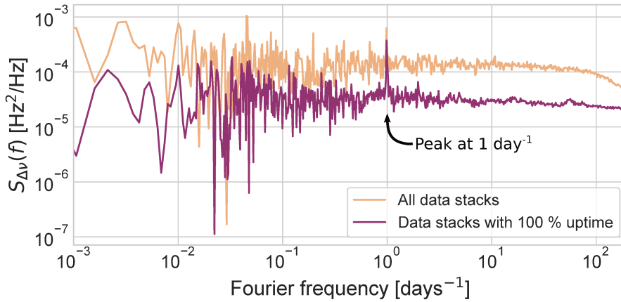
FIGURE 4.13: Frequency PSD when using all stacks of data (orange), and when only using stacks of data with 100 % uptime. Missing data has been replaced with simulated noise for both spectra.
